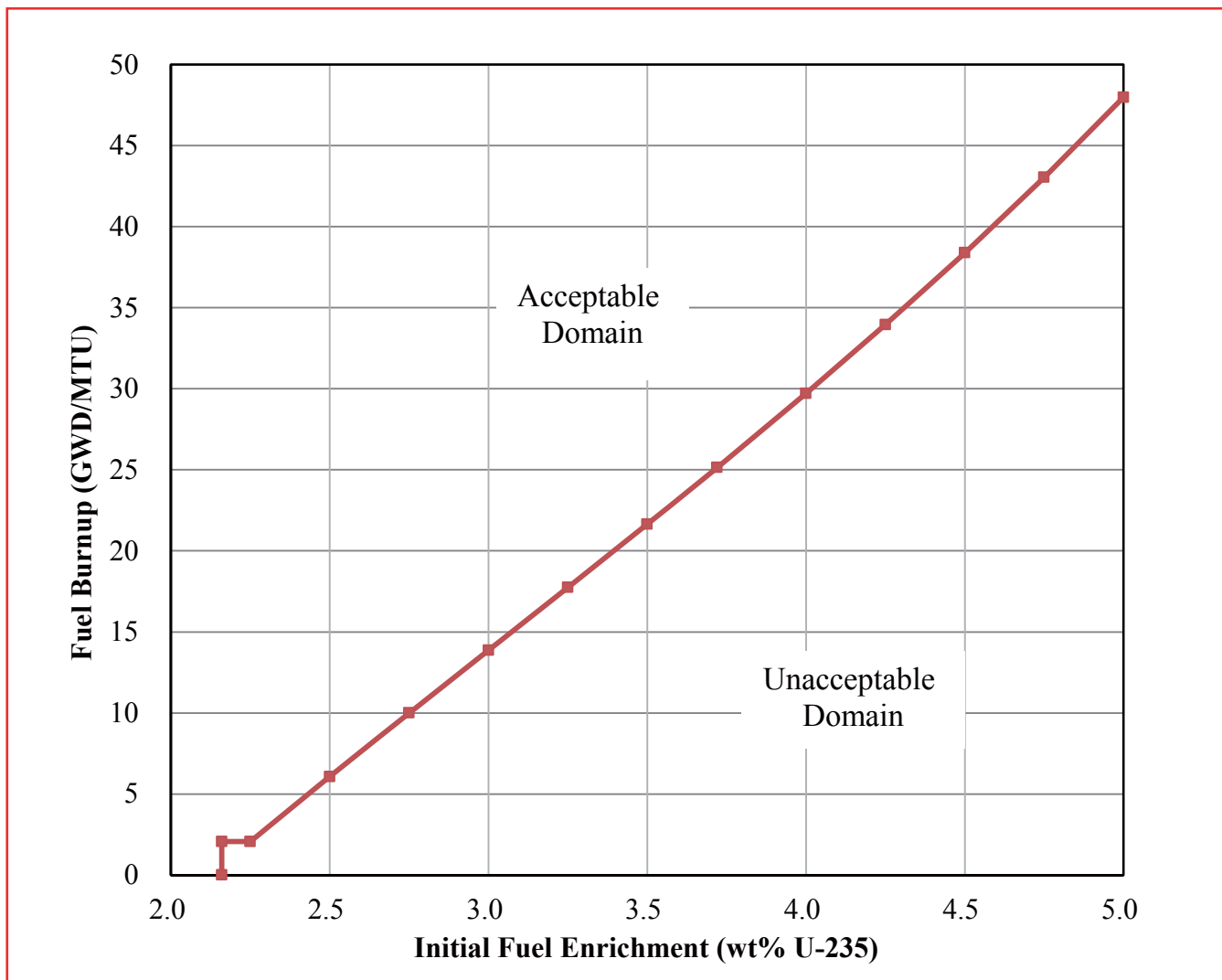
Figure 3.7.16-1 (page 1 of 1) Discharge Burnup vs. Initial Enrichment for Region II Racks
