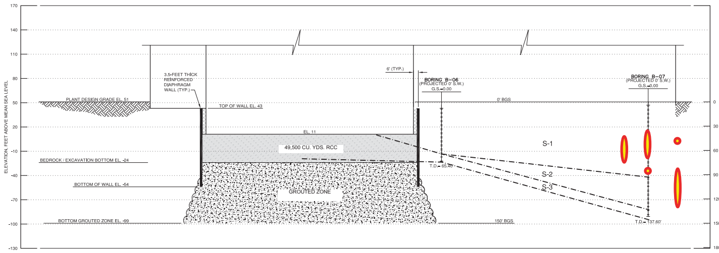
SECTION A
