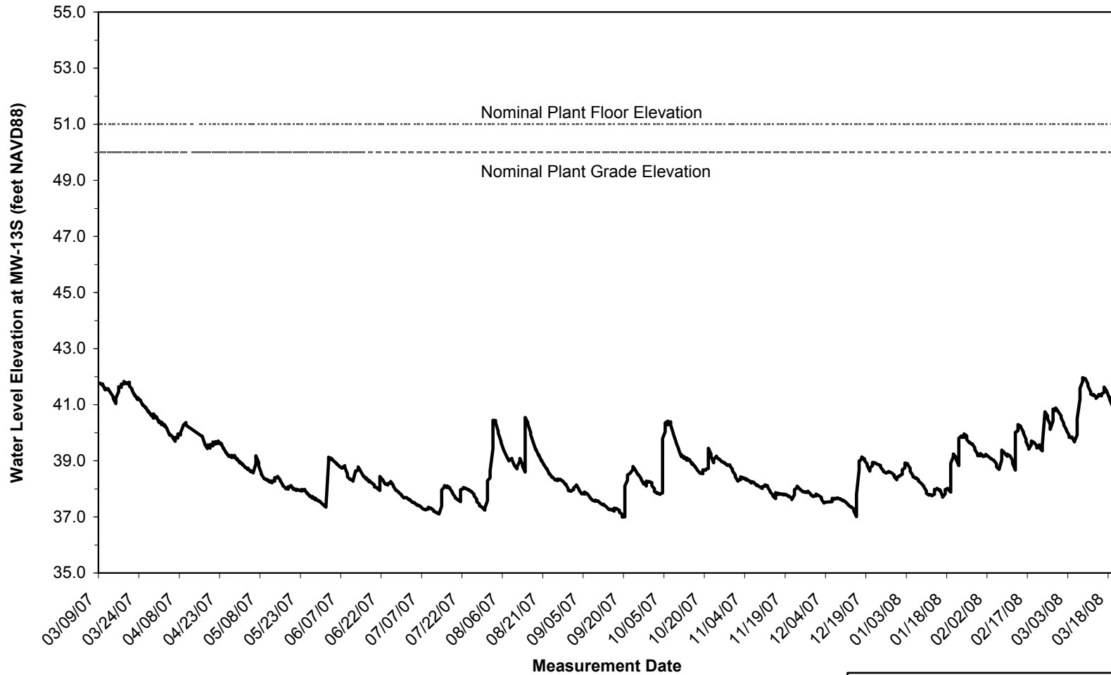
Duke Energy Florida Levy Nuclear Plant Units 1 and 2 Part 2, Final Safety Analysis Report Surficial Aquifer Groundwater Elevation at LNP 2 FIGURE 2.4.12-224 Rev 6
