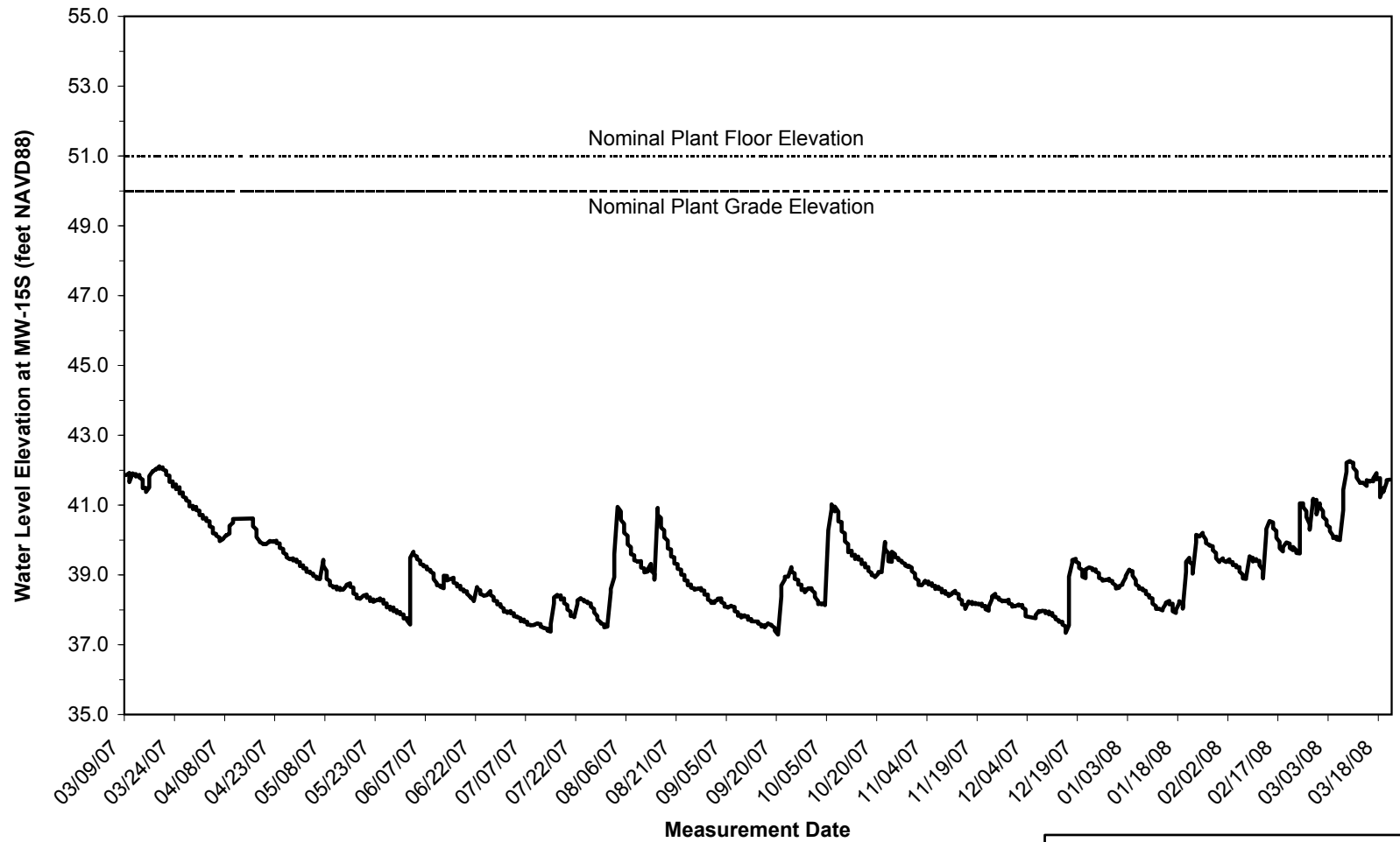
Duke Energy Florida Levy Nuclear Plant Units 1 and 2 Part 2, Final Safety Analysis Report Surficial Aquifer Groundwater Elevation at LNP 1 FIGURE 2.4.12-223 Rev 6
