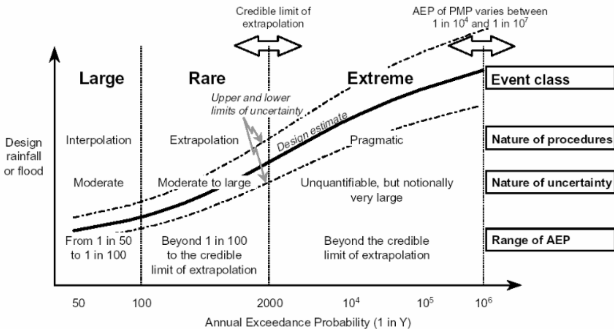
Figure D-1 - Characteristics of Notional Floods (Nathan and Weinmann, 2001)
