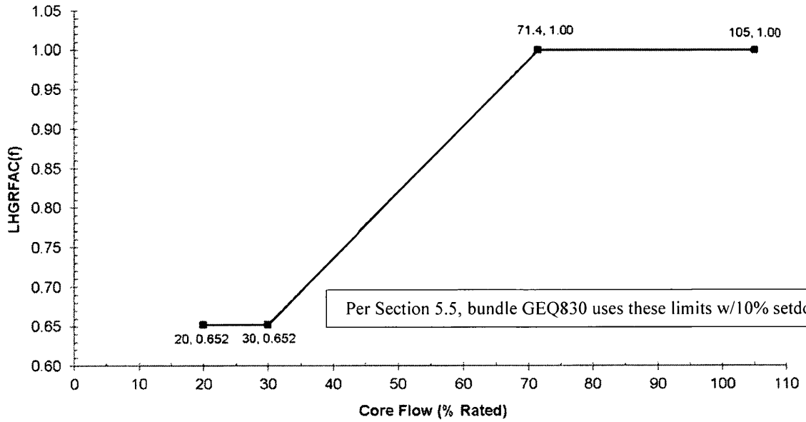
Figure 3-2 Cycle 21 Flow-Dependent LHGR Factor Note: These factors to be applied to the exposure-dependent limits as described in Section 5.3
