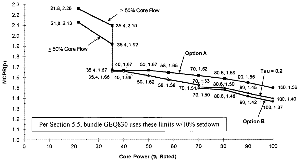
Figure 2-2 Cycle 21 Power-Dependent MCPR Limits BOC to MOC with EOC-RPT Inoperable
