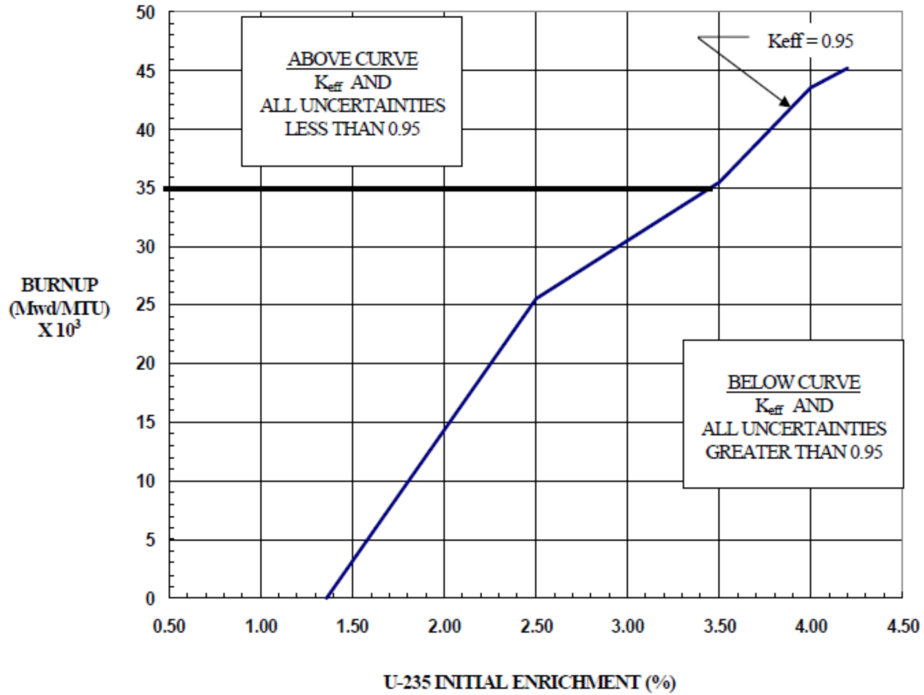
FUEL CRITICALITY ACCEPTABILITY CURVE
