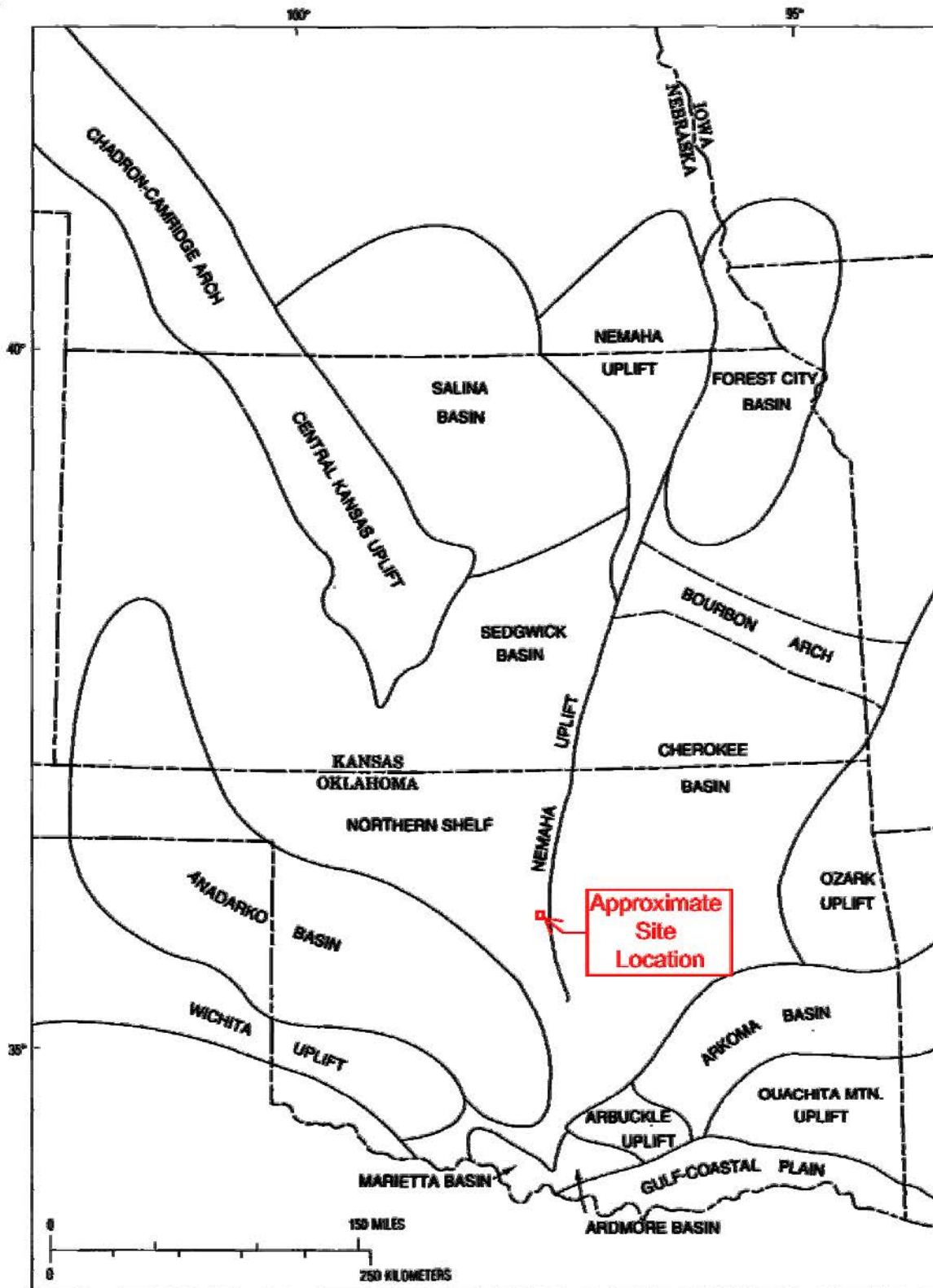
Figure 2-5 LOCATION OF THE NEMAHA UPLIFT DECOMMISSIONING PLAN CIMARRON SITE, OKLAHOMA
