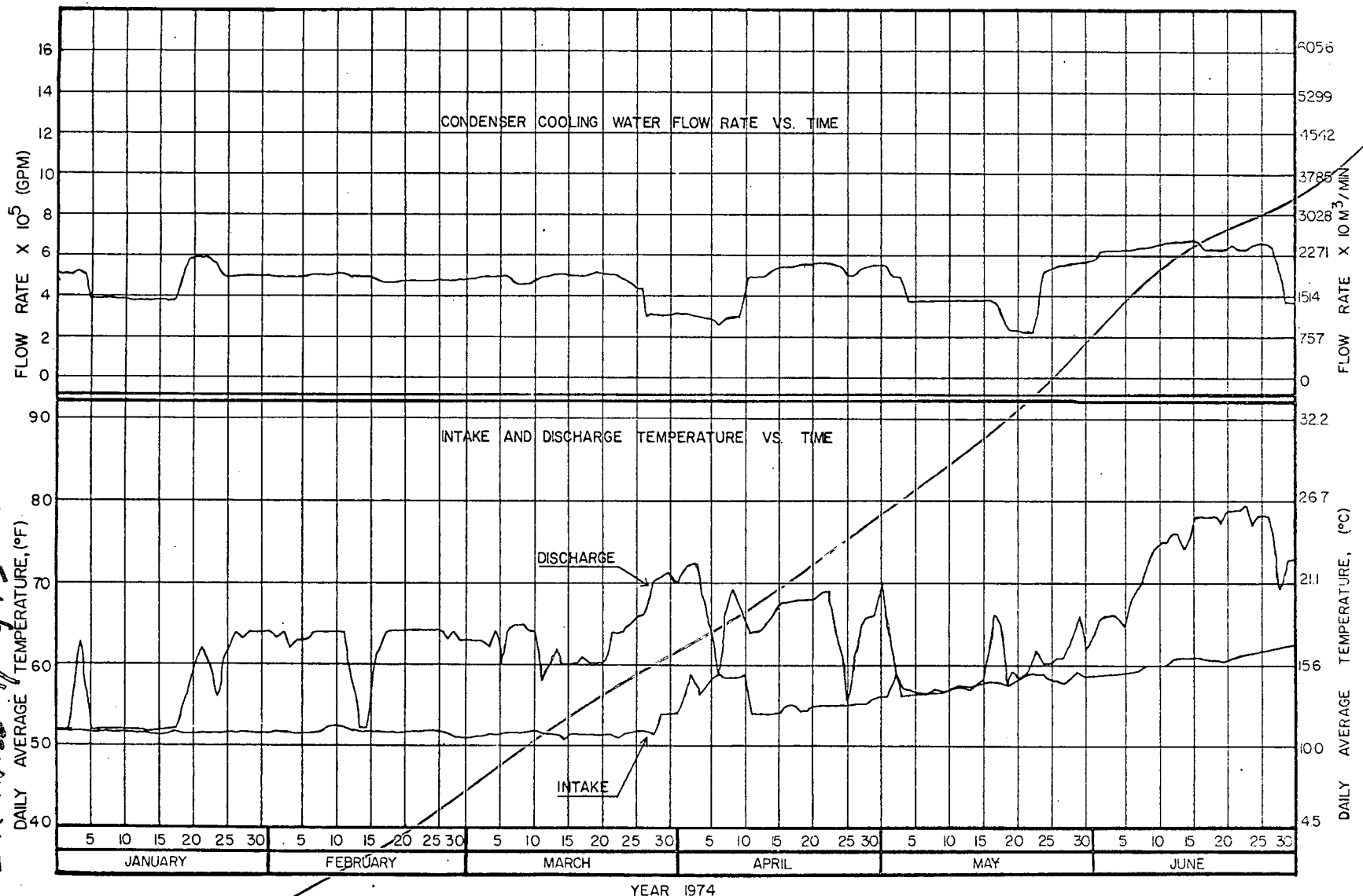
FIGURE 1.1-1 OCONEE NUCLEAR STATION DAILY AVERAGE TEMPERATURES AND CONDENSER FLOW RATES ONS 6/74
