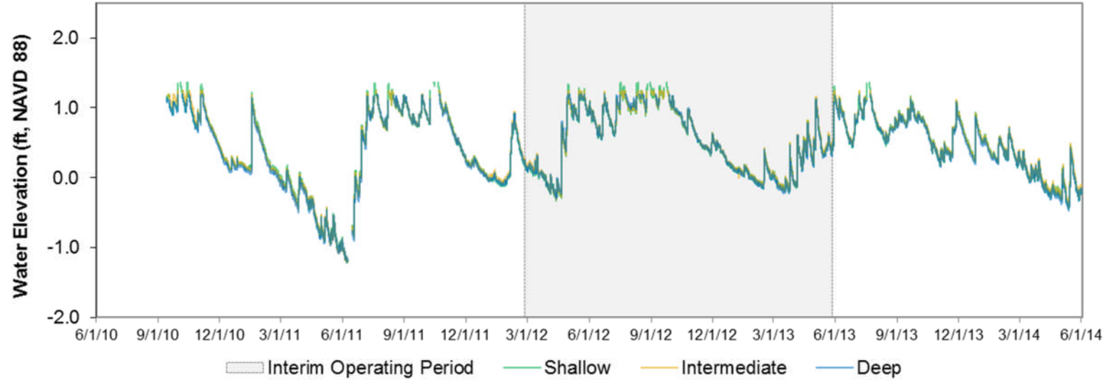
Figure 2.3-7. TPGW-7 Water Elevations.
