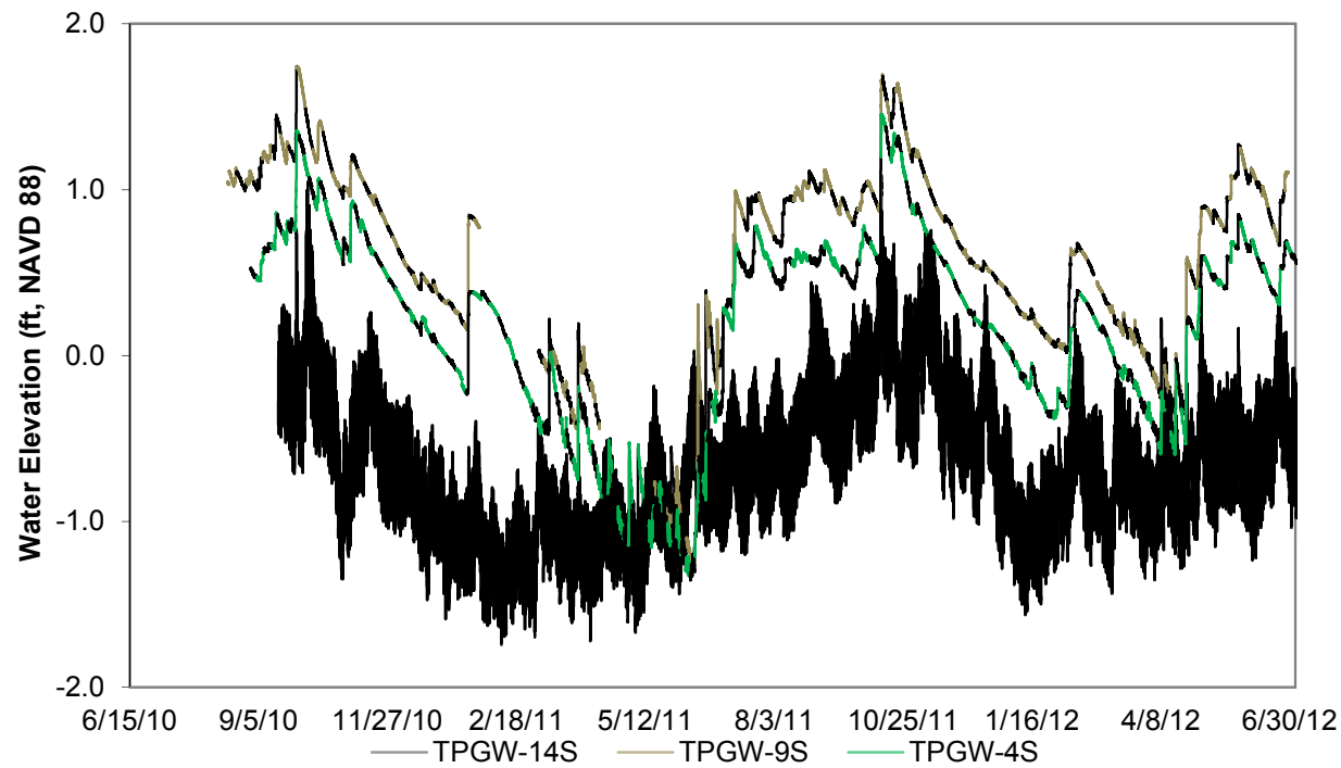
Figure 2.3-16. Comparison of Time Series Groundwater Water Elevations across the Landscape at TPGW-14, TPGW-9 and TPGW-4.
