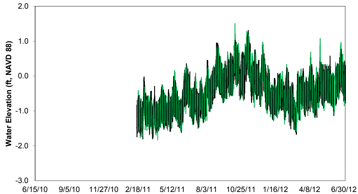
Figure 2.3-24. TPBBSW-14 Water Elevations.
