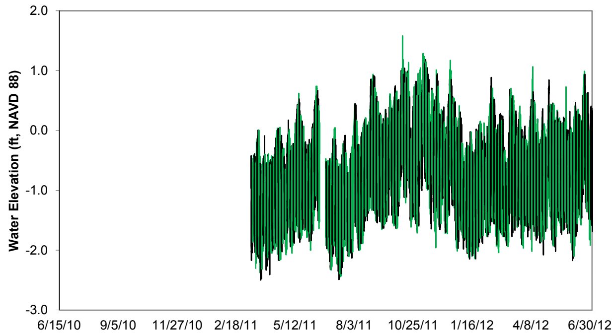
Figure 2.3-22. TPBBSW-10 Water Elevations.
