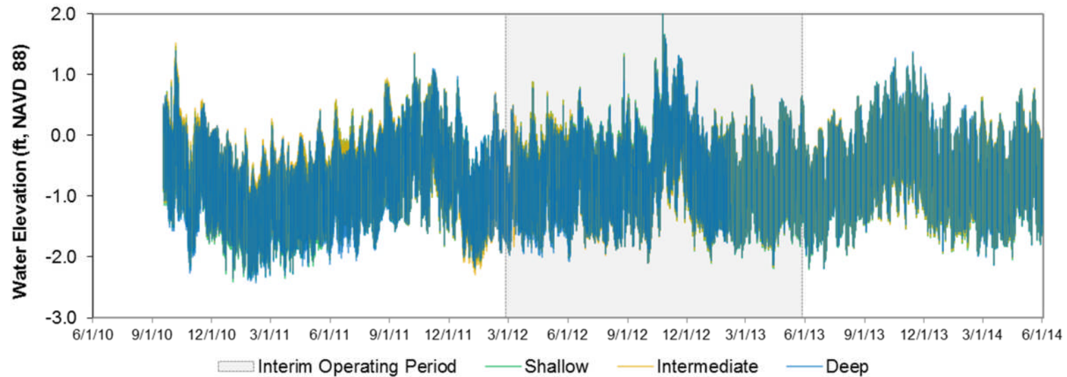
Figure 2.3-11. TPGW-11 Water Elevations.
