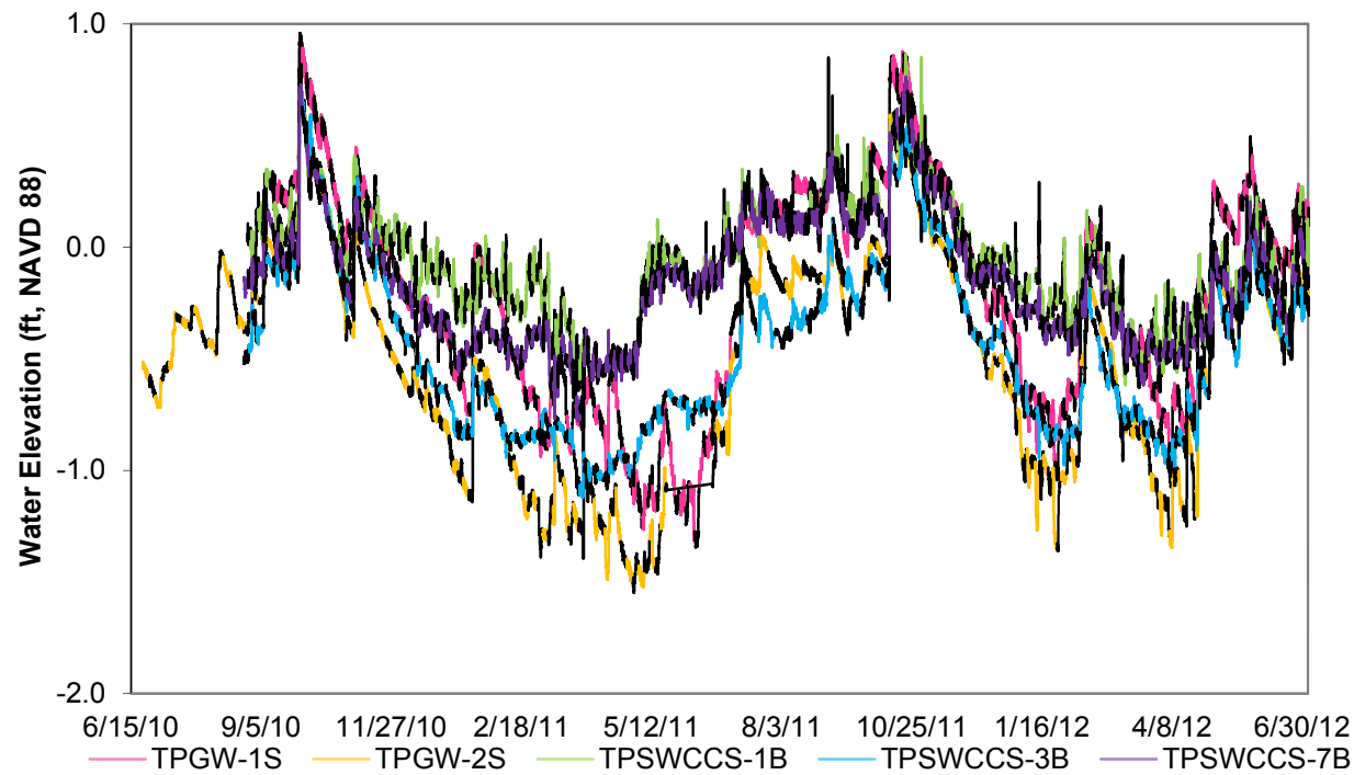
Figure 2.3-20. Comparison of Time Series Groundwater Water Elevations at TPGW-1 and TPGW-2, and CCS Surface Water Stations TPSWCCS-1, TPSWCCS-3, and TPSWCCS-7.
