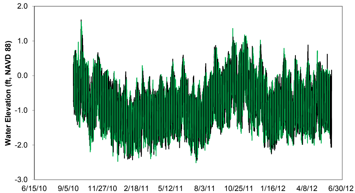
Figure 2.3-23. TPBBSW-3 Water Elevations.
