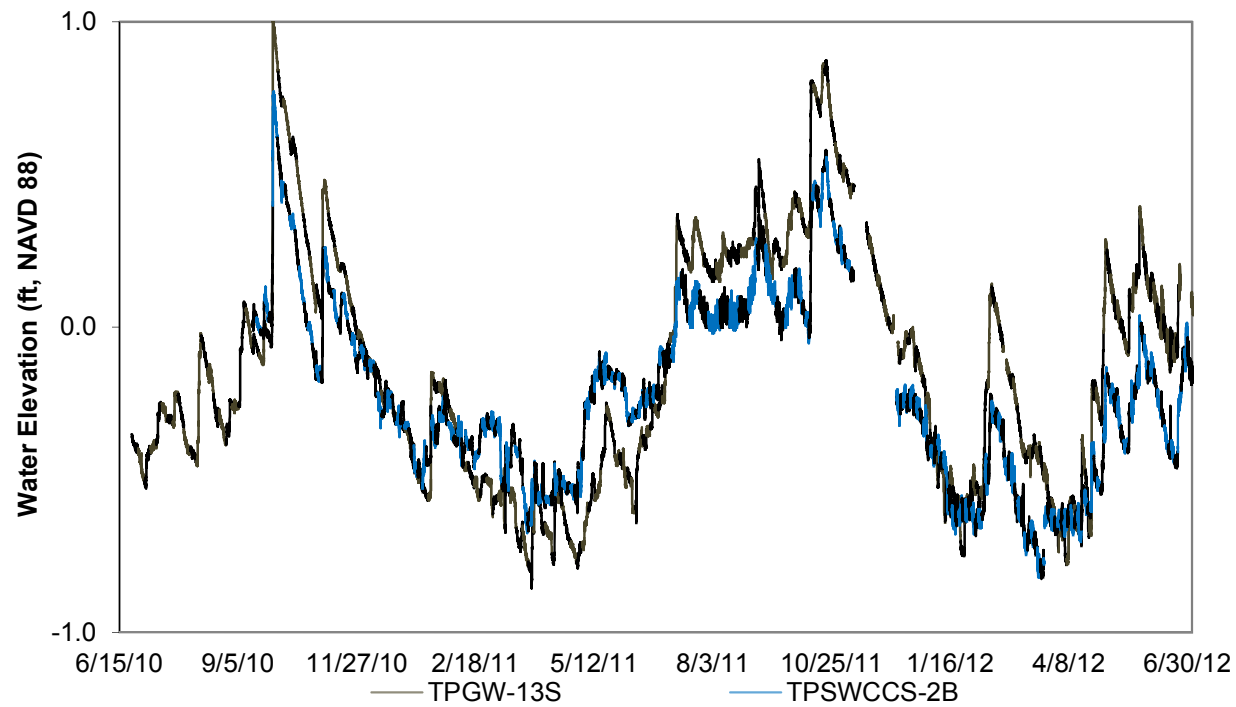
Figure 2.3-19. Comparison of Time Series Groundwater Water Elevations at TPGW-13 and TPSWCCS-2.
