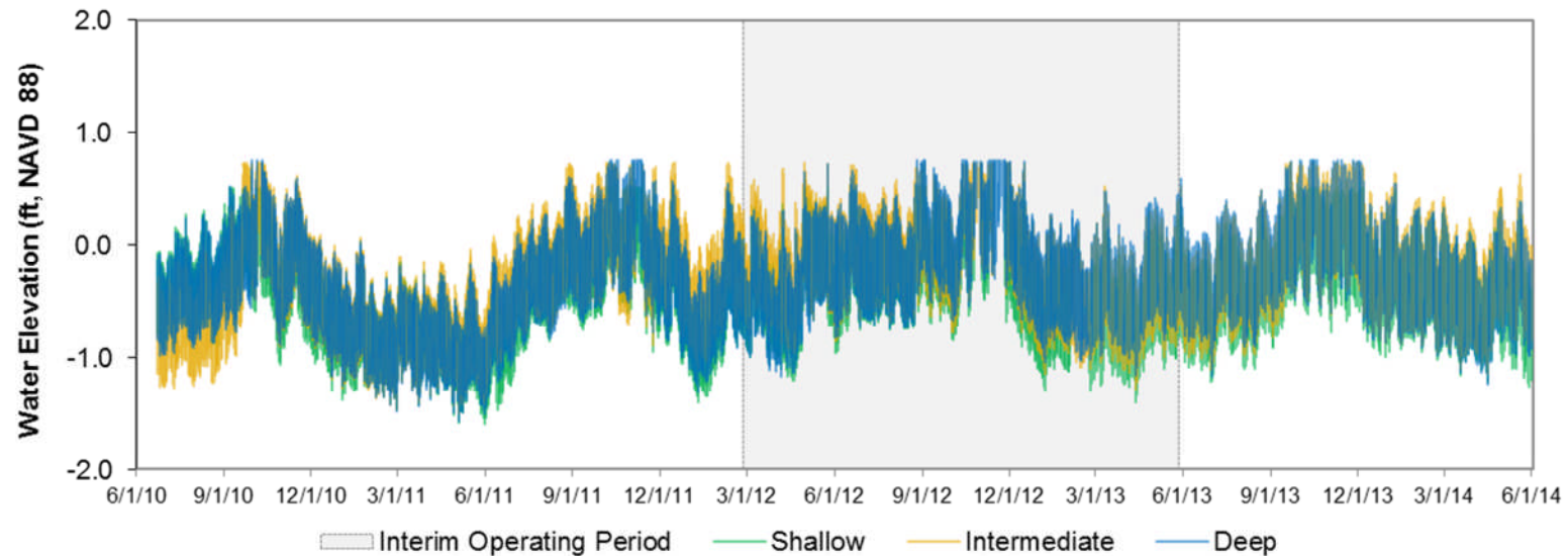
Figure 2.3-12. TPGW-12 Water Elevations.
