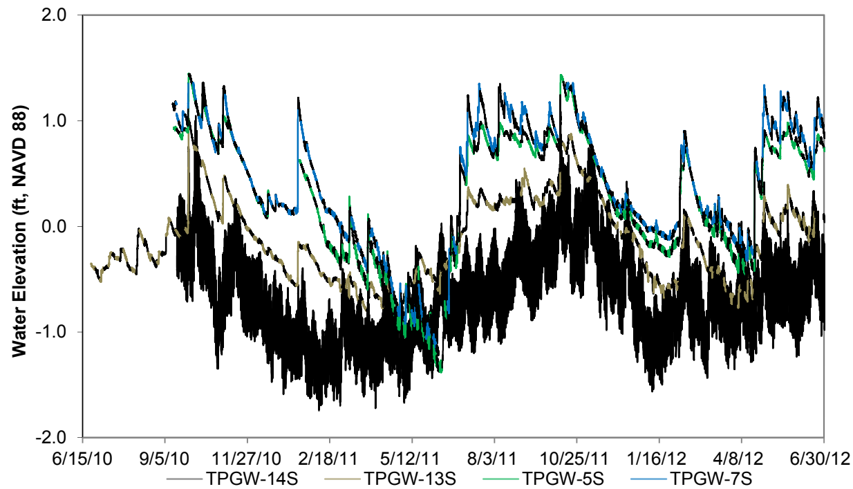
Figure 2.3-15. Comparison of Time Series Groundwater Water Elevations across the Landscape at TPGW-14, TPGW-13, TPGW-5 and TPGW-7.
