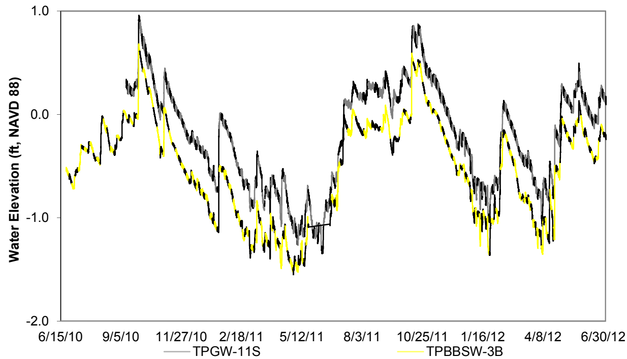
Figure 2.3-21. Comparison of Daily Average Time Series Groundwater Water Elevations in Biscayne Bay Well TPGW-11 and Biscayne Bay Surface Water Station TPBBSW-3.
