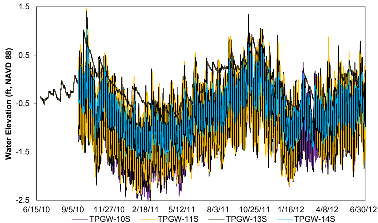
Figure 2.3-18. Comparison of Time Series Groundwater Water Elevations across the Landscape at TPGW-10, TPGW-11, TPGW-13, and TPGW-14.
