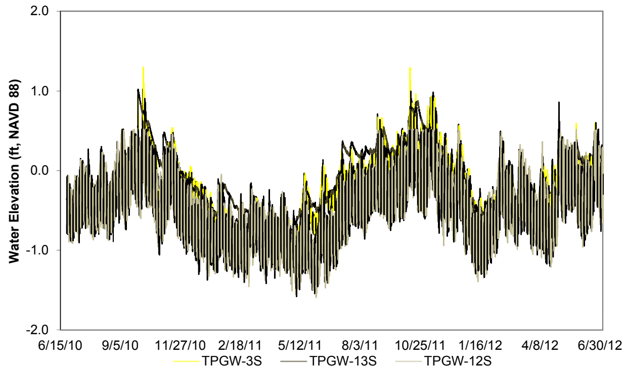
Figure 2.3-17. Comparison of Time Series Groundwater Water Elevations across the Landscape at TPGW-3, TPGW-13, and TPGW-12.
