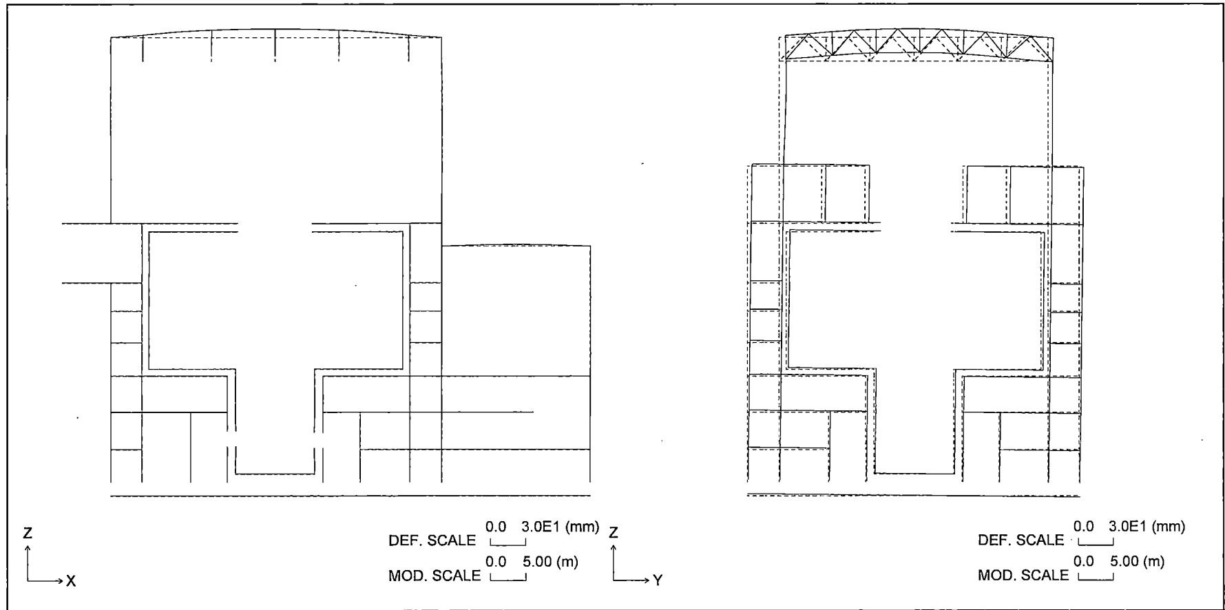
Figure 6.2.4-18 Section Deformation for Wind Load (West Wind)
