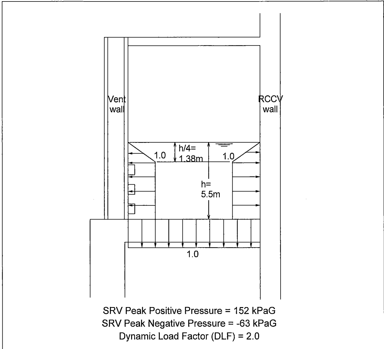
Figure 5.2.3-1 Safety Relief Valve (SRV) Pressure Loads
