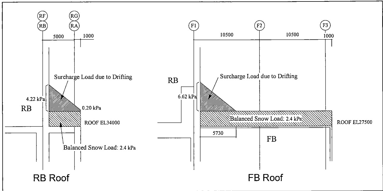
Figure 5.1.2-1 Snow Load
