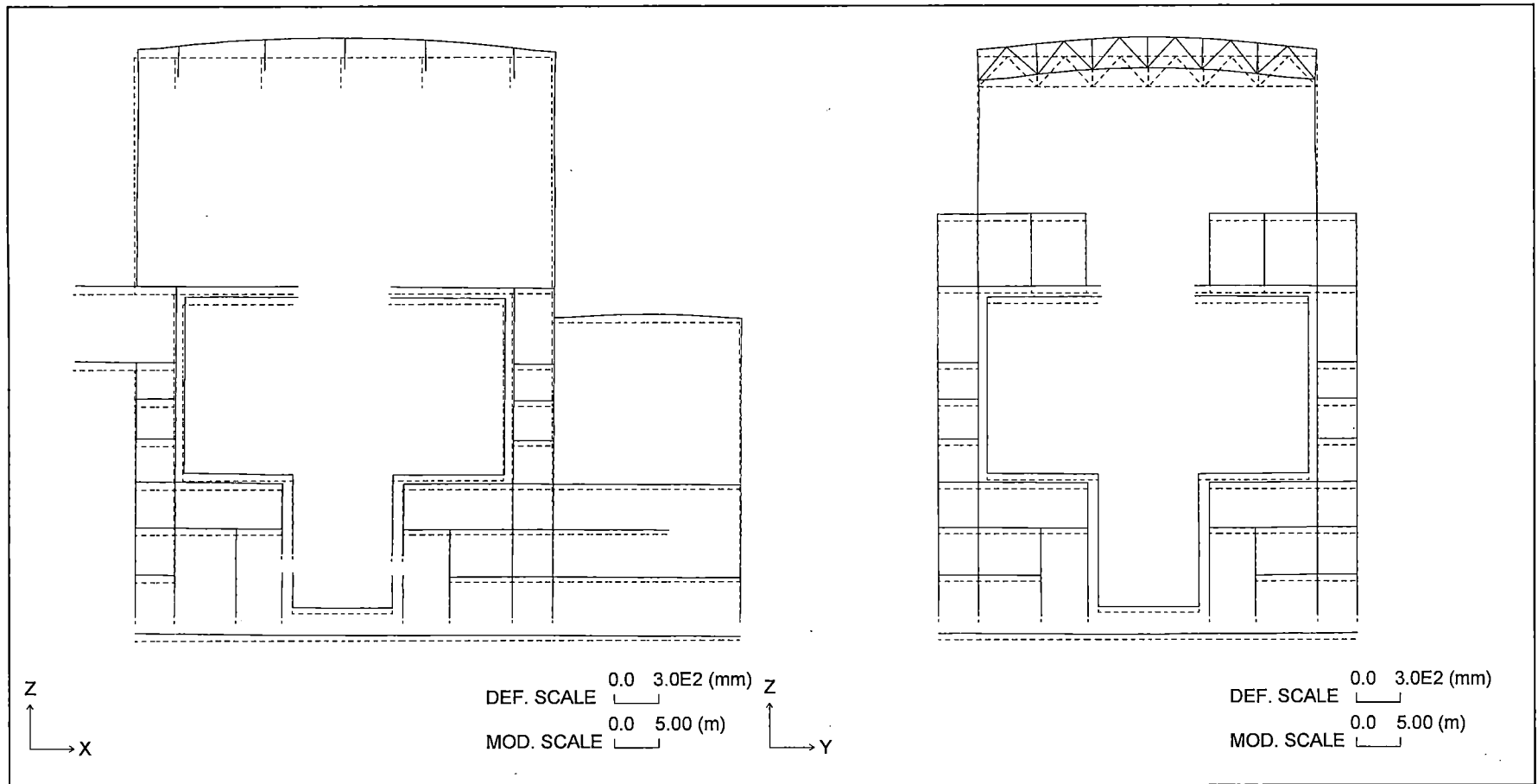
Figure 6.2.4-12 Section Deformation for Seismic Load (Vertical: Upward)
