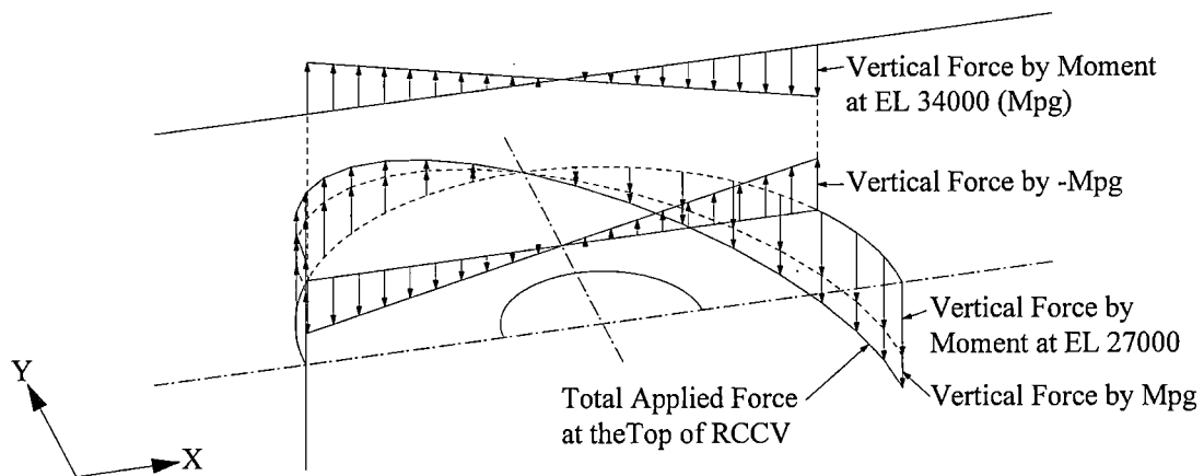
X-direction Moment
