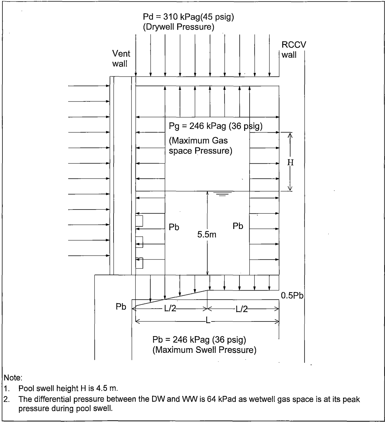
Figure 5.2.3-5 Pool Swell (PS) Pressure Loads
