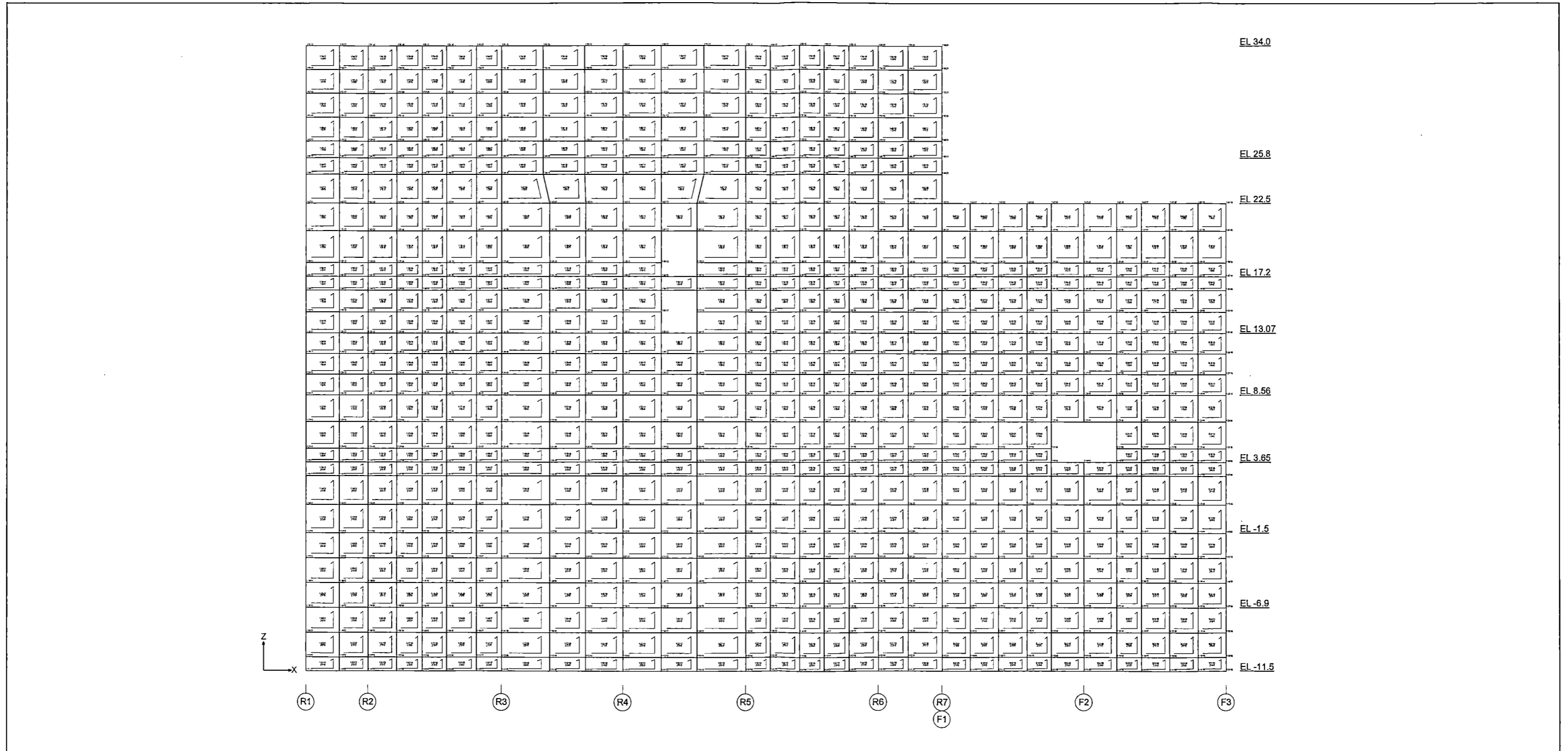
Figure 6.2.2-24 FE Model of the External Wall (RG/FF Column Line)
