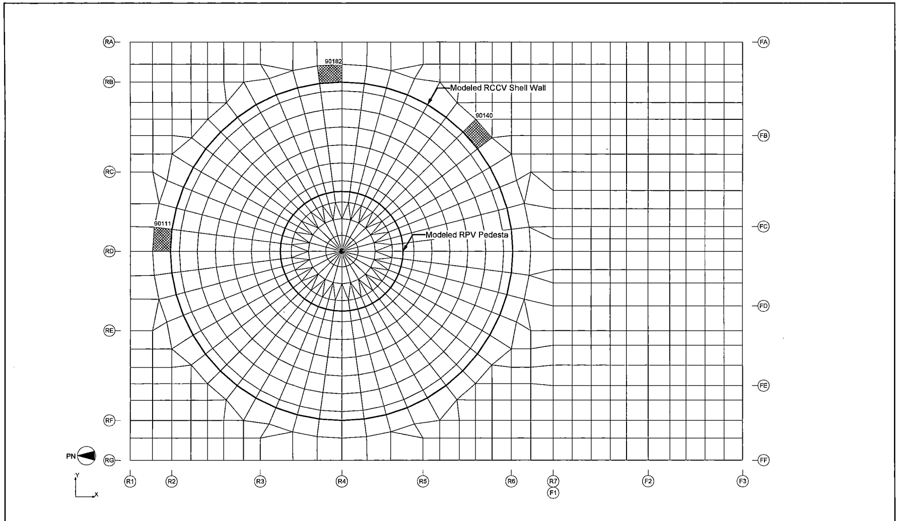
Figure 6.2.4-28 Elements Selected for Tabulation (Basemat)
