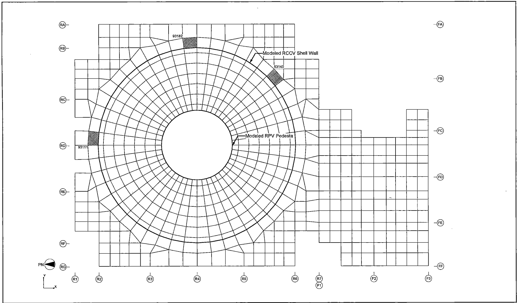
Figure 6.2.4-29 Elements Selected for Tabulation (Slab at EL 4,650)
