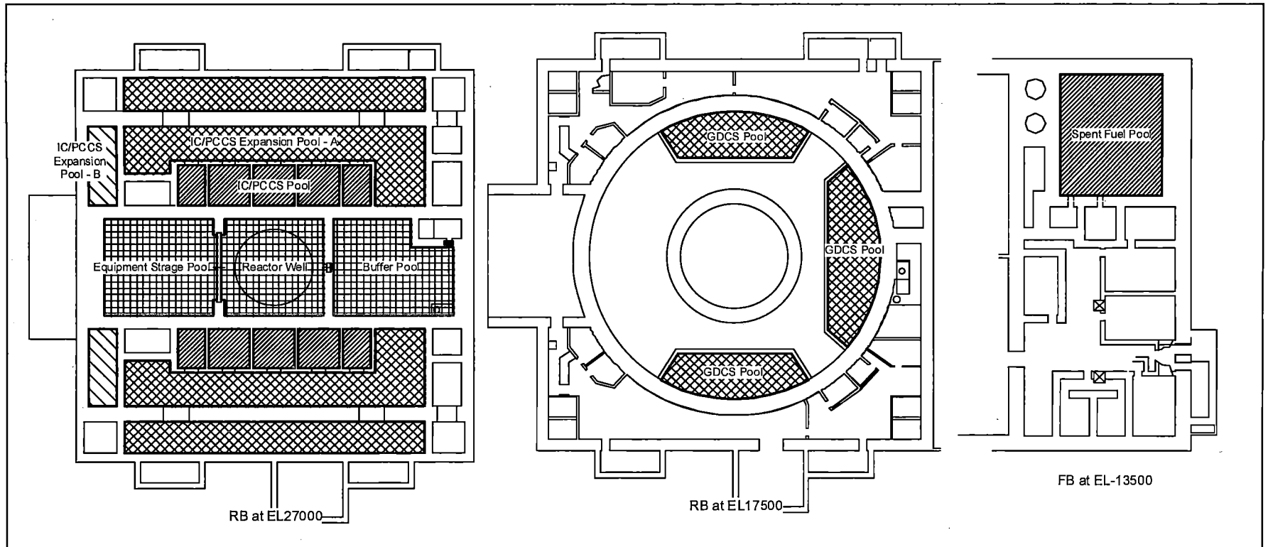
Figure 5.3.3-2 Position of Each Pool
