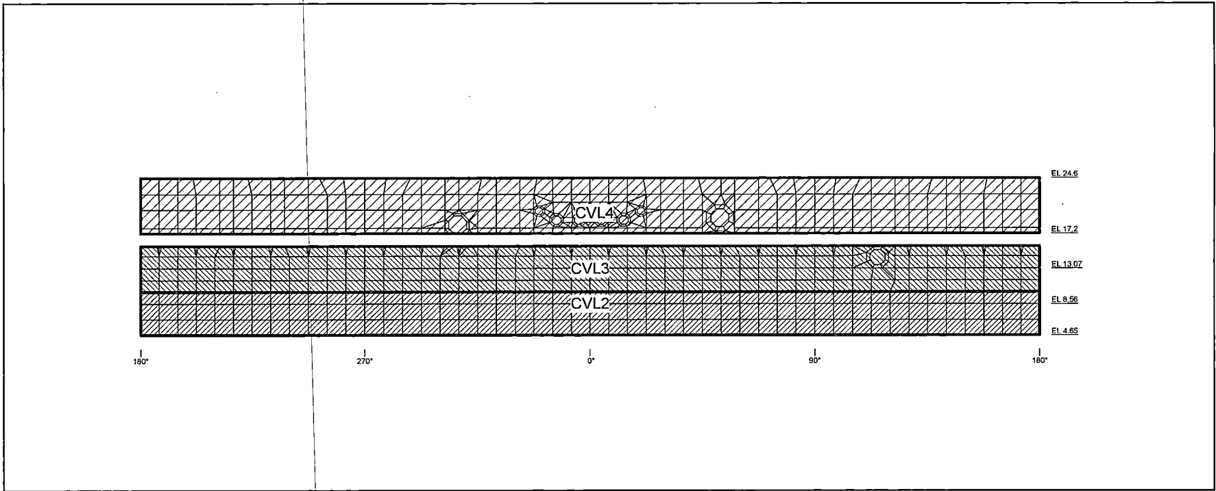
Figure 6.2.3.4-29 Application of Thermal Load on the RCCV Liner (Condition 2)
