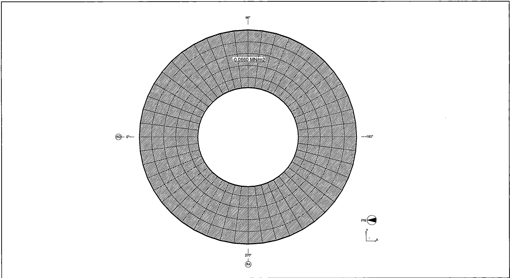
Figure 6.2.3.5-8 Application of Hydrodynamic Load on the Suppression Pool Slab Liner (CH Negative)
