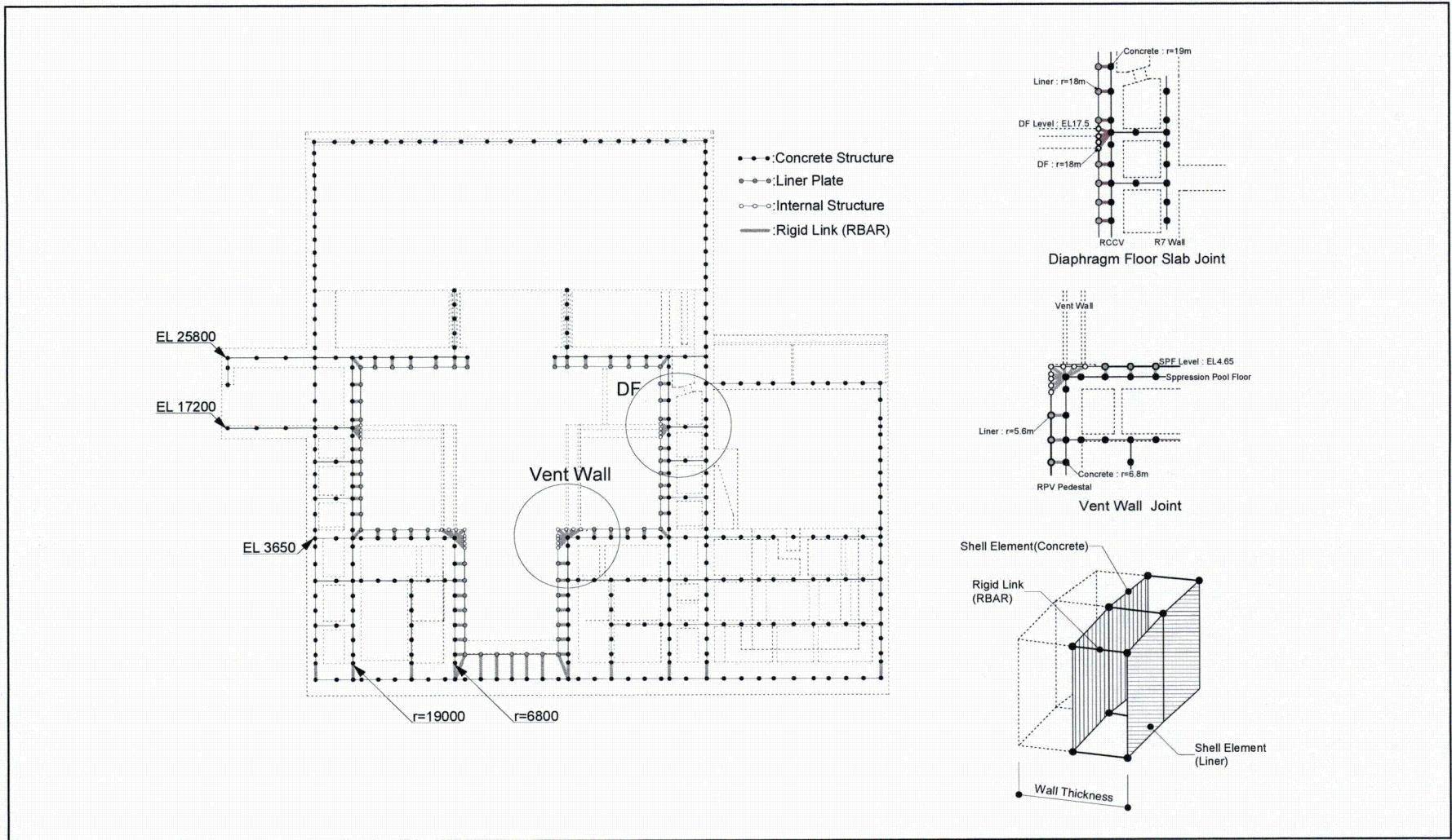
Figure 6.2.2-16 Rigid Bar Elements between Concrete and Liner
