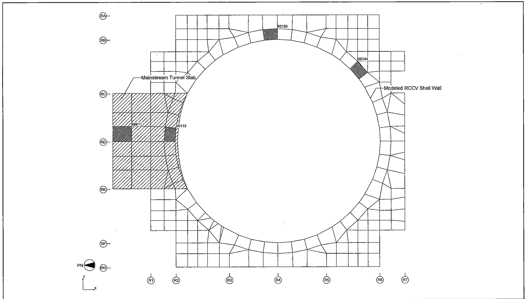
Figure 6.2.4-30 Elements Selected for Tabulation (Slab at EL 17,500)
