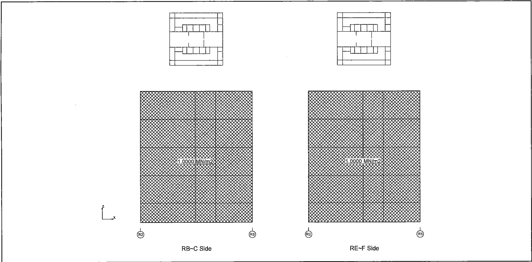
Figure 6.2.3.3-19 Containment Pressure Load (IC/PCCS Pool: Wall-1)
