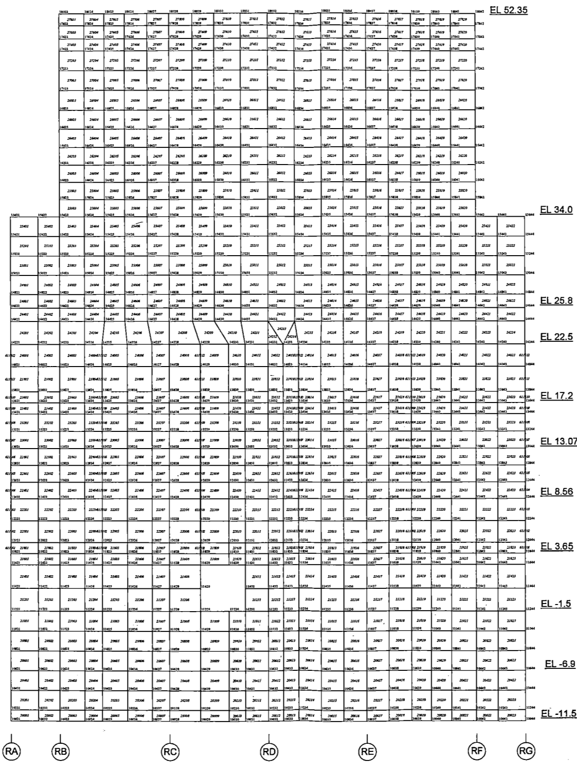
Figure 6.2-26 FE Model of the External Wall (R7/F1 Column Line)
