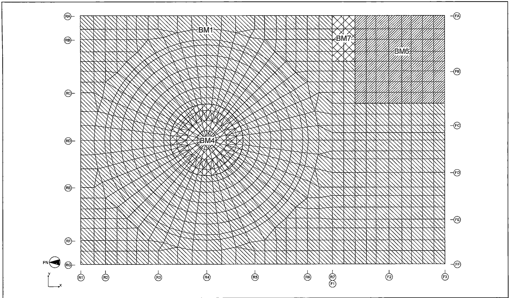
Figure 6.2.3.4-13 Application of Thermal Load on the Basemat (during LOCA Flooding)
