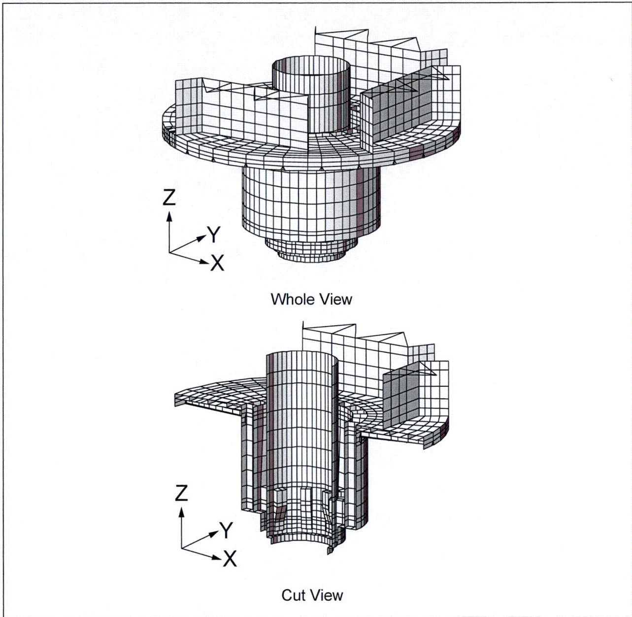
Figure 6.2.2-4 FE Model of RCCV Internal Structures
