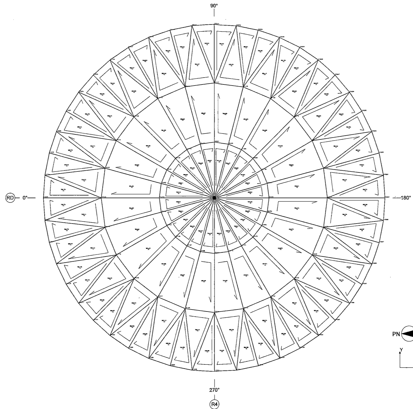
Figure 6.2.2-13 FE Model of the Basemat Liner (EL -10,400)
