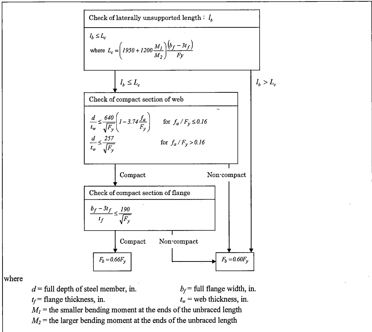
Figure 6.4.2-3 Allowable Bending Stress of Box Members
