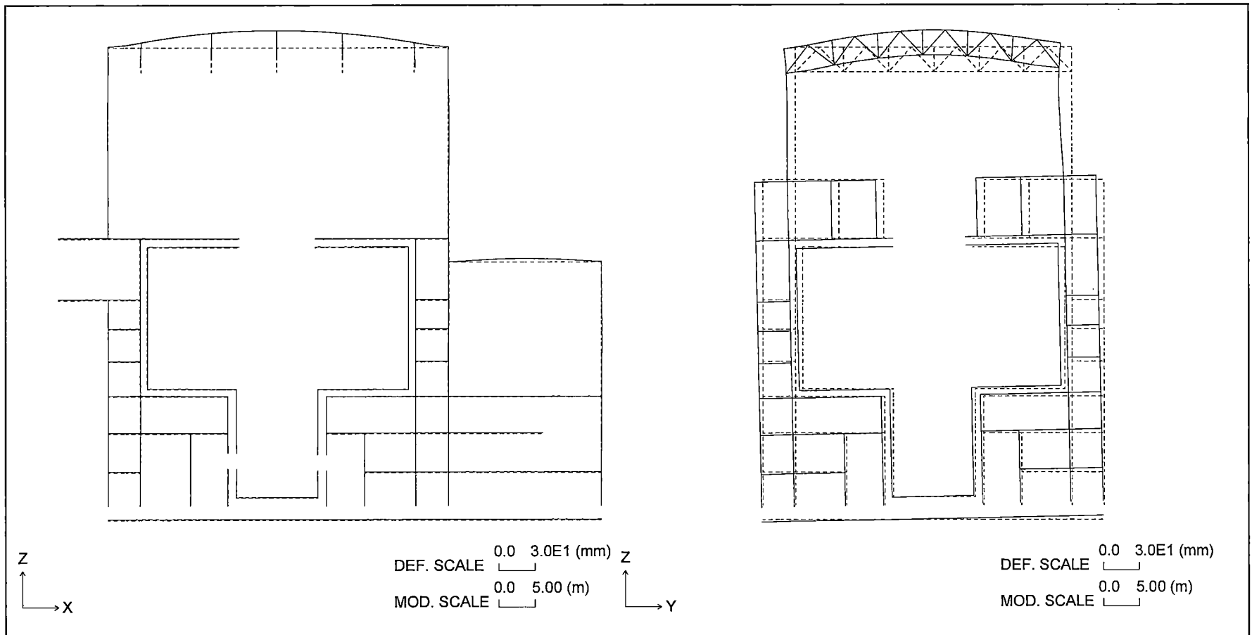
Figure 6.2.4-21 Section Deformation for Tornado Load (East Wind)
