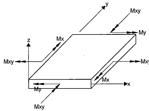
Moments
