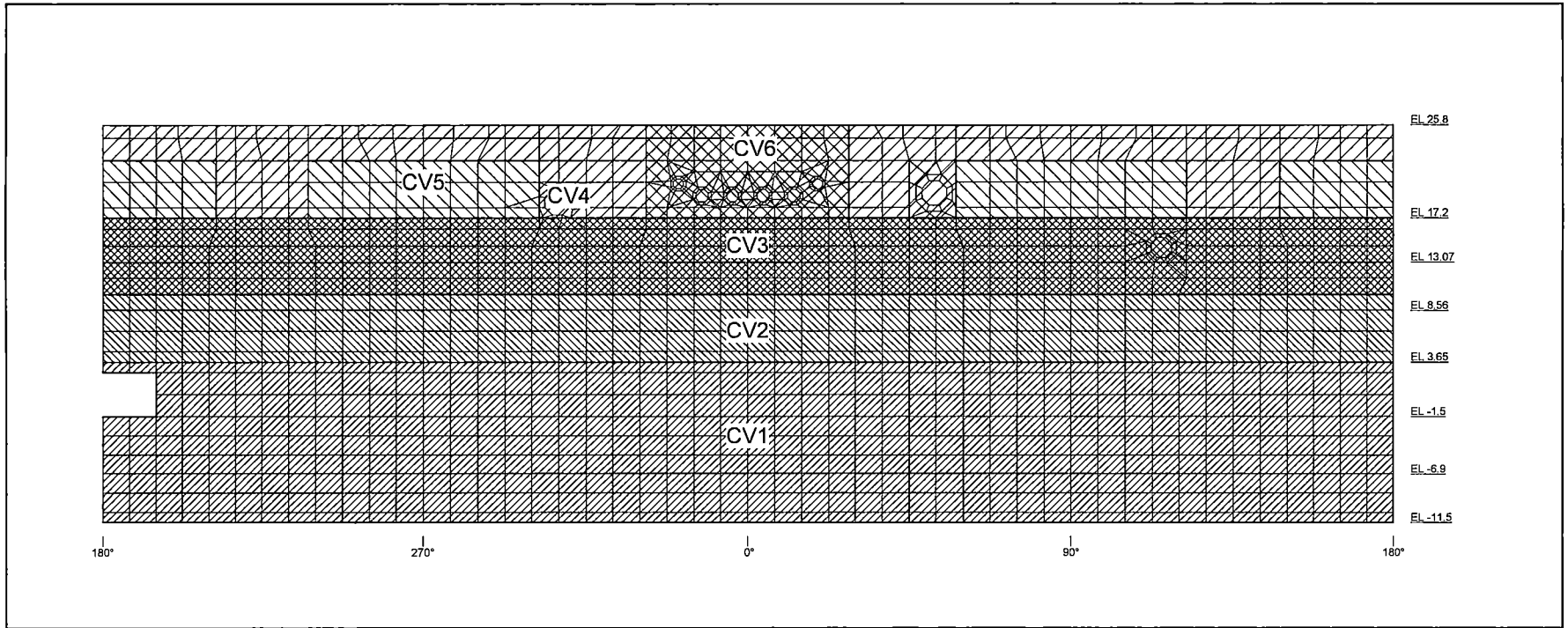
Figure 6.2.3.4-2 Application of Thermal Load on the RCCV Wall (LOCA Condition 1)
