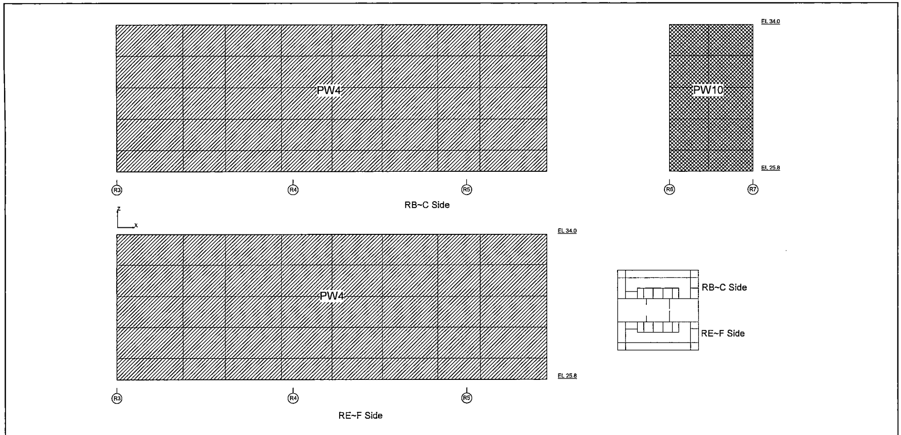
Figure 6.2.3.4-23 Application of Thermal Load on the IC/PCCS Pool Wall-1 (1)
