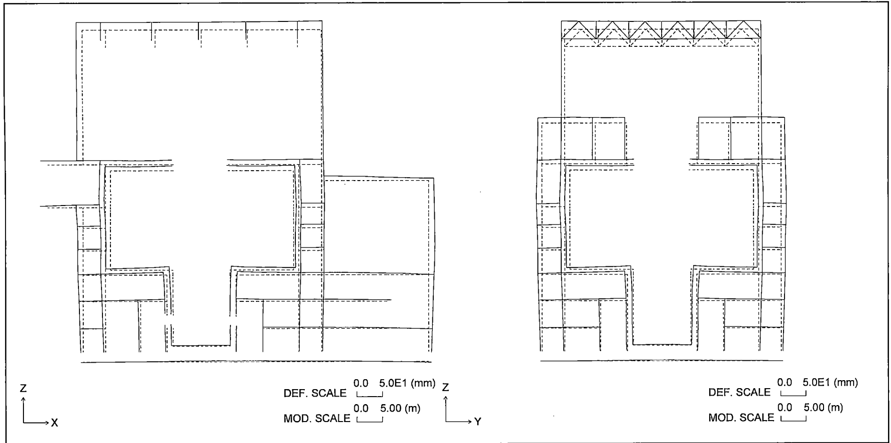
Figure 6.2.4-8 Section Deformation for Thermal Load (LOCA After 6 min.: Summer)
