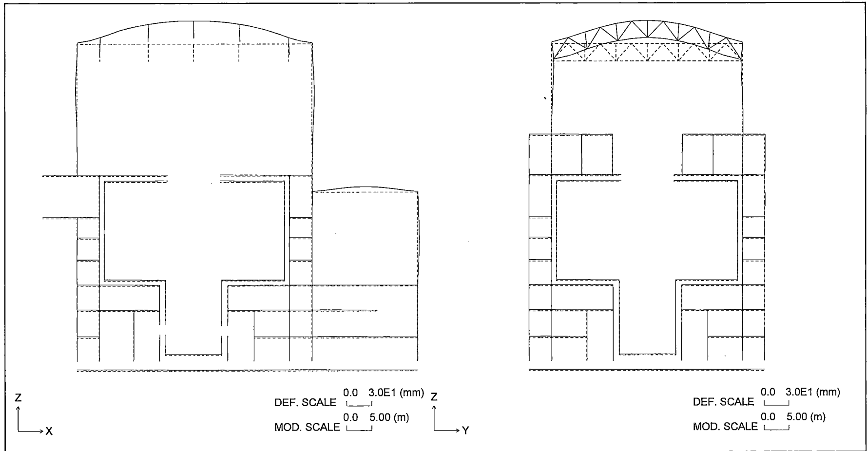
Figure 6.2.4-23 Section Deformation for Tornado Load (Differential Pressure)
