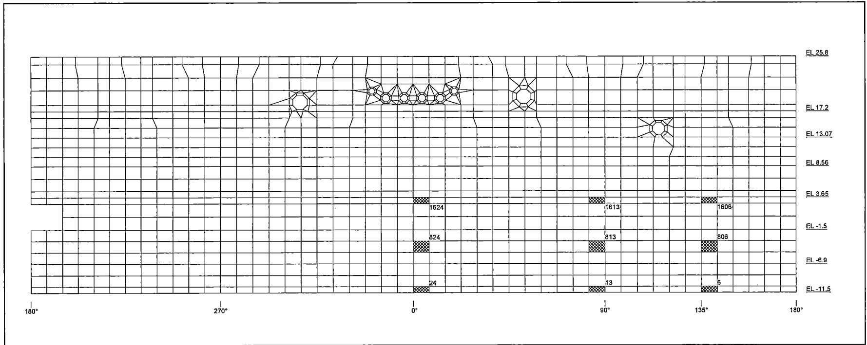
Figure 6.2.4-24 Elements Selected for Tabulation (Wall below RCCV)
