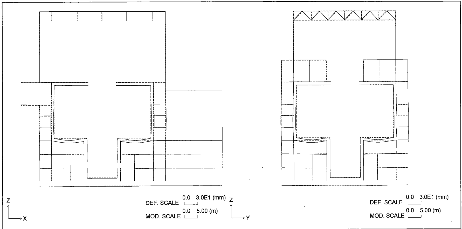
Figure 6.2.4-3 Section Deformation for Wetwell Unit Pressure (1 MPa)
