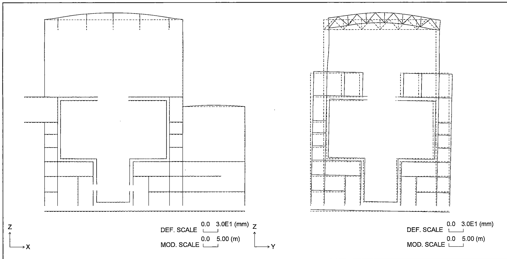
Figure 6.2.4-22 Section Deformation for Tornado Load (West Wind)
