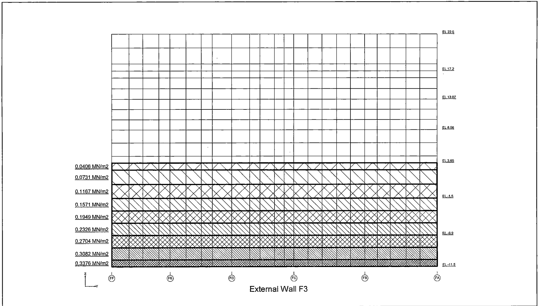
Figure 6.2.3.2-7 Lateral Soil Pressure Load at Rest (F3 External Wall)
