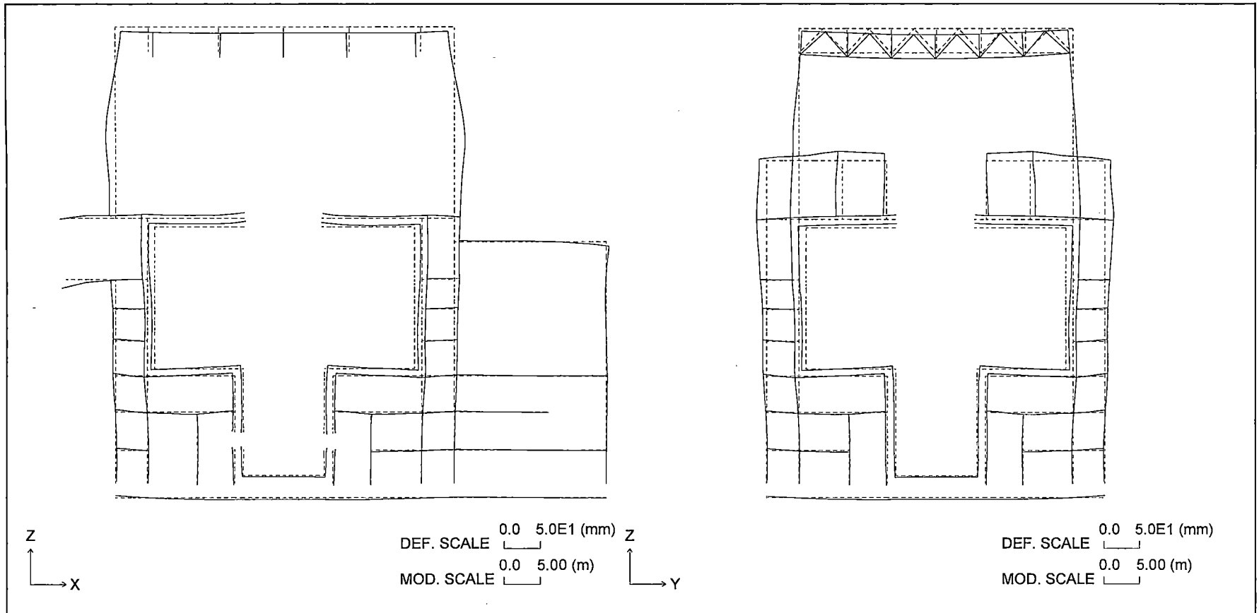
Figure 6.2.4-6 Section Deformation for Thermal Load (LOCA After 72 hr.: Winter)
