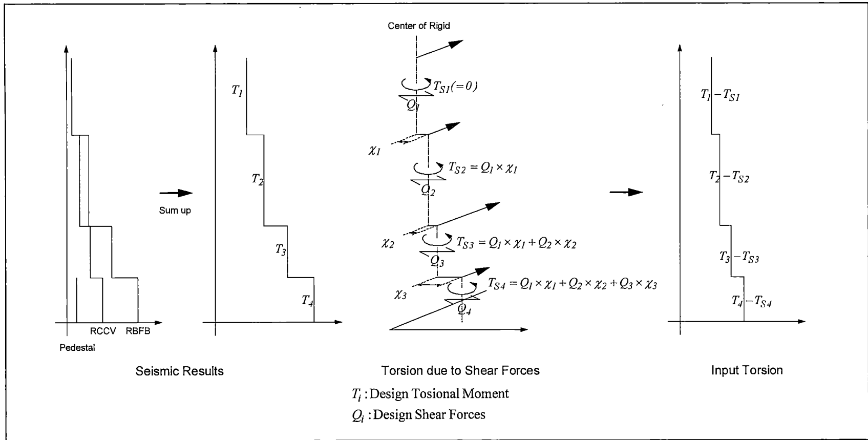
Figure 6.2.3.9-19 Calculation Method of Input Torsional Moment
