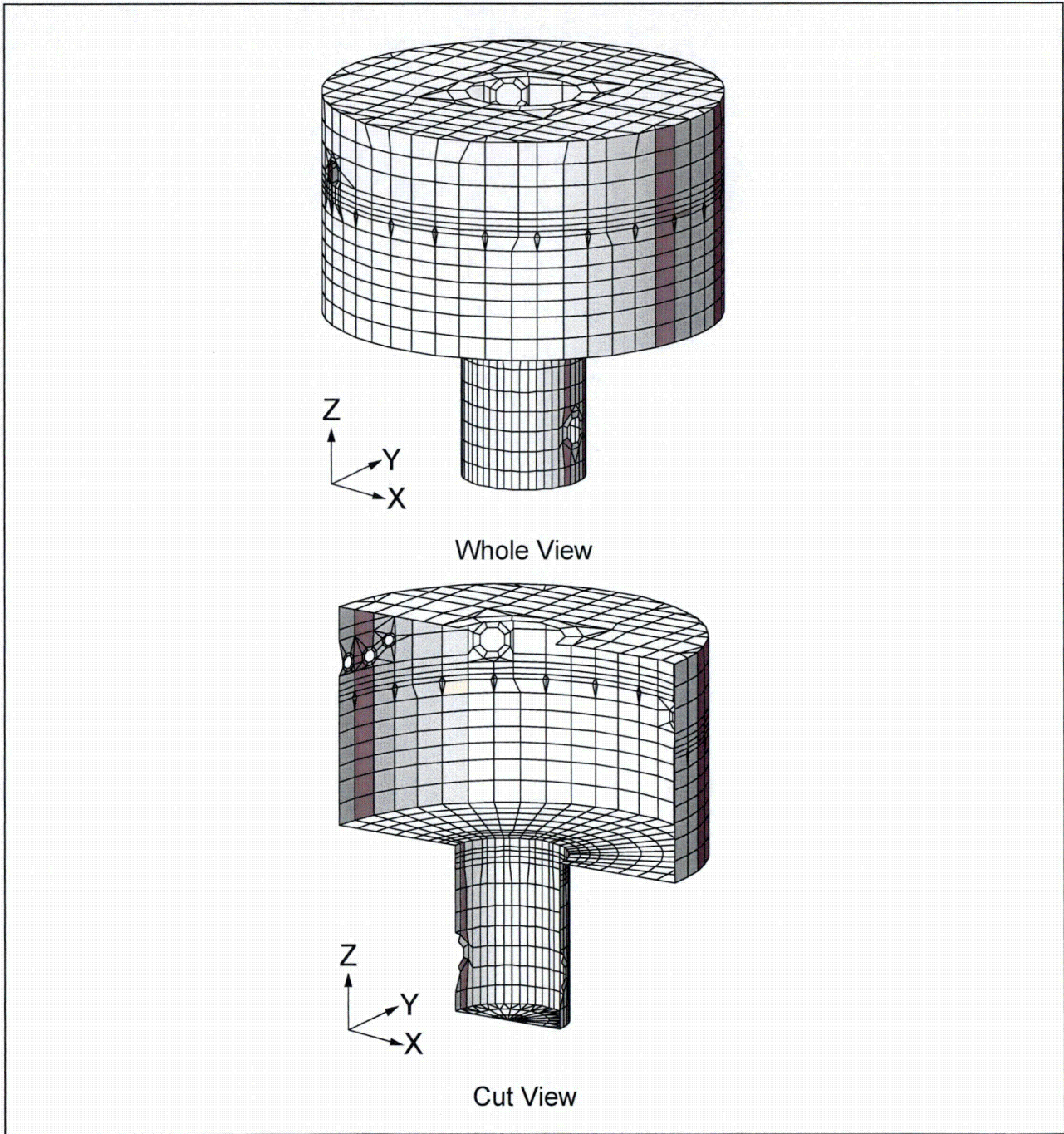
Figure 6.2.2-3 FE Model of RCCV Liner
