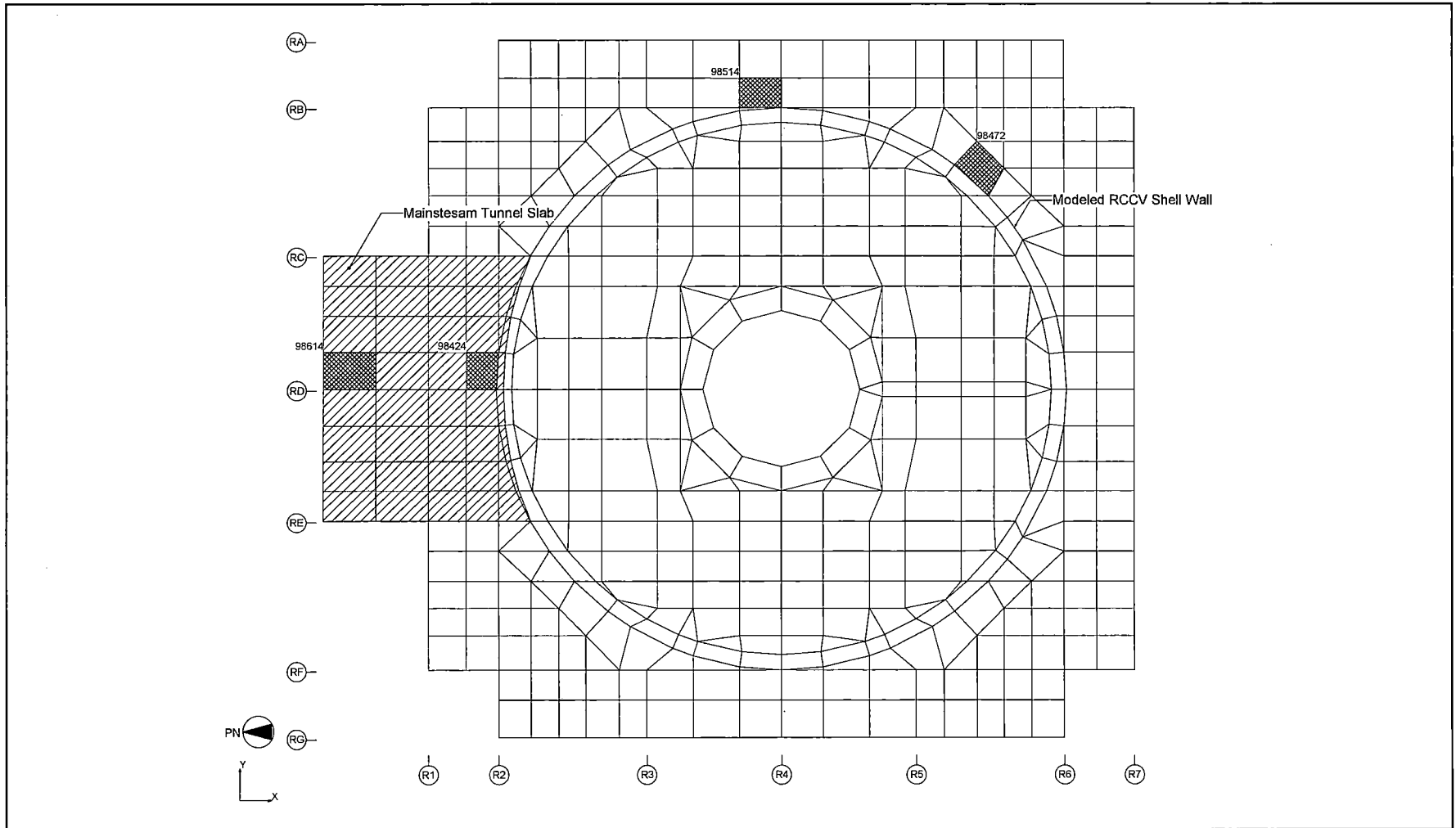
Figure 6.2.4-31 Elements Selected for Tabulation (Slab at EL 27,000)
