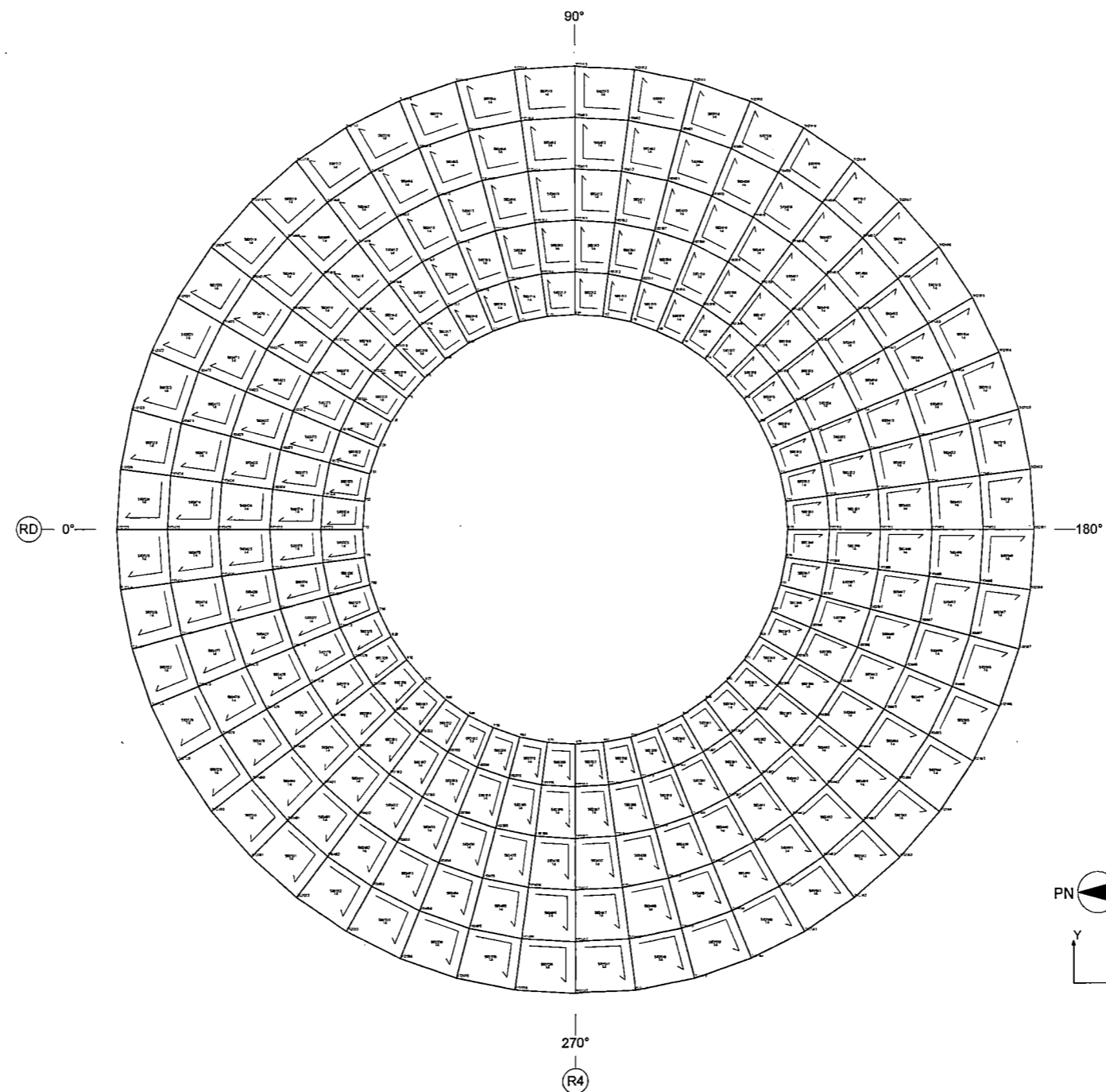
Figure 6.2.2-14 FE Model of the Suppression Pool Floor Slab Liner (EL 4,650)
