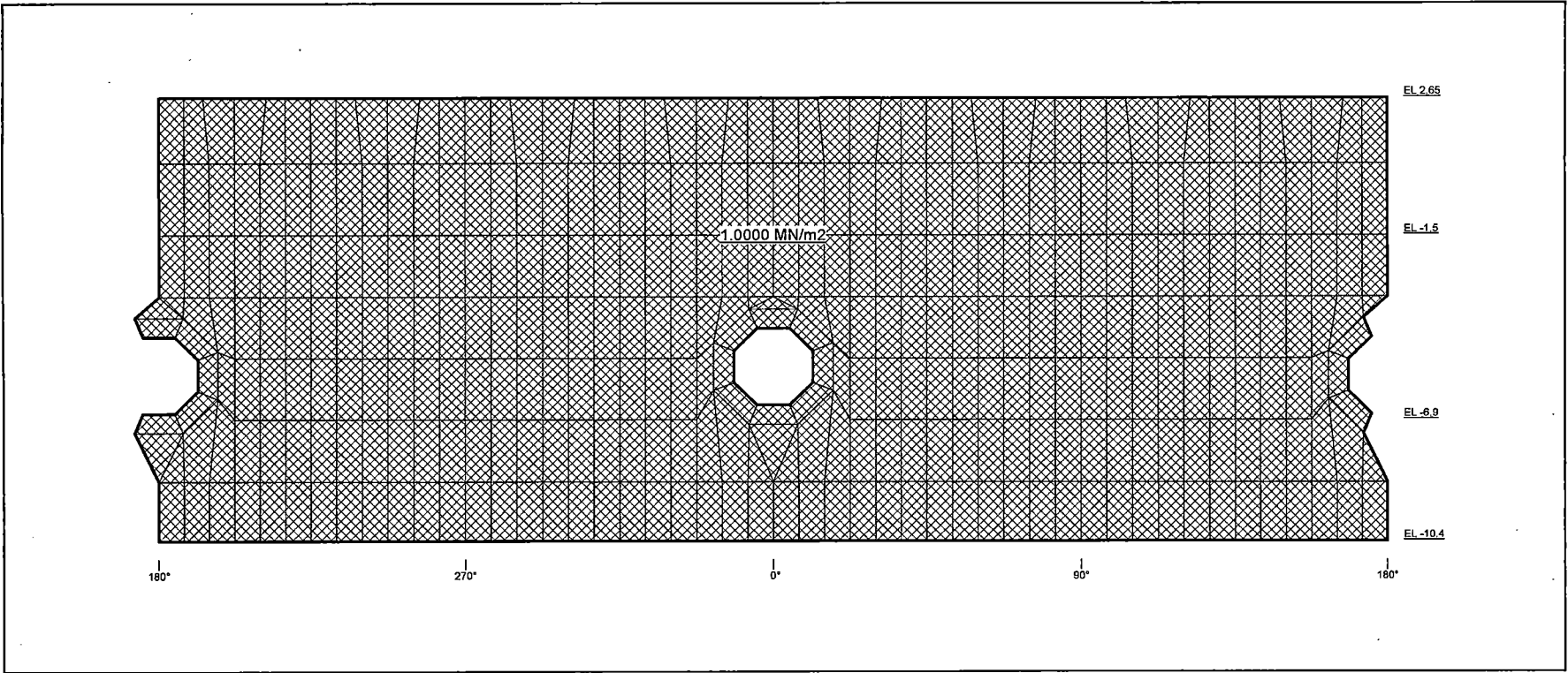
Figure 6.2.3.3-4 Containment Pressure Load (Drywell: RPV Pedestal Liner)
