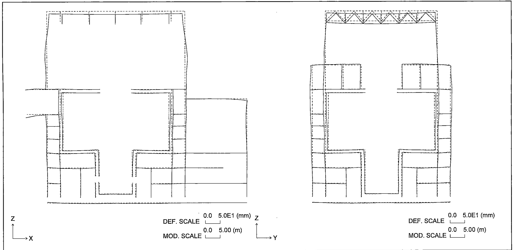
Figure 6.2.4-5 Section Deformation for Thermal Load (LOCA After 6 min.: Winter)
