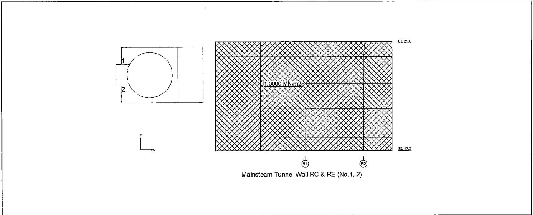
Figure 6.2.3.3-24 HELB Pressure Load (MS Tunnel: Walls)
