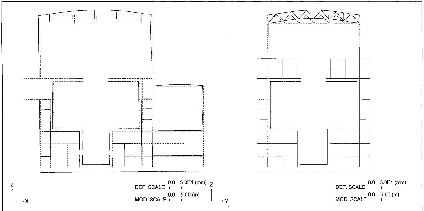
Figure 6.2.4-20 Section Deformation for Tornado Load (South Wind)
