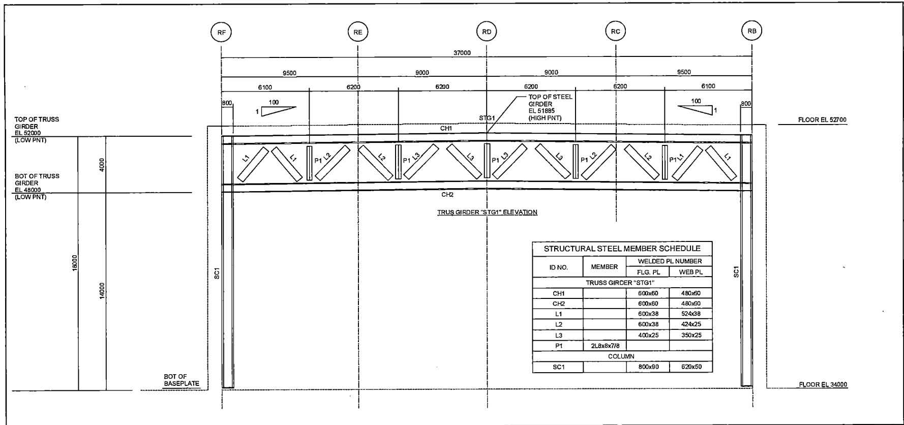
Figure 7.1-5 RB Roof Truss Structural Steel Member
