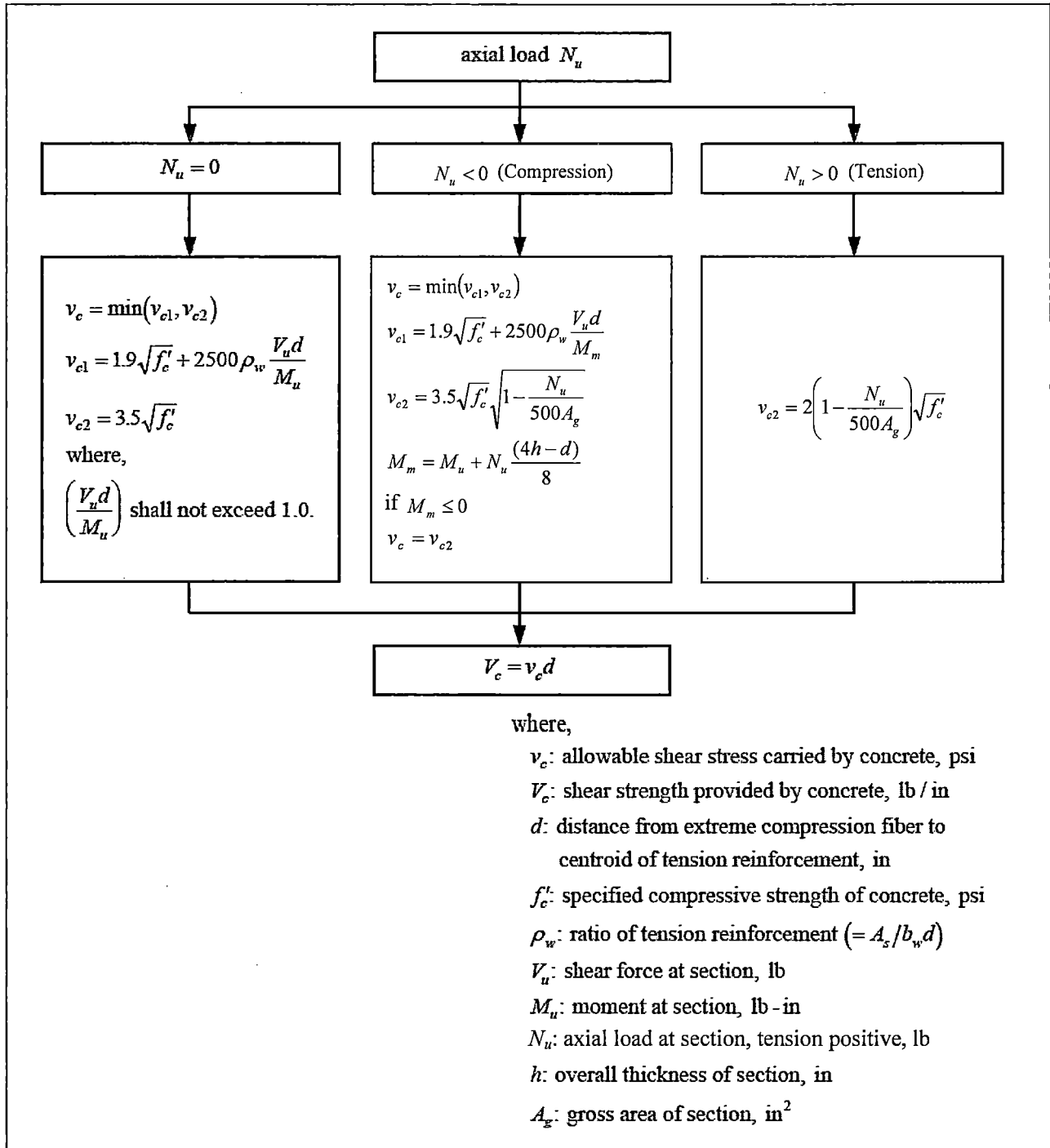
Figure 6.4.1-2 Calculation of Shear Strength Provided by Concrete
