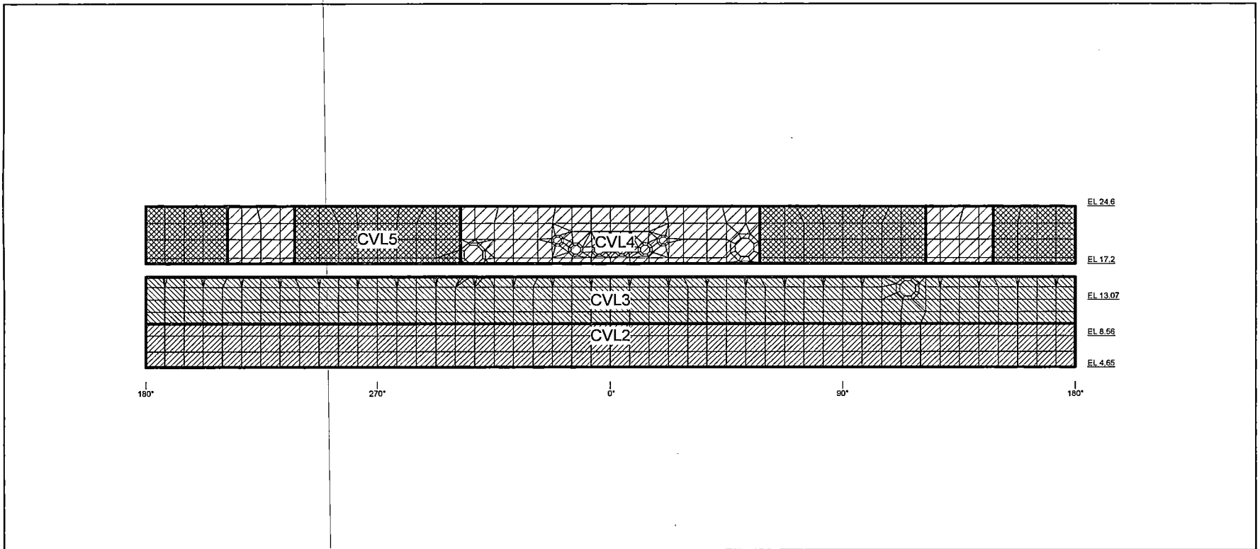
Figure 6.2.3.4-27 Application of Thermal Load on the RCCV Liner (Normal Operation)
