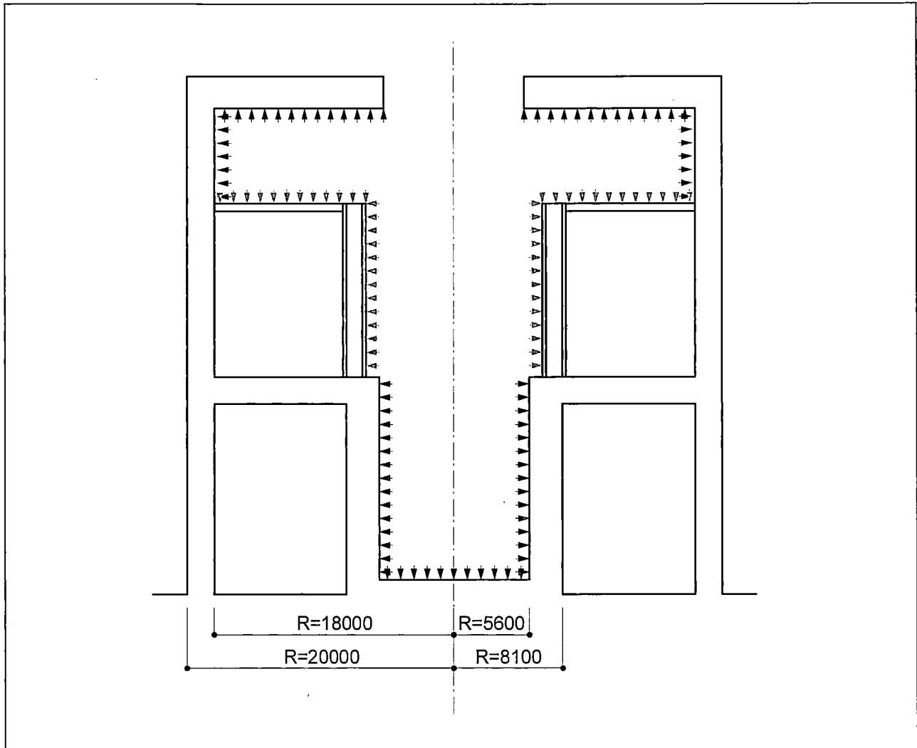
Figure 6.2.3.3-1 Containment Pressure Loads - Drywell Unit Pressure
