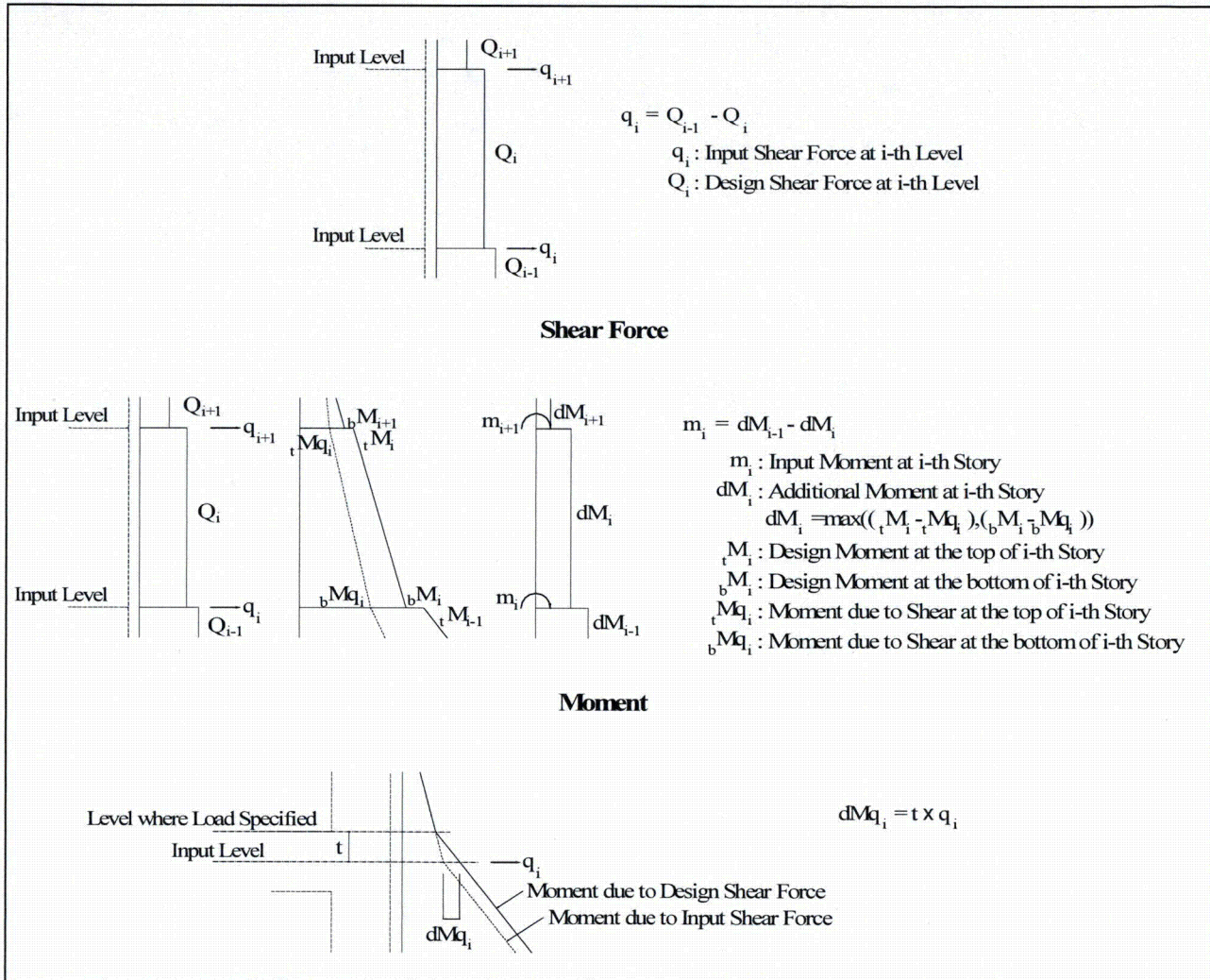
Figure 6.2.3.9-2 Calculation of Applied Shear Forces and Moments
