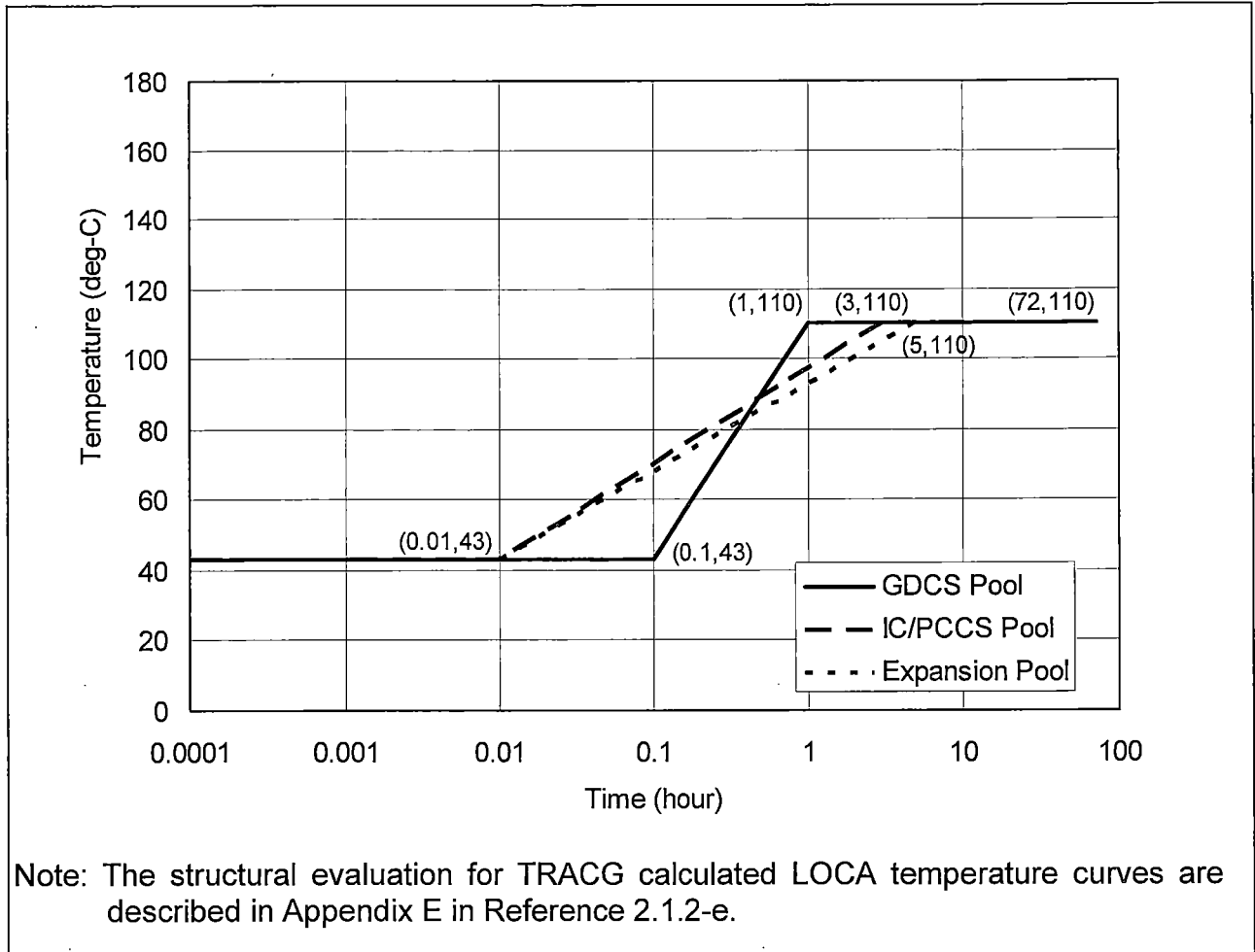
Figure 5.2.2-2 Envelopes of Transient Temperature Curves – Other Pools at DBA
