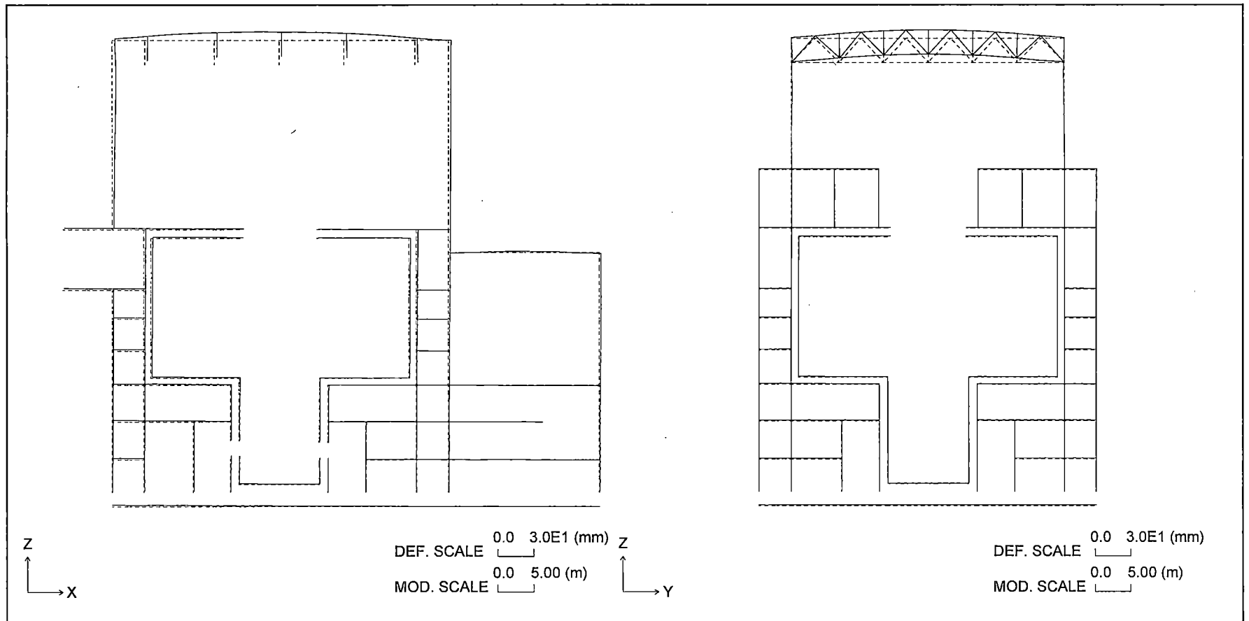
Figure 6.2.4-15 Section Deformation for Wind Load (North Wind)
