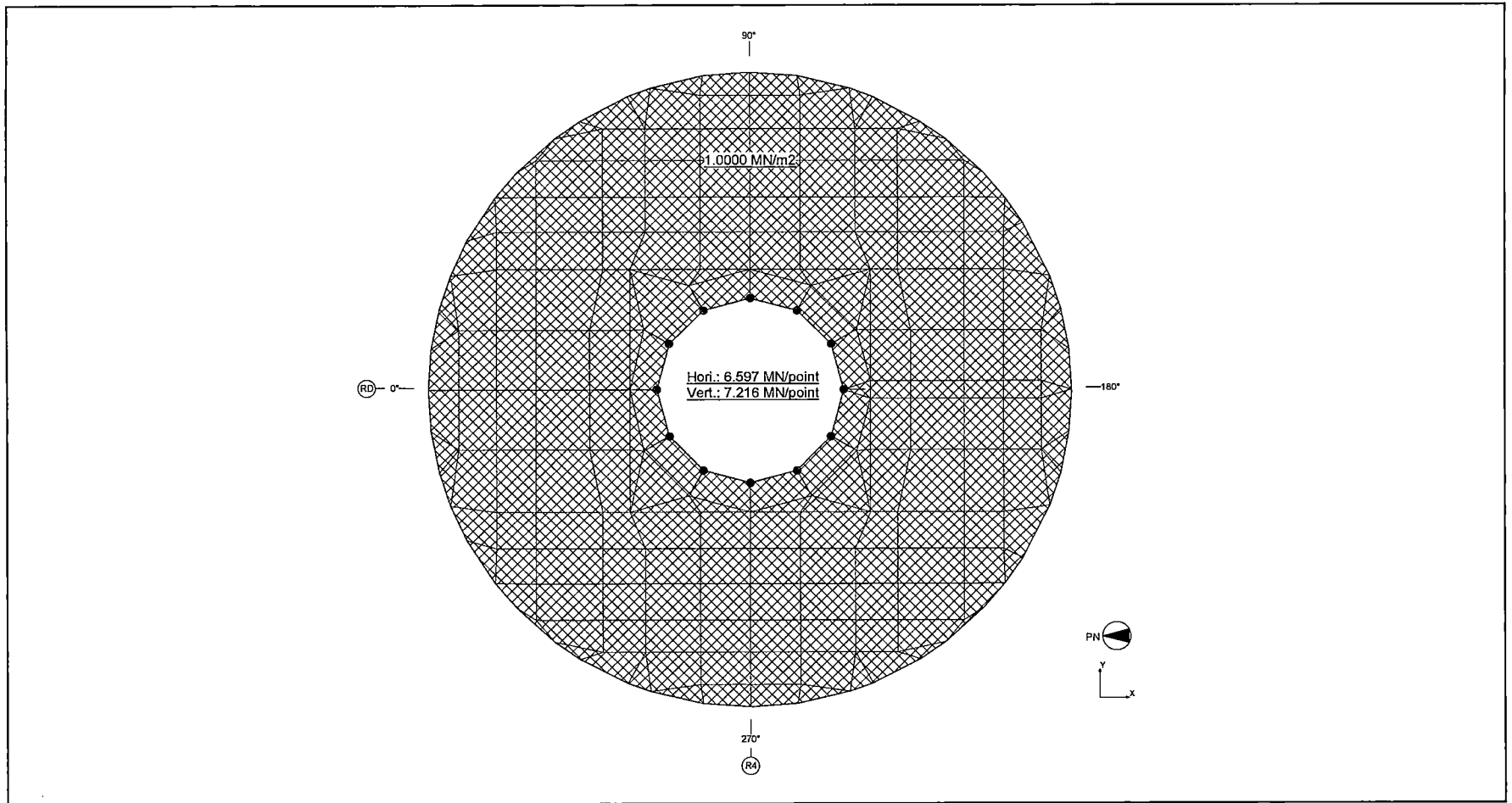
Figure 6.2.3.3-6 Containment Pressure Load (Drywell: Topslab Liner)
