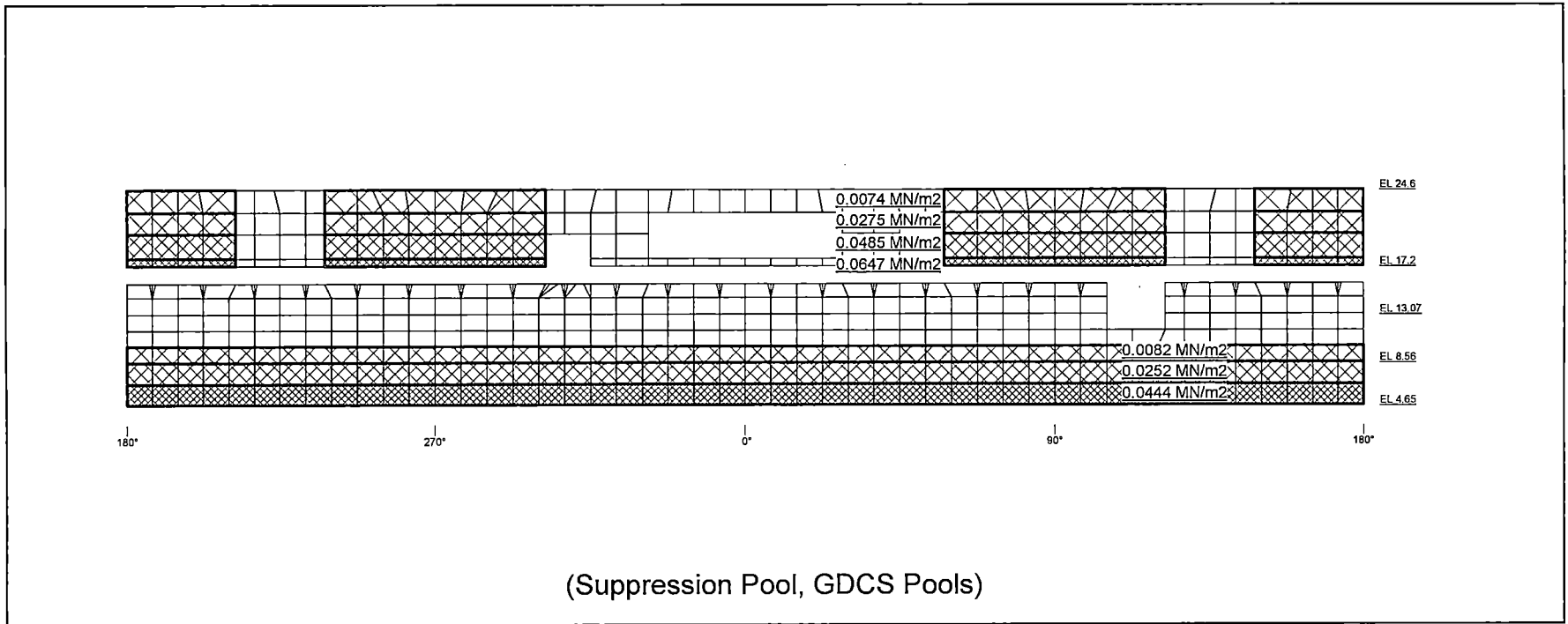
Figure 6.2.3.1-15 Hydrostatic Loads on the RCCV Wall Liner
