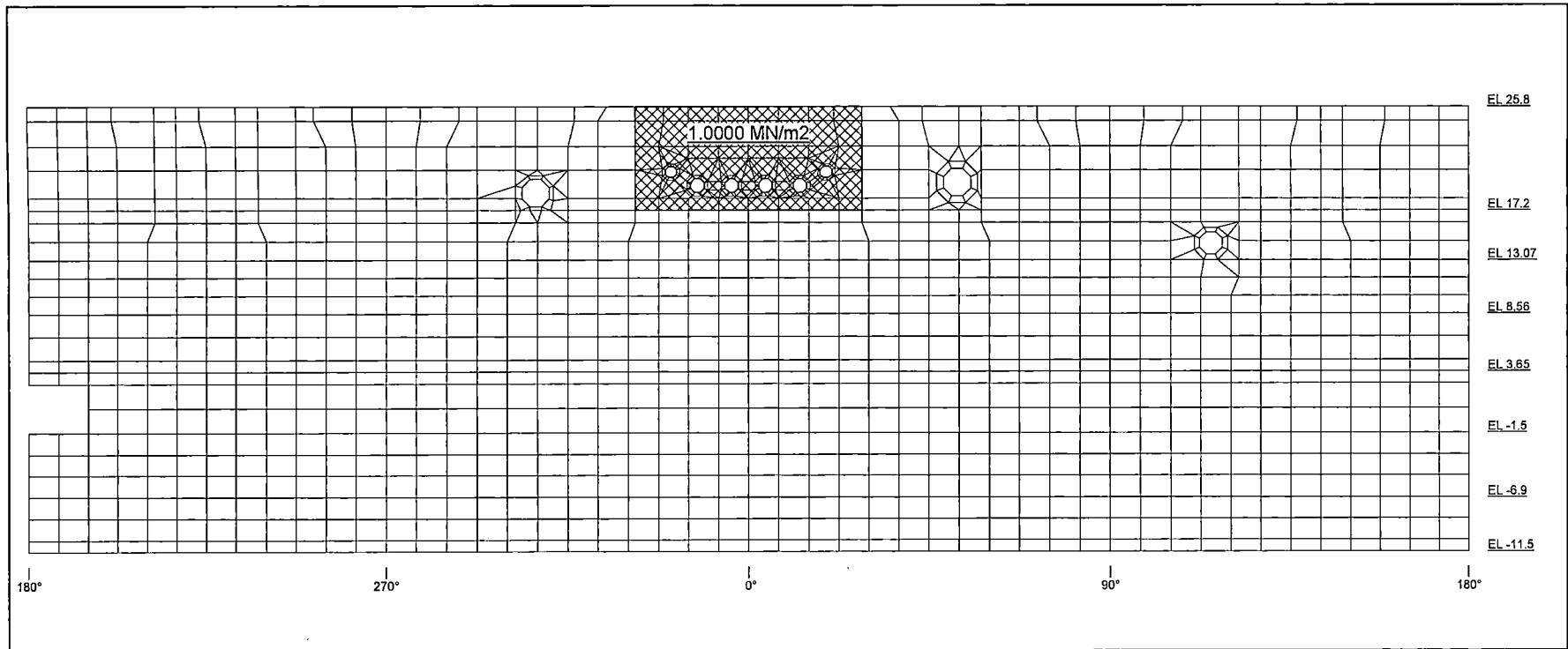
Figure 6.2.3.3-23 HELB Pressure Load (MS Tunnel: RCCV Wall)
