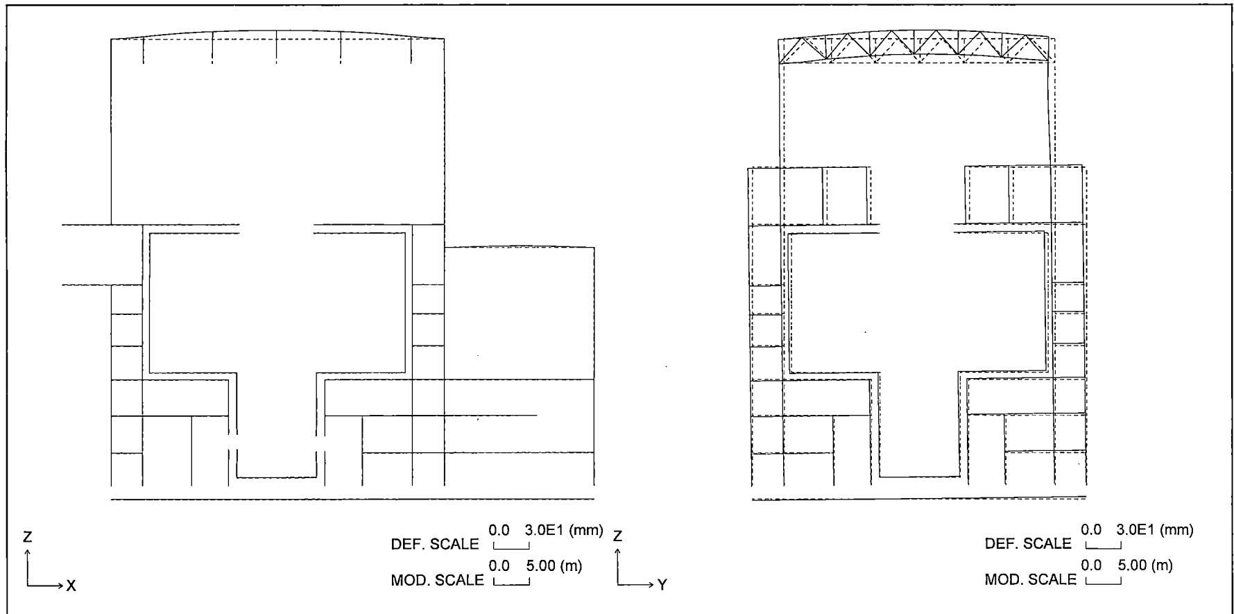
Figure 6.2.4-17 Section Deformation for Wind Load (East Wind)
