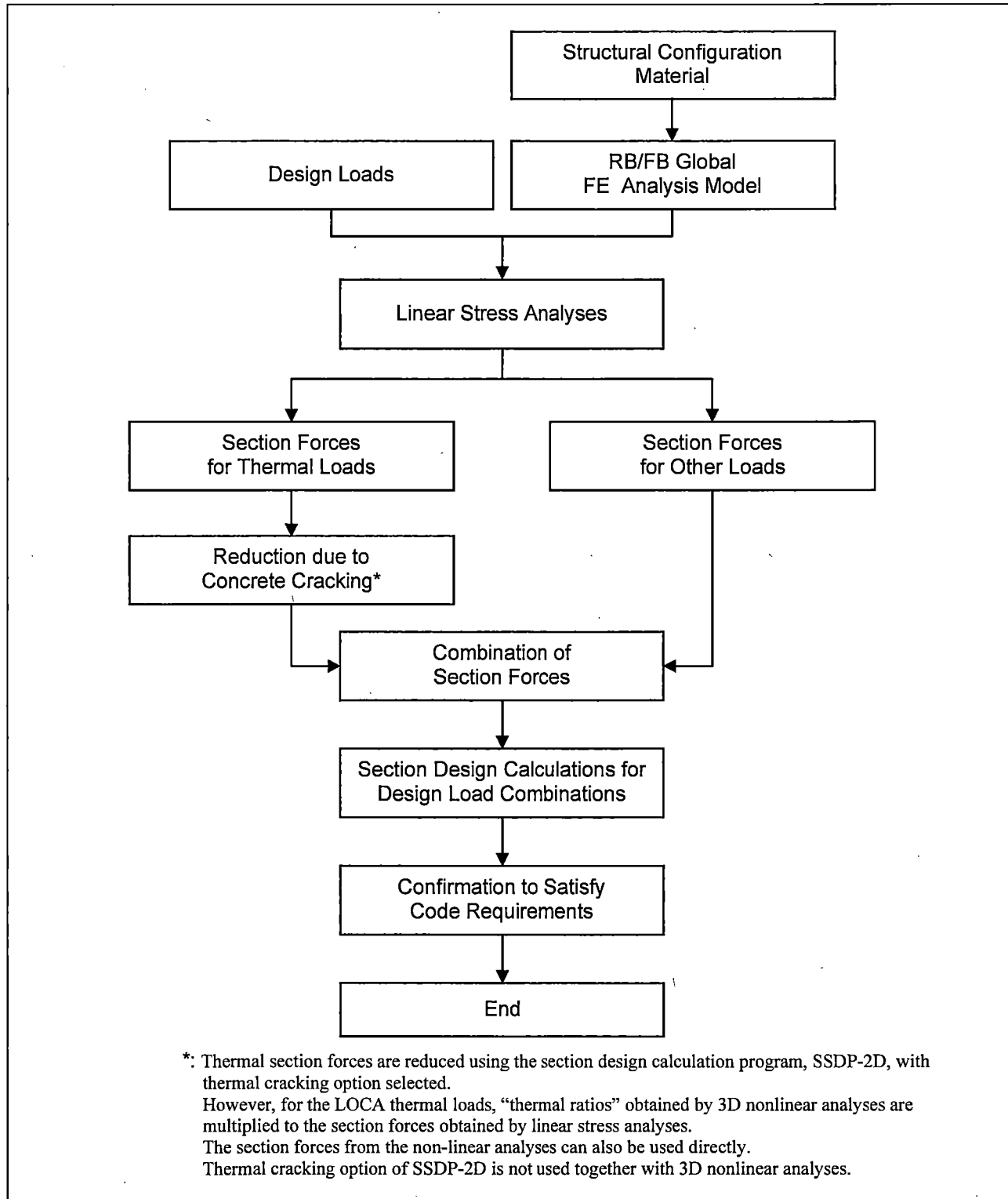
Figure 6.4.1-1 Flow Chart of Design for Reinforced Concrete Structures
