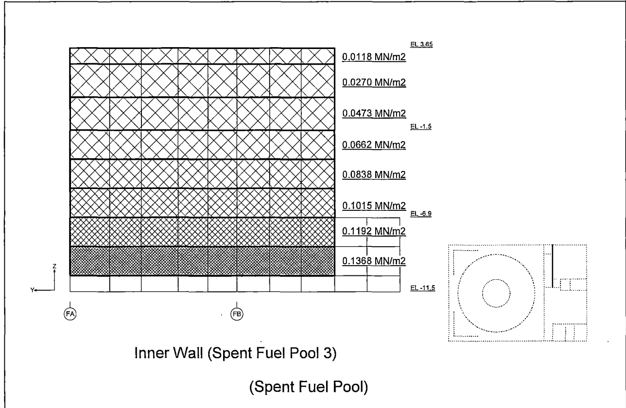
Figure 6.2.3.1-25 Hydrostatic Loads on the Inner Wall at EL -11,500 (3)
