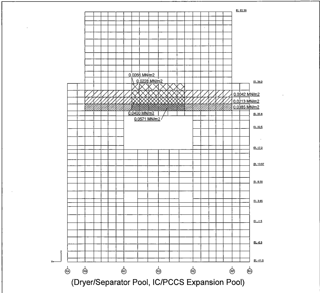
Figure 6.2.3.1-20 Hydrostatic Loads on the R1 External Wall
