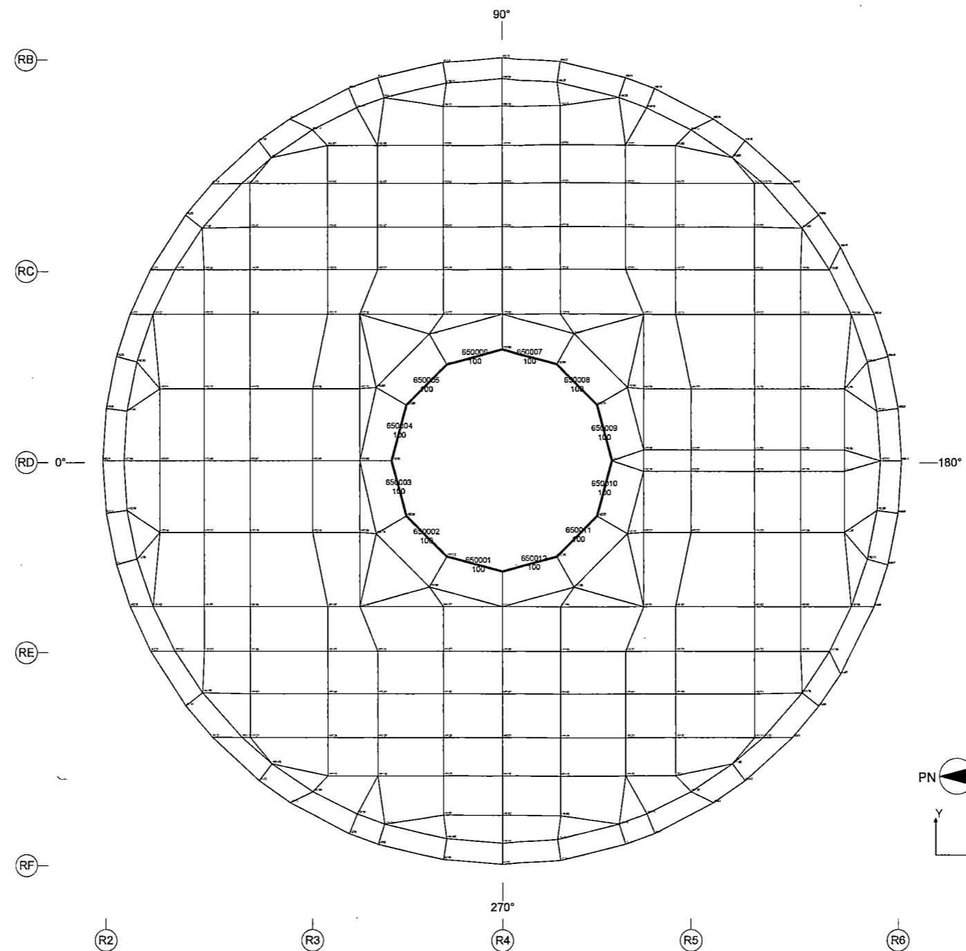
Figure 6.2.2-17 FE Model of Sleeve at the RCCV Top Head Opening
