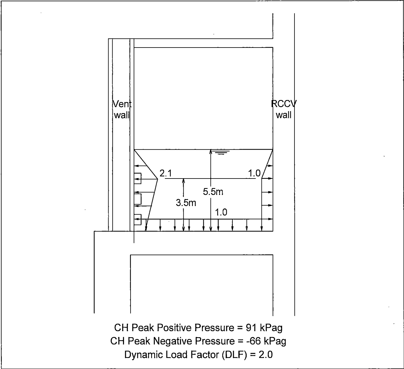
Figure 5.2.3-3 Chugging (CH) Pressure Loads
