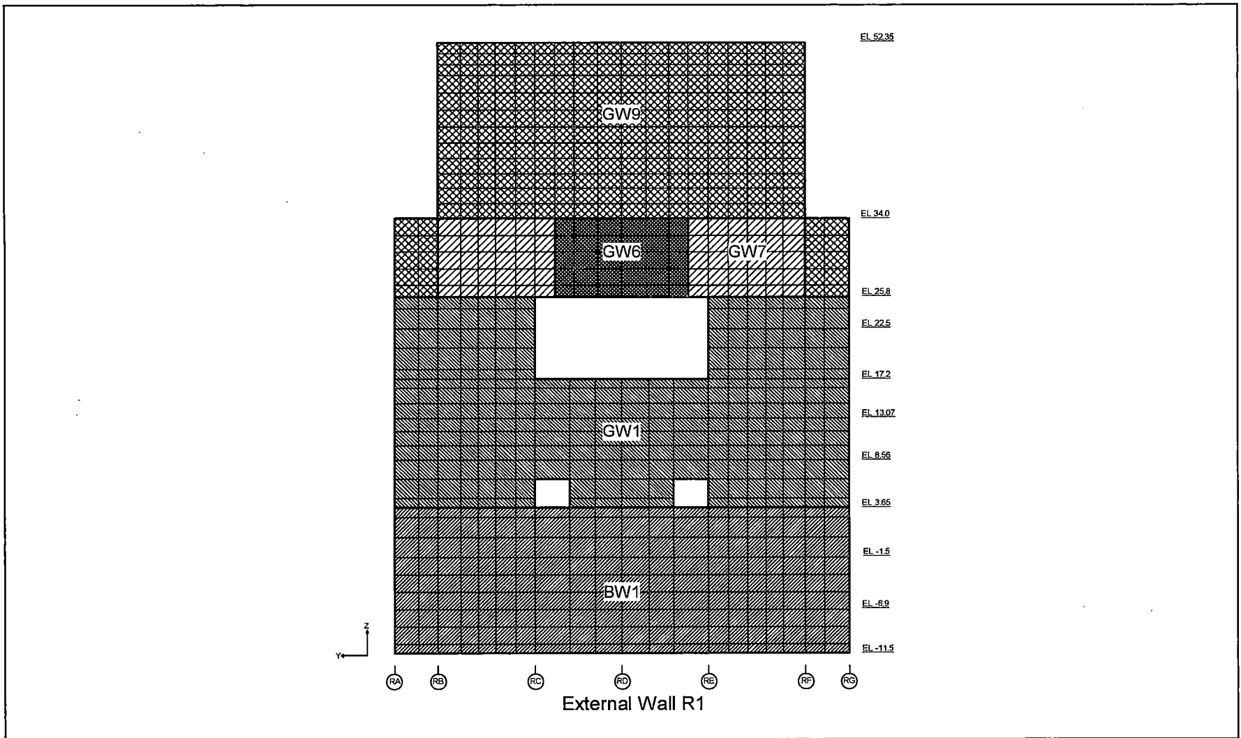
Figure 6.2.3.4-9 Application of Thermal Load on the External Wall (R1)
