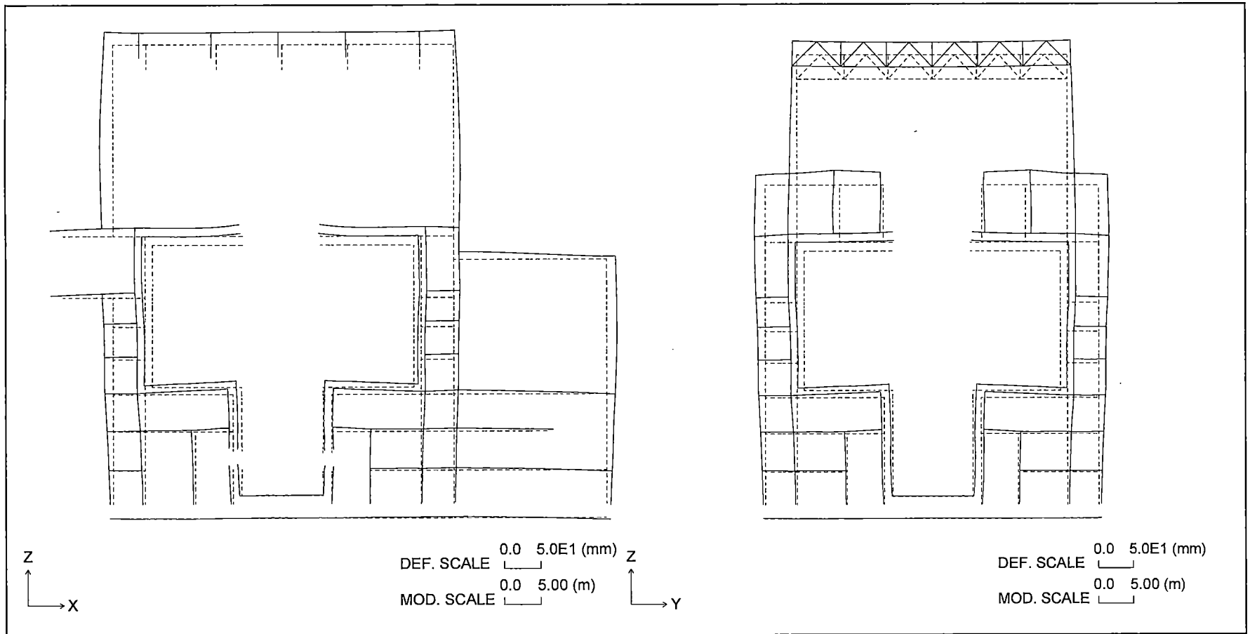
Figure 6.2.4-9 Section Deformation for Thermal Load (LOCA After 72 hr.: Summer)
