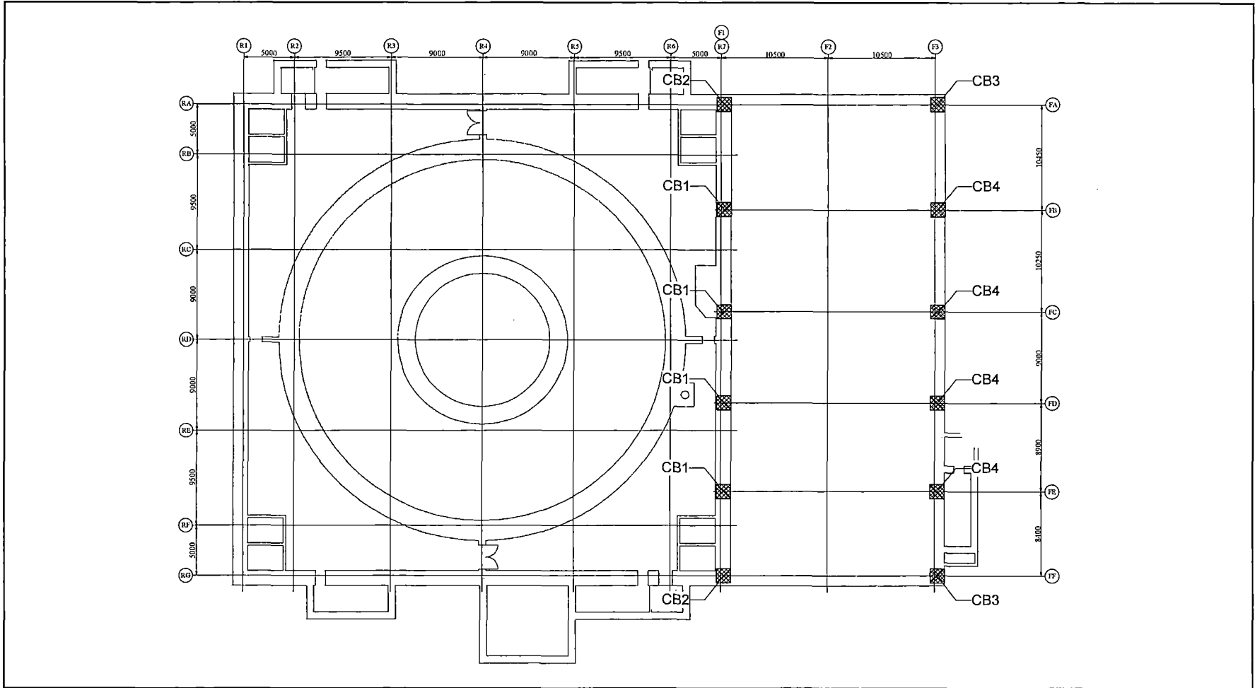
Figure 6.2.3.4-35 Application of Thermal Load on the Reinforced Concrete Girder and Column (EL 9,060)
