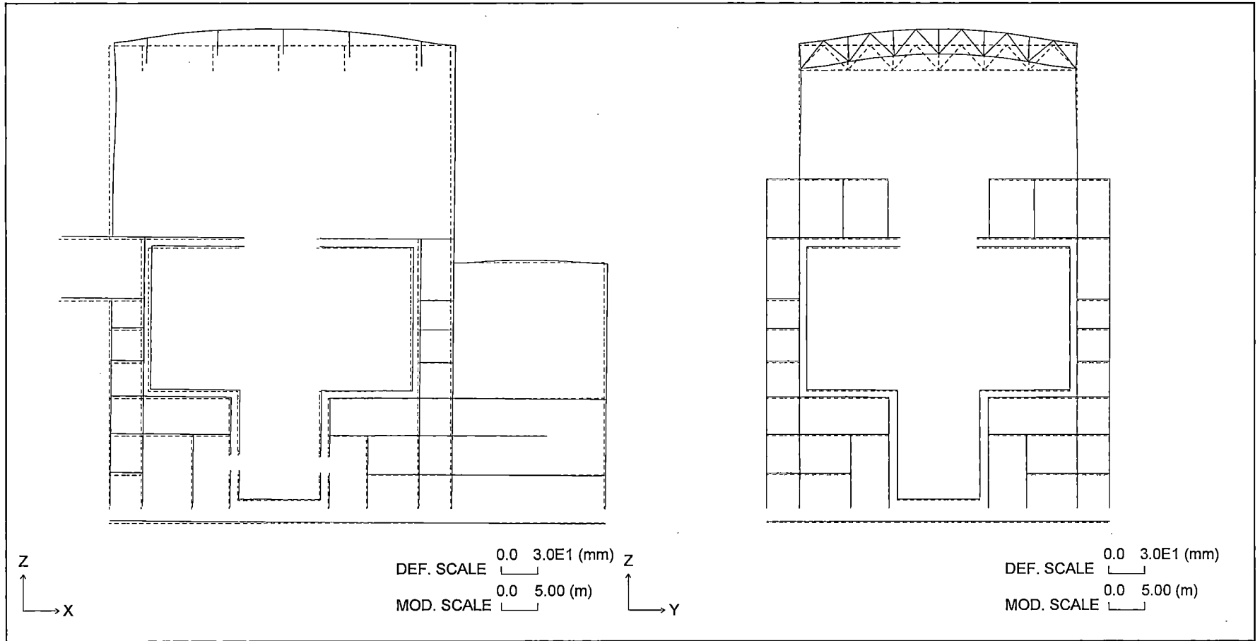
Figure 6.2.4-19 Section Deformation for Tornado Load (North Wind)
