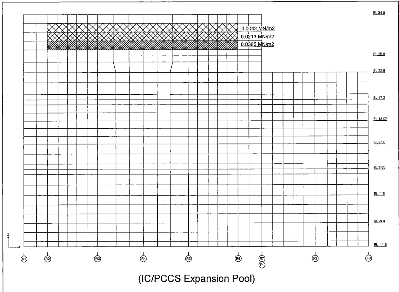
Figure 6.2.3.1-19 Hydrostatic Loads on the RG/FF External Wall
