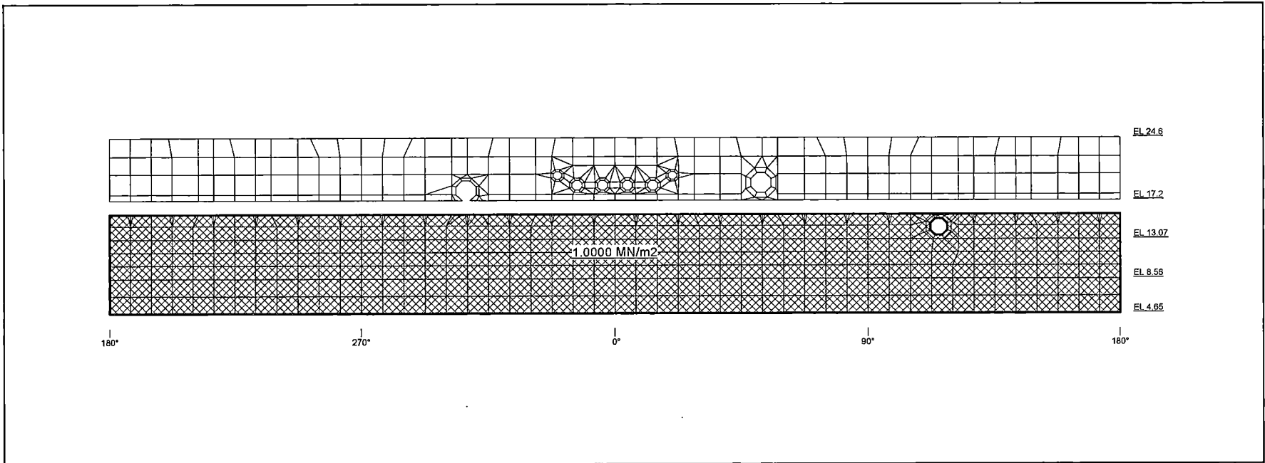
Figure 6.2.3.3-7 Containment Pressure Load (Wetwell: RCCV Liner)
