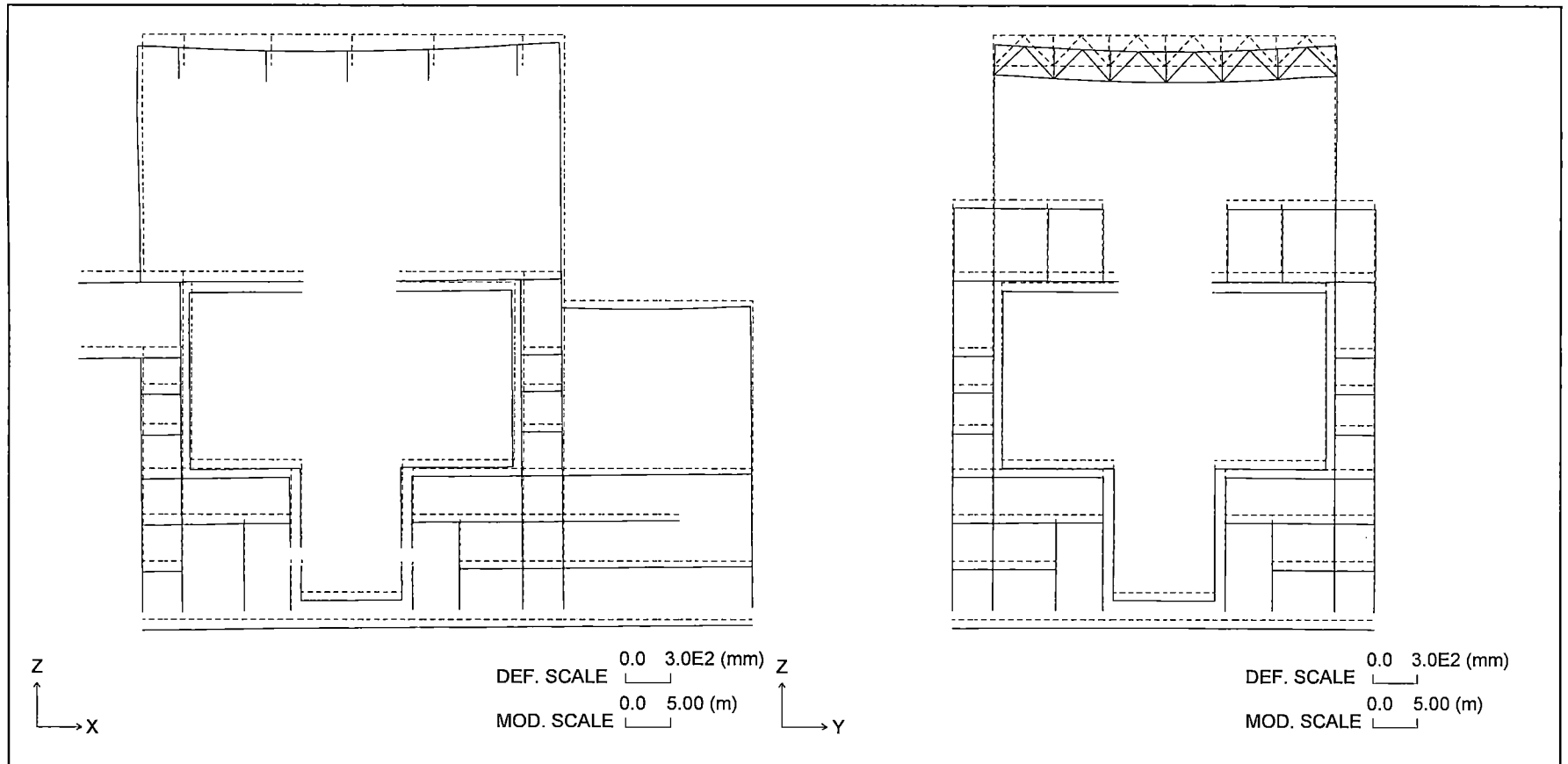
Figure 6.2.4-1 Section Deformation for Dead Load
