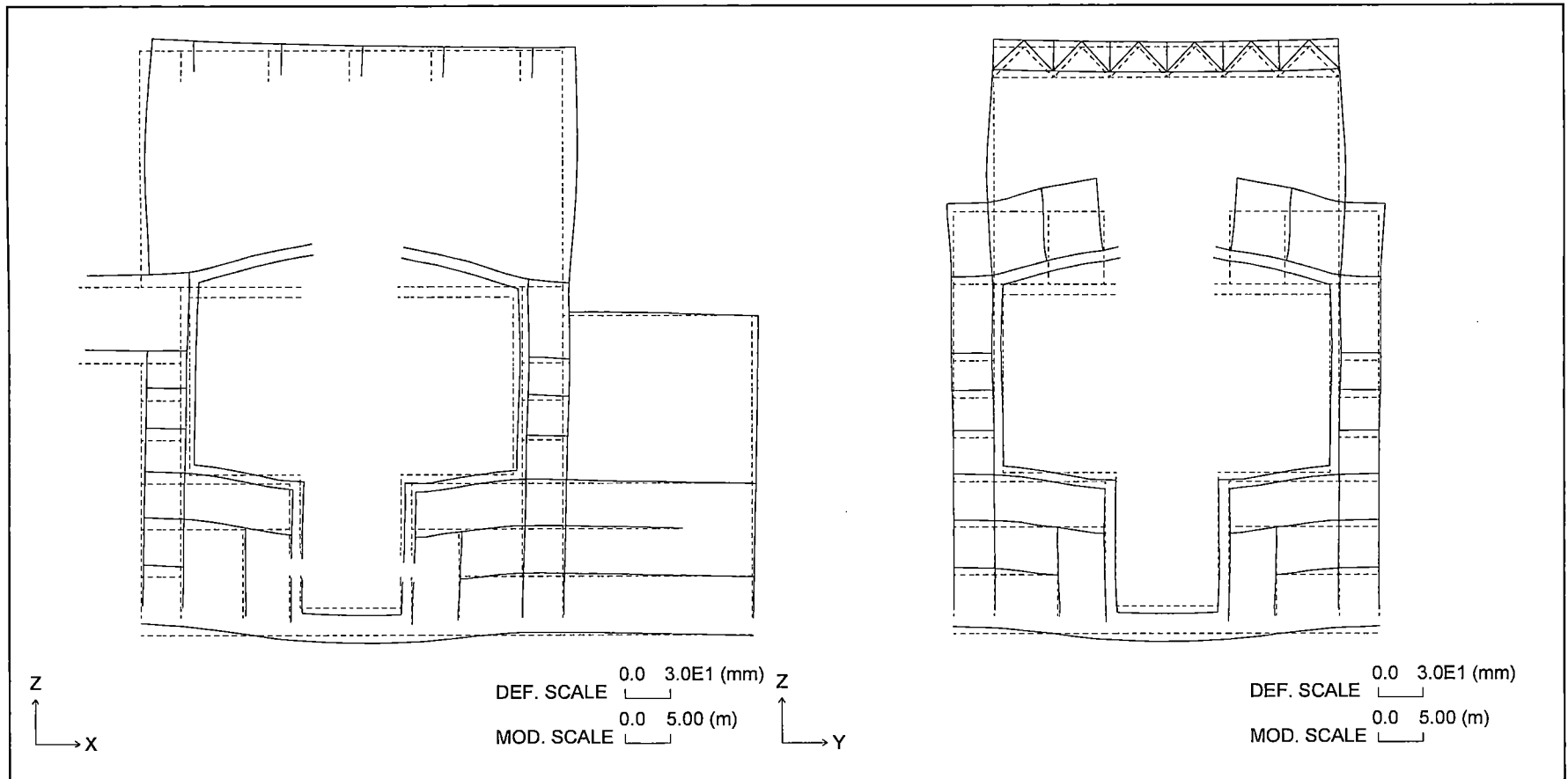
Figure 6.2.4-2 Section Deformation for Drywell Unit Pressure
