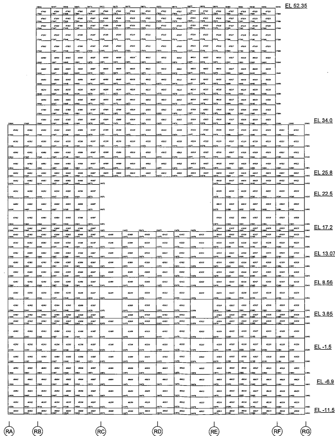
Figure 6.2-25 FE Model of the External Wall (R1 Column Line)
