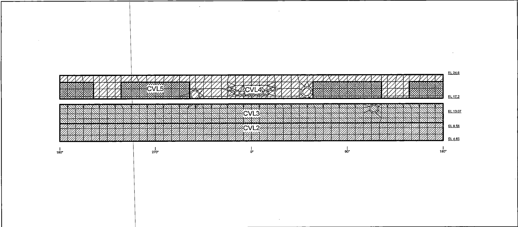
Figure 6.2.3.4-28 Application of Thermal Load on the RCCV Liner (Condition 1)
