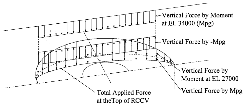
Y-direction Moment
