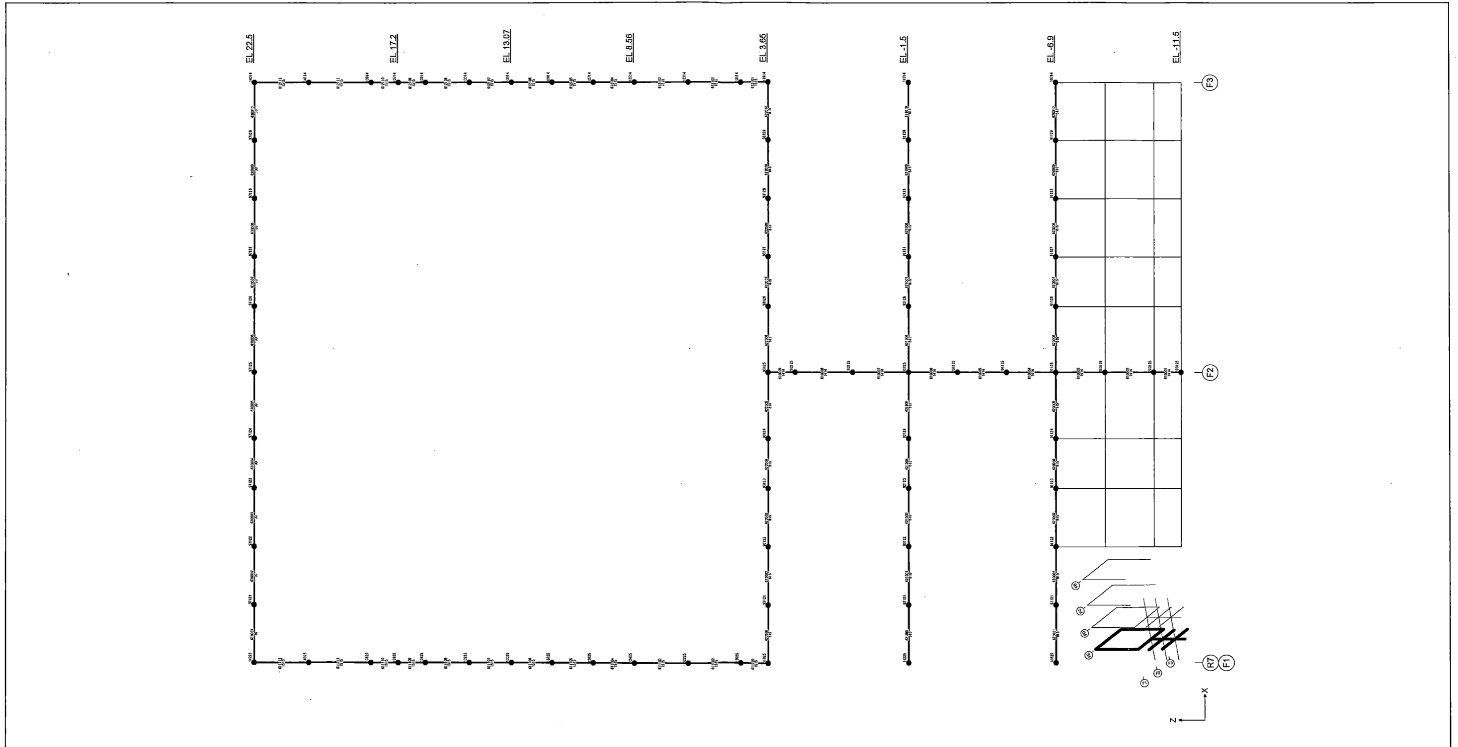
Figure 6.2.2-34 FE Model of the FB Frame (FE Column Line)
