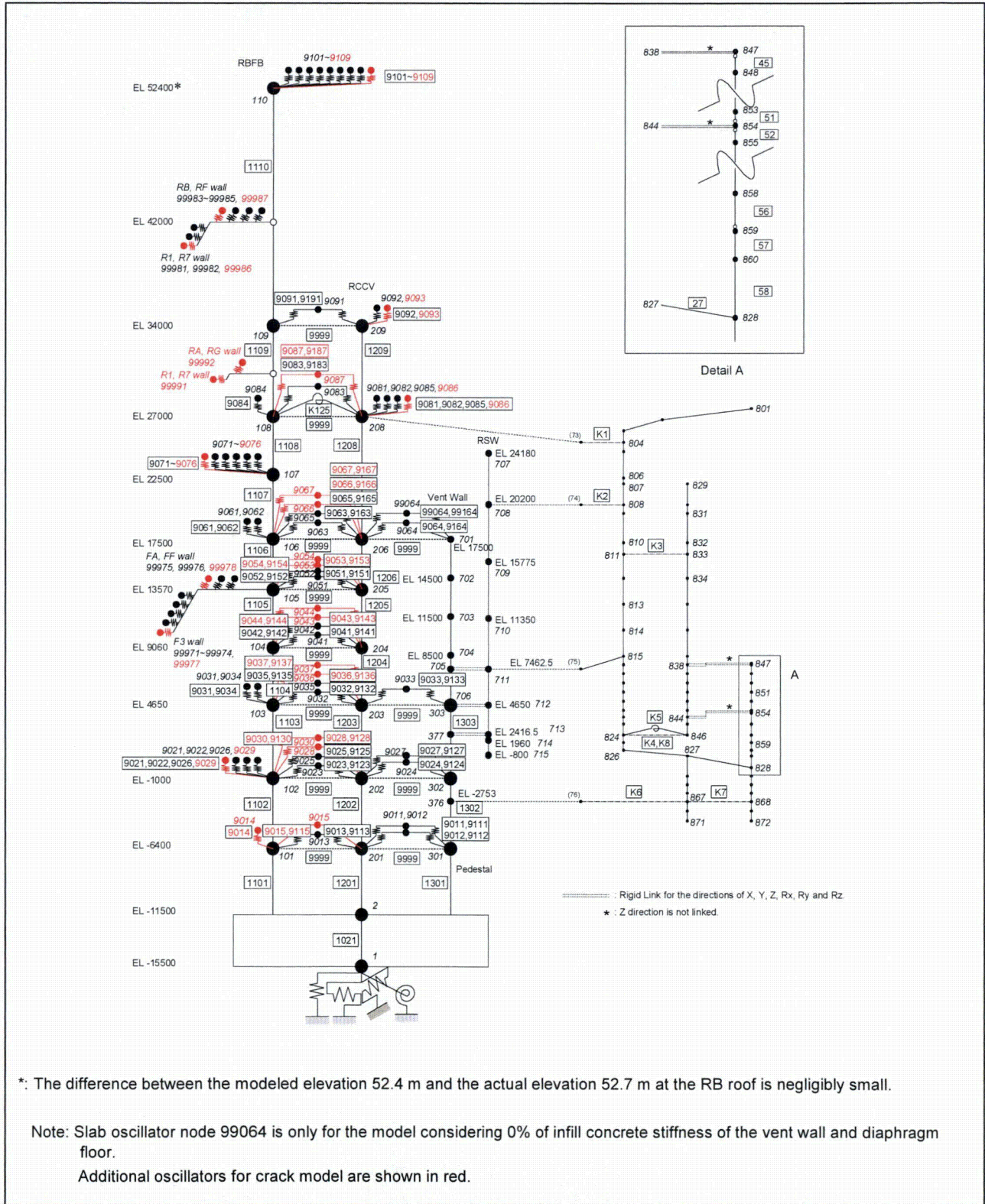
Figure 5.3.3-1 Dynamic Analysis Model
