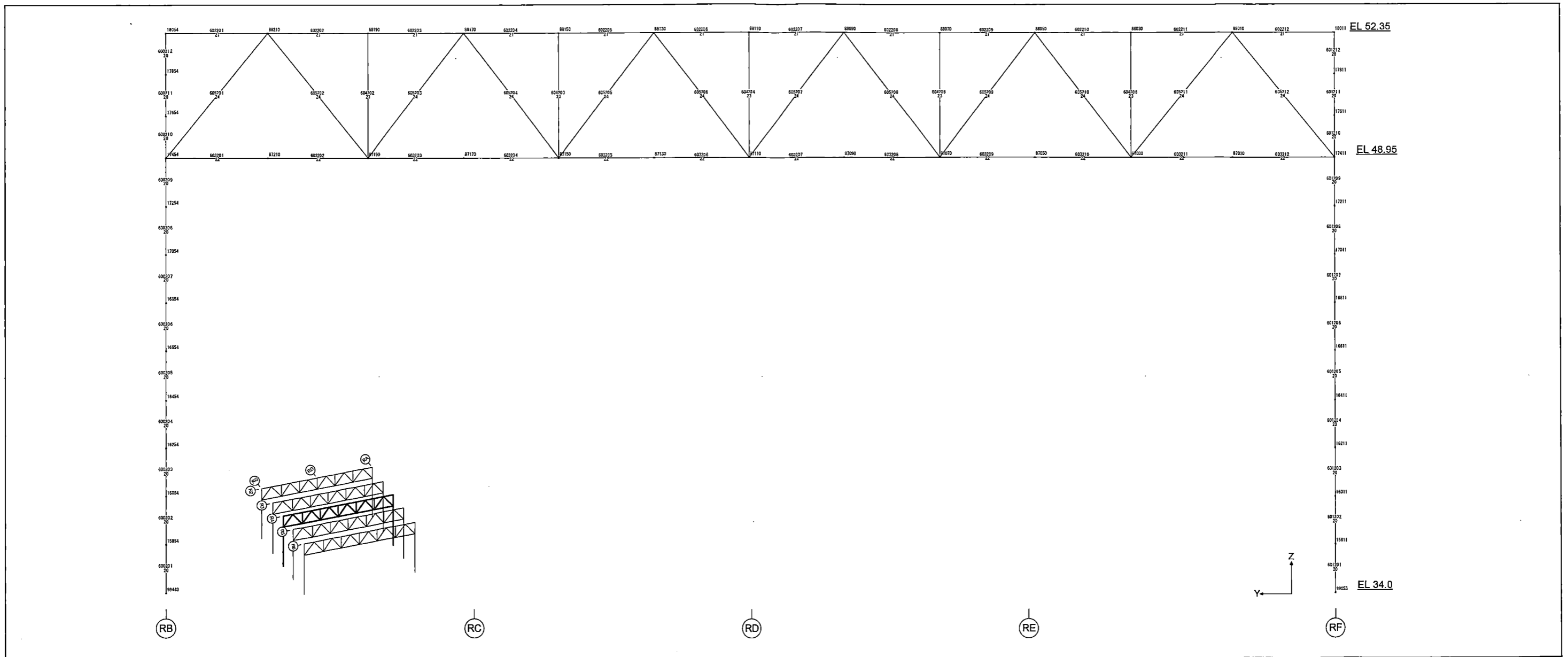
Figure 6.2.2-36 FE Model of the Roof Truss (R4 Column Line)
