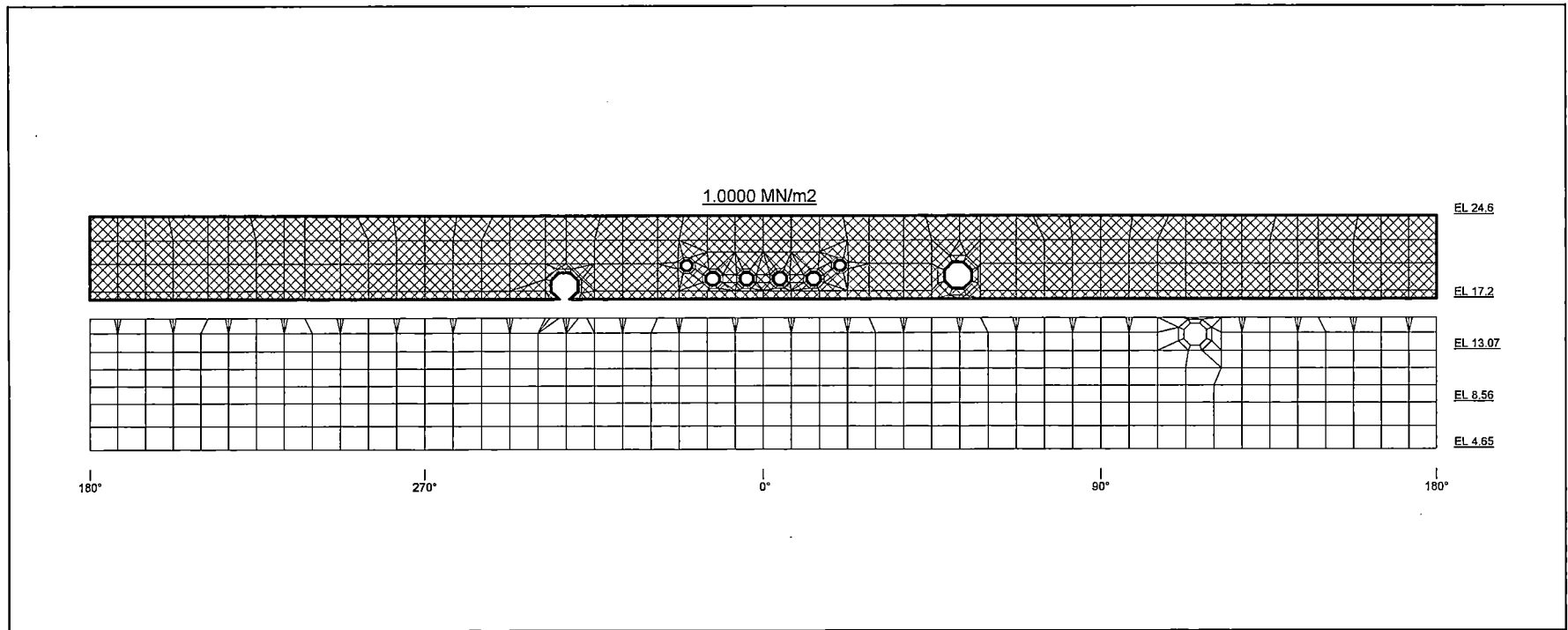
Figure 6.2.3.3-3 Containment Pressure Load (Drywell: RCCV Liner)
