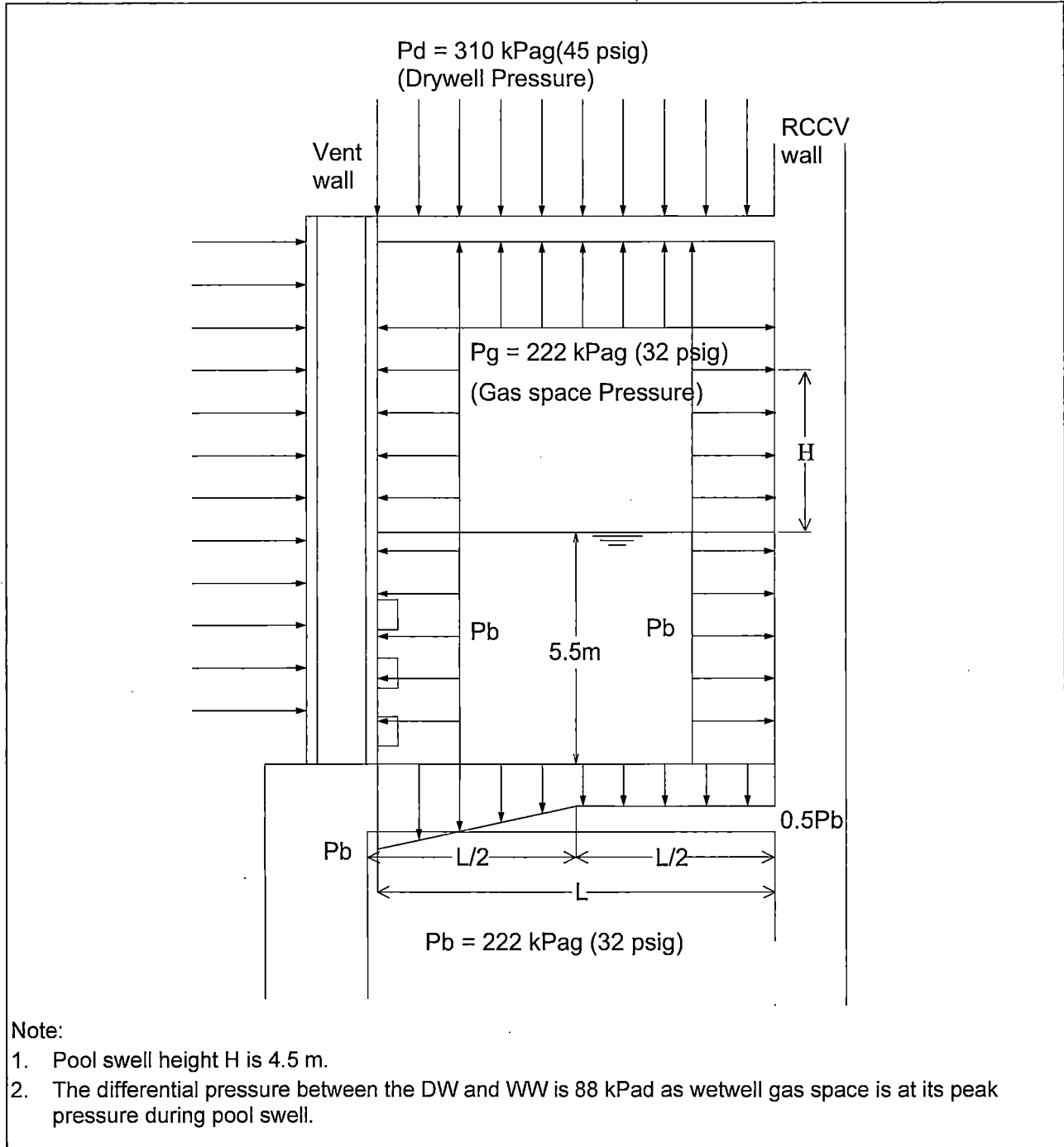
Figure 5.2.3-6 Pool Swell (PS) Pressure Concurrent with Froth Impact Loads
