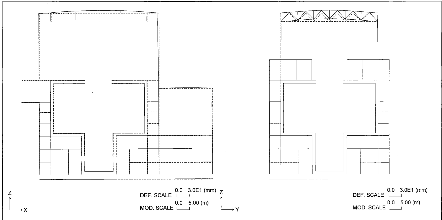
Figure 6.2.4-16 Section Deformation for Wind Load (South Wind)
