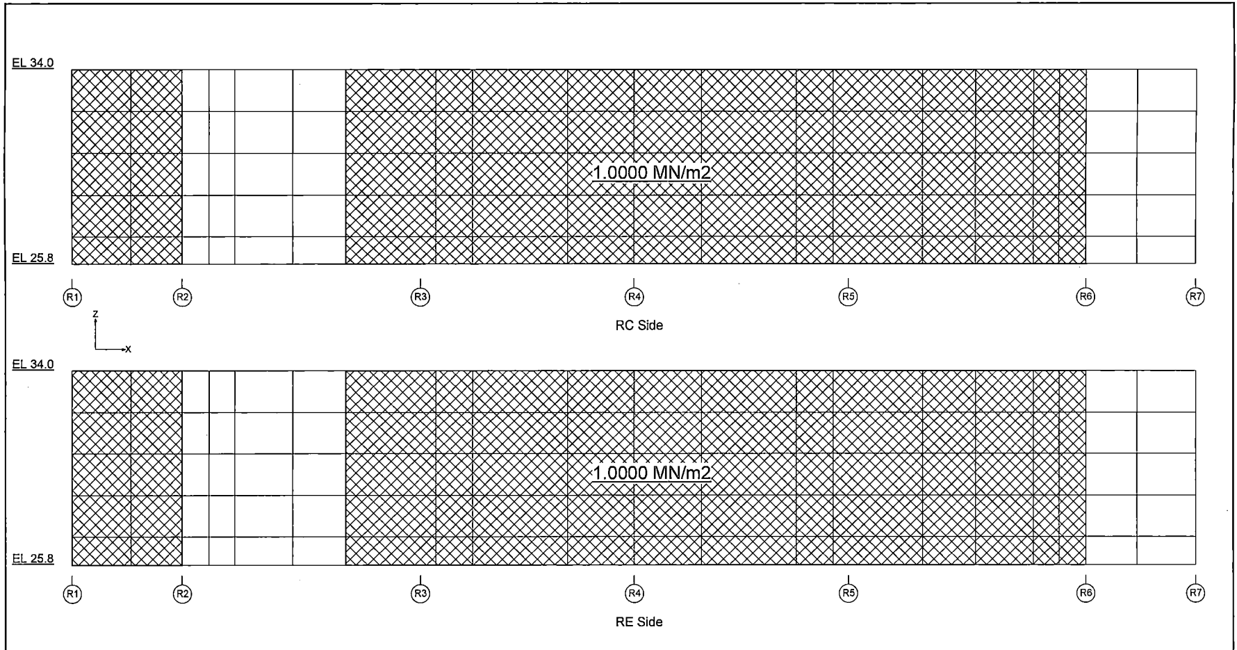
Figure 6.2.3.3-18 Containment Pressure Load (IC/PCCS Pool: Pool Girder)
