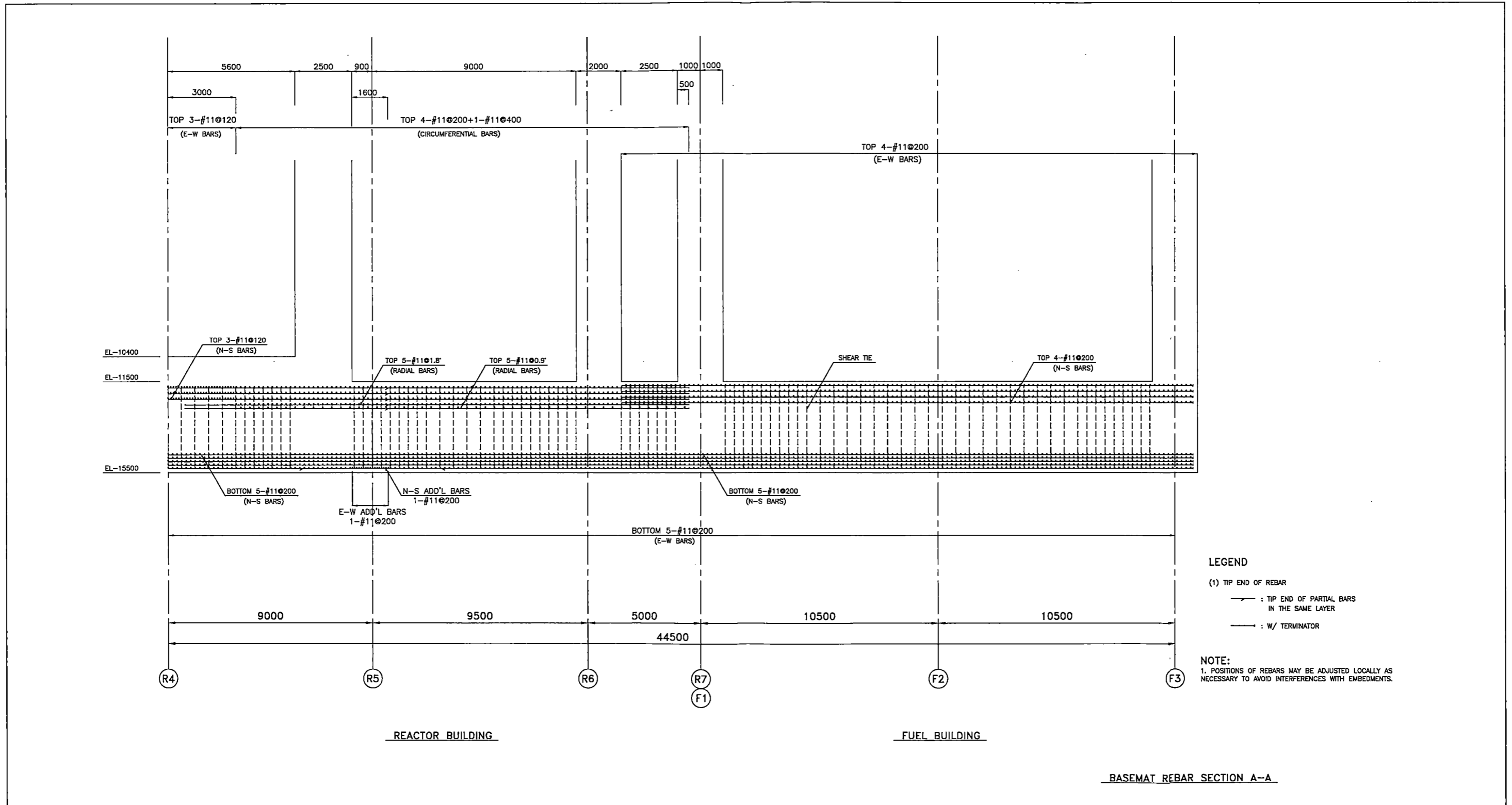
Figure 7.1-2 Reinforcing Steel of Foundation Mat: Section A-A
