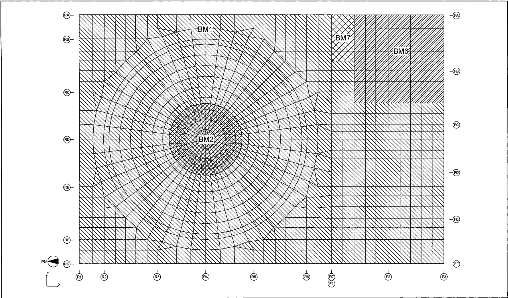
Figure 6.2.3.4-12 Application of Thermal Load on the Basemat
