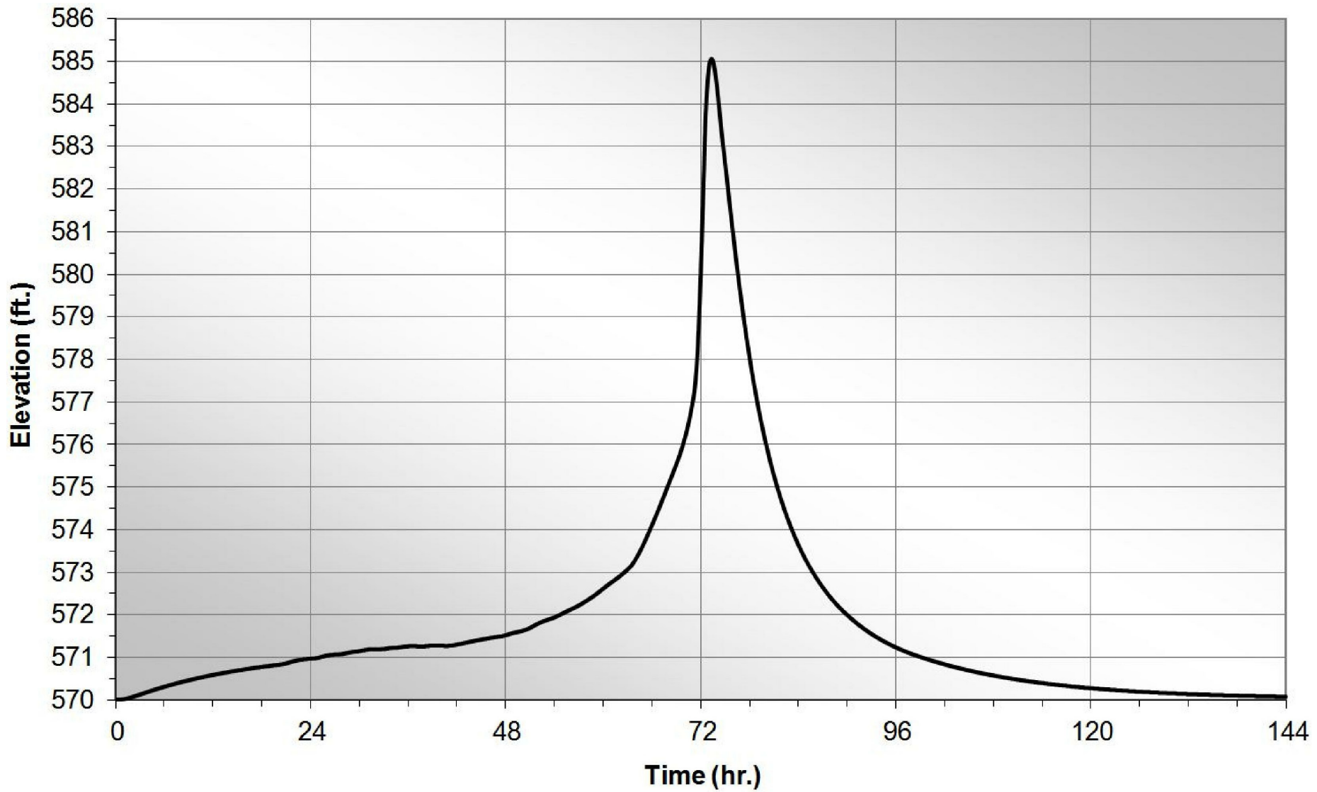
WILLIAM STATES LEE III NUCLEAR STATION UNITS 1 & 2 Flood El. Hydrograph Make-Up Pond B With Upper Arm Dam Failure, 72-hr. Local Intense Precipitation FIGURE 2.4.4-205 Rev 7
