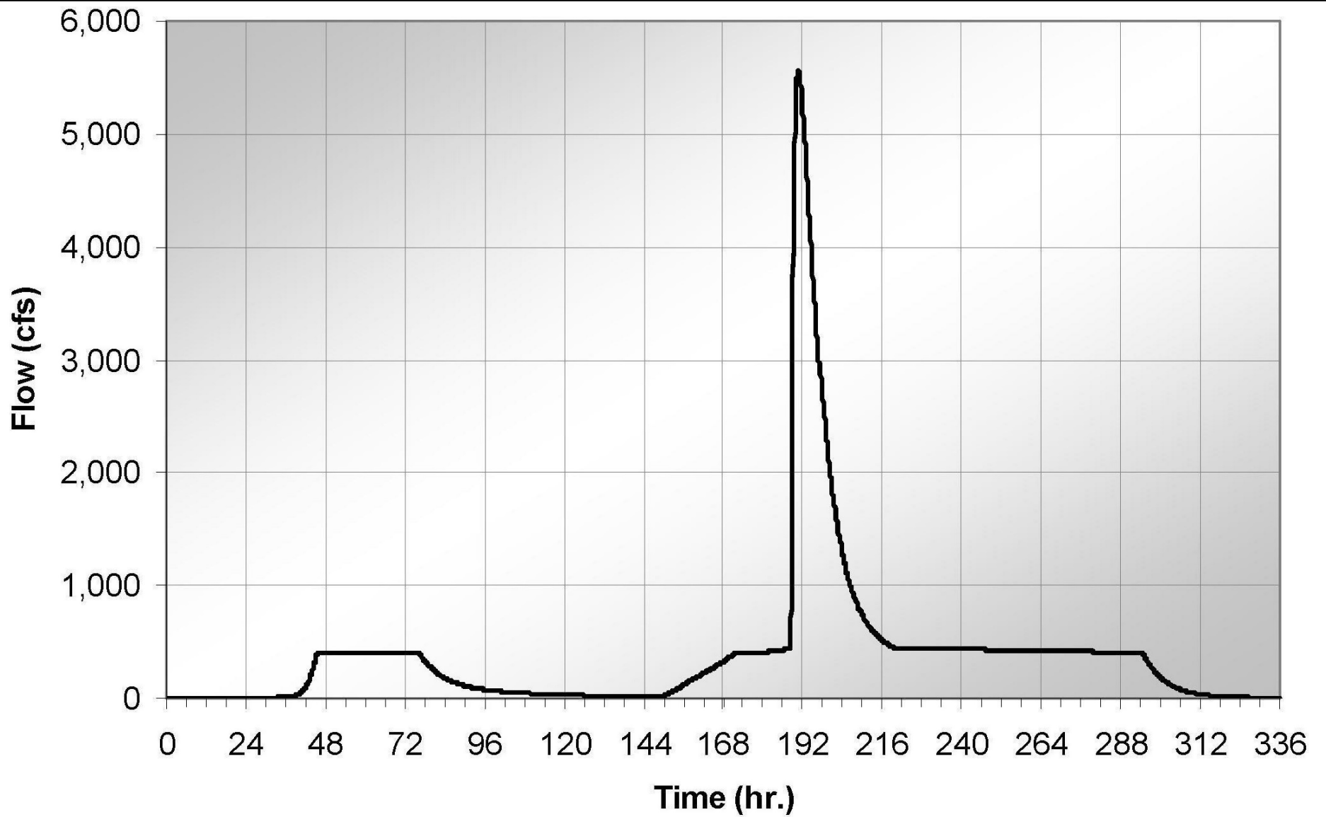
WILLIAM STATES LEE III NUCLEAR STATION UNITS 1 & 2 Subbasin Lake Wheelchel (WLCHL) PMF Inflow Hydrograph FIGURE 2.4.3-245 Rev 2
