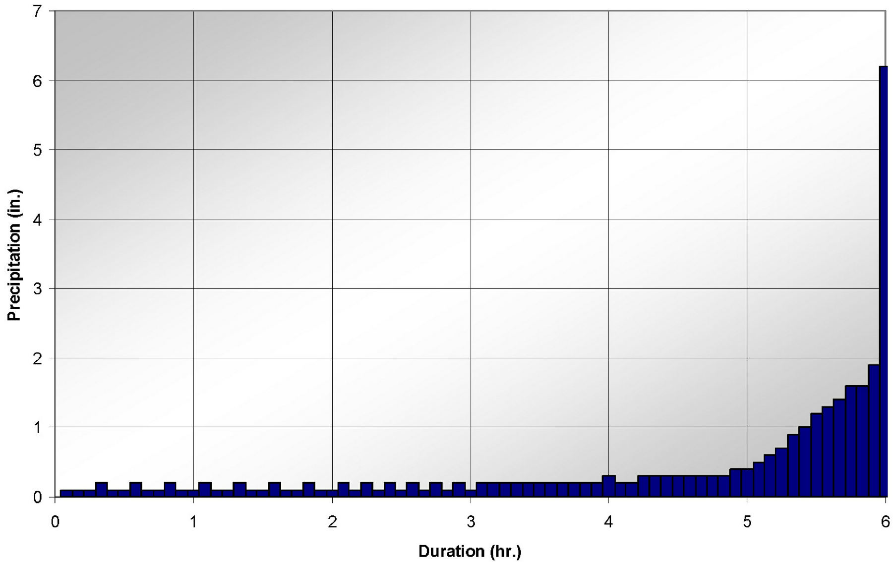
WILLIAM STATES LEE III NUCLEAR STATION UNITS 1 & 2 Local Intense Probable Maximum Precipitation 6-Hour End Peaking Hyetograph FIGURE 2.4.3-235 Rev 2
