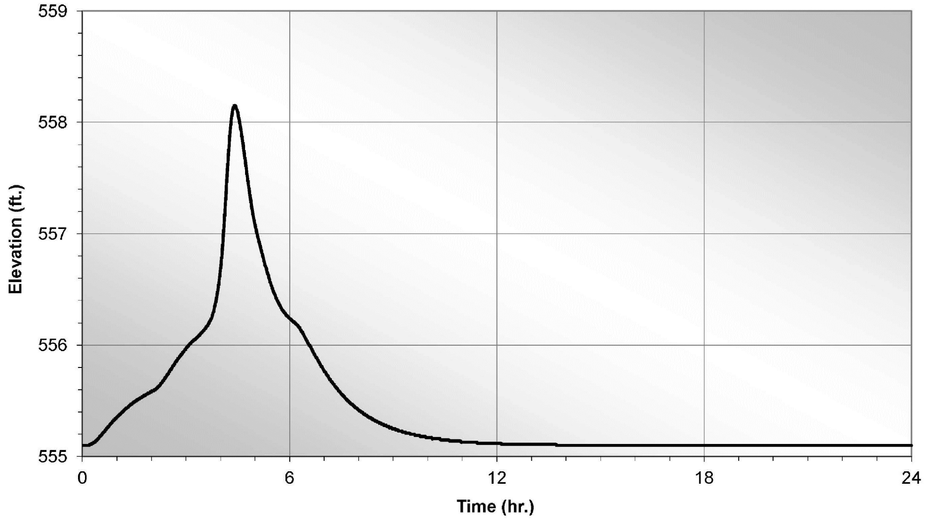
WILLIAM STATES LEE III NUCLEAR STATION UNITS 1 & 2 Flood Elevation Hydrograph Make-Up Pond A 6-Hour Local Intense Precipitation FIGURE 2.4.3-233 Rev 7
