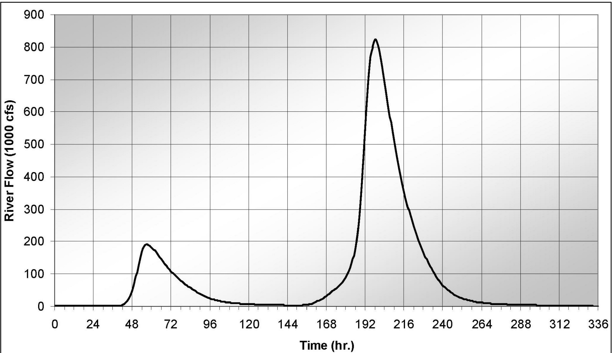
WILLIAM STATES LEE III NUCLEAR STATION UNITS 1 & 2 PMF Hydrograph, Broad River at Lee Nuclear Station FIGURE 2.4.3-226 Rev 2
