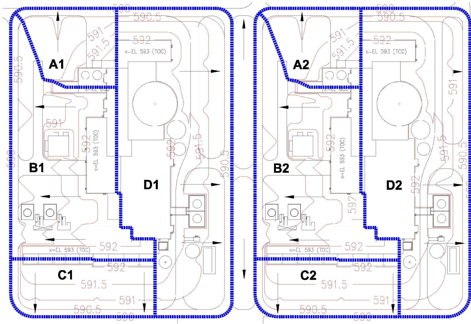
WILLIAM STATES LEE III NUCLEAR STATION UNITS 1 & 2 Site Analysis Drainage Areas FIGURE 2.4.2-204 Rev 7
