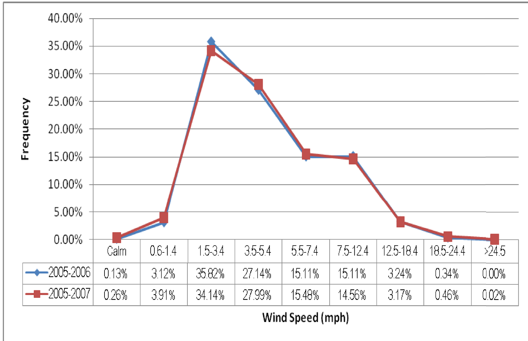
FIGURE 2CC-206 WIND SPEED FREQUENCY (10 M LEVEL)
