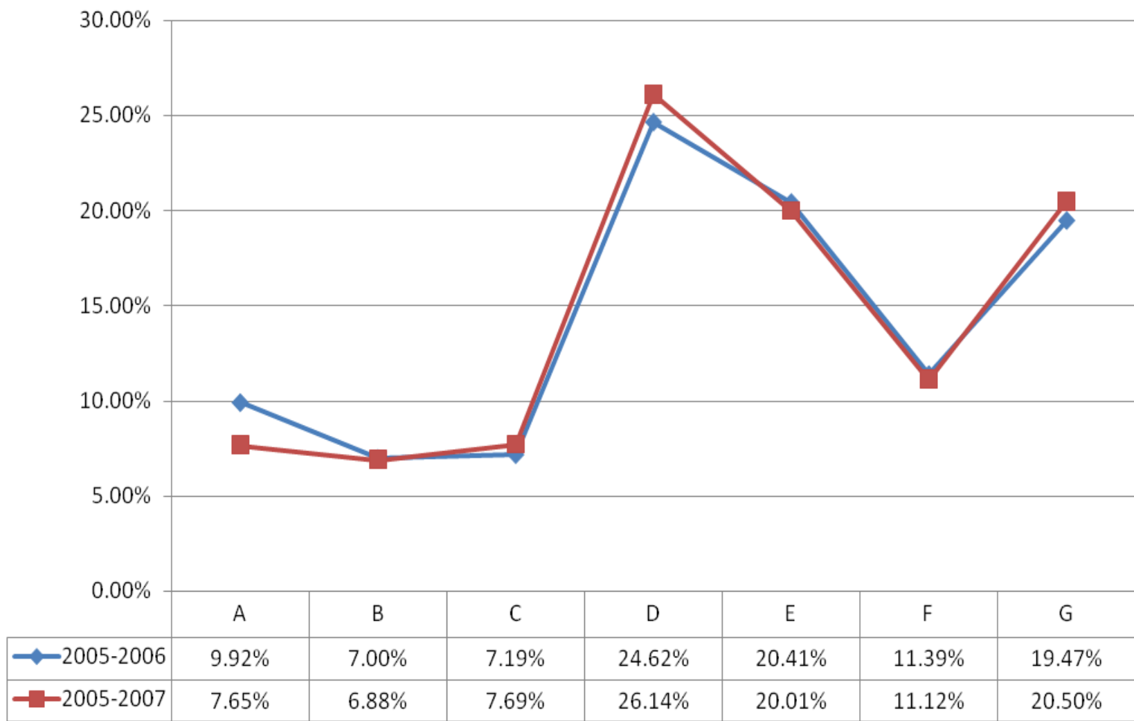
FIGURE 2CC-205 LEE NUCLEAR STATION STABILITY CLASS COMPARISON
