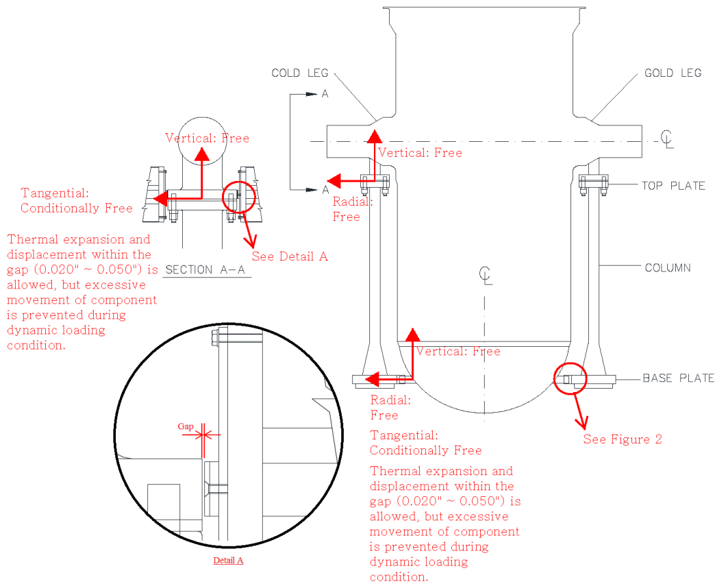
Figure 1 RV Support Assembly Detail (1/2)
