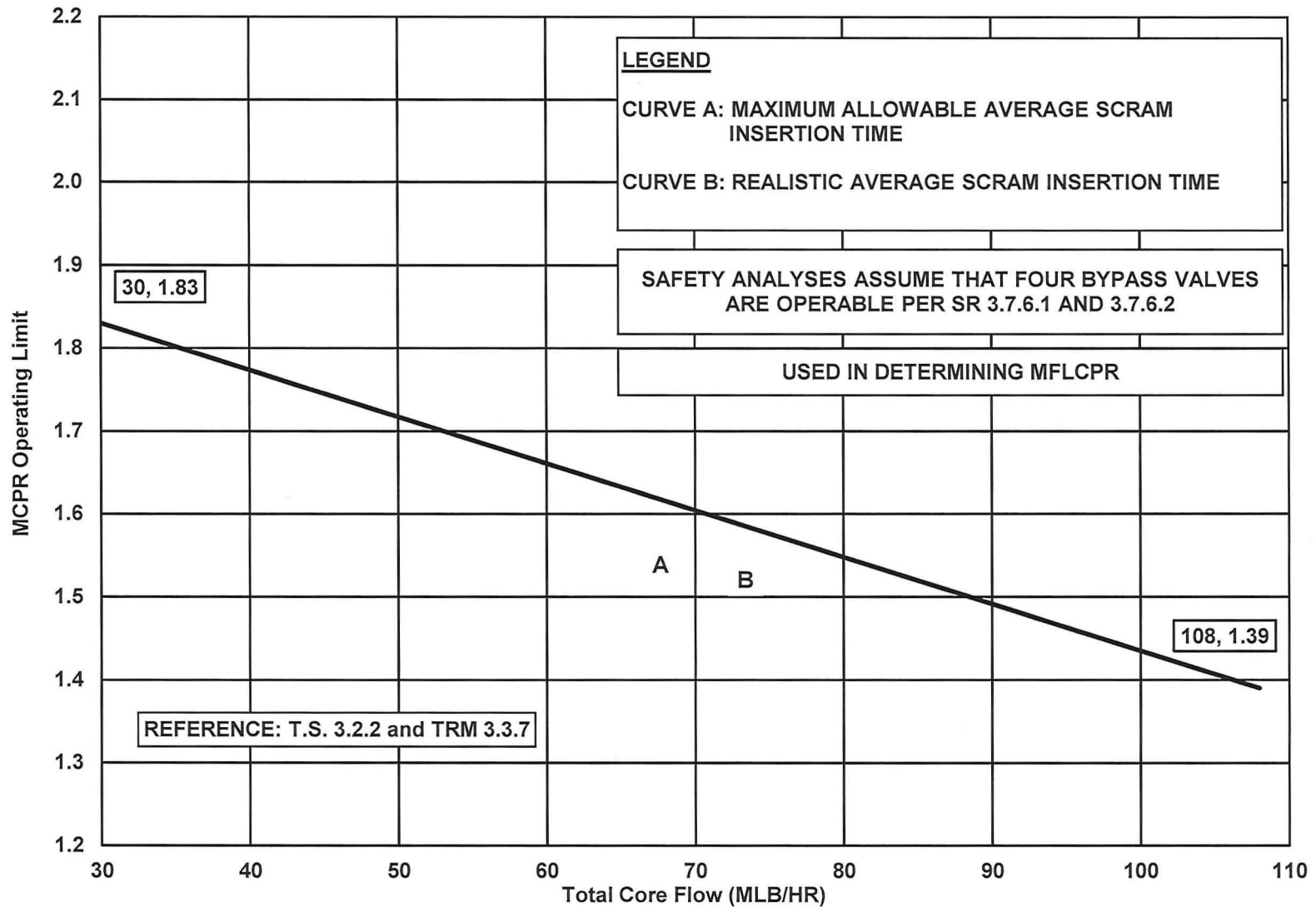
MCPR OPERATING LIMIT VERSUS TOTAL CORE FLOW ONE TSV OR TCV CLOSED* TWO LOOP OPERATION (BOC TO EOC)
