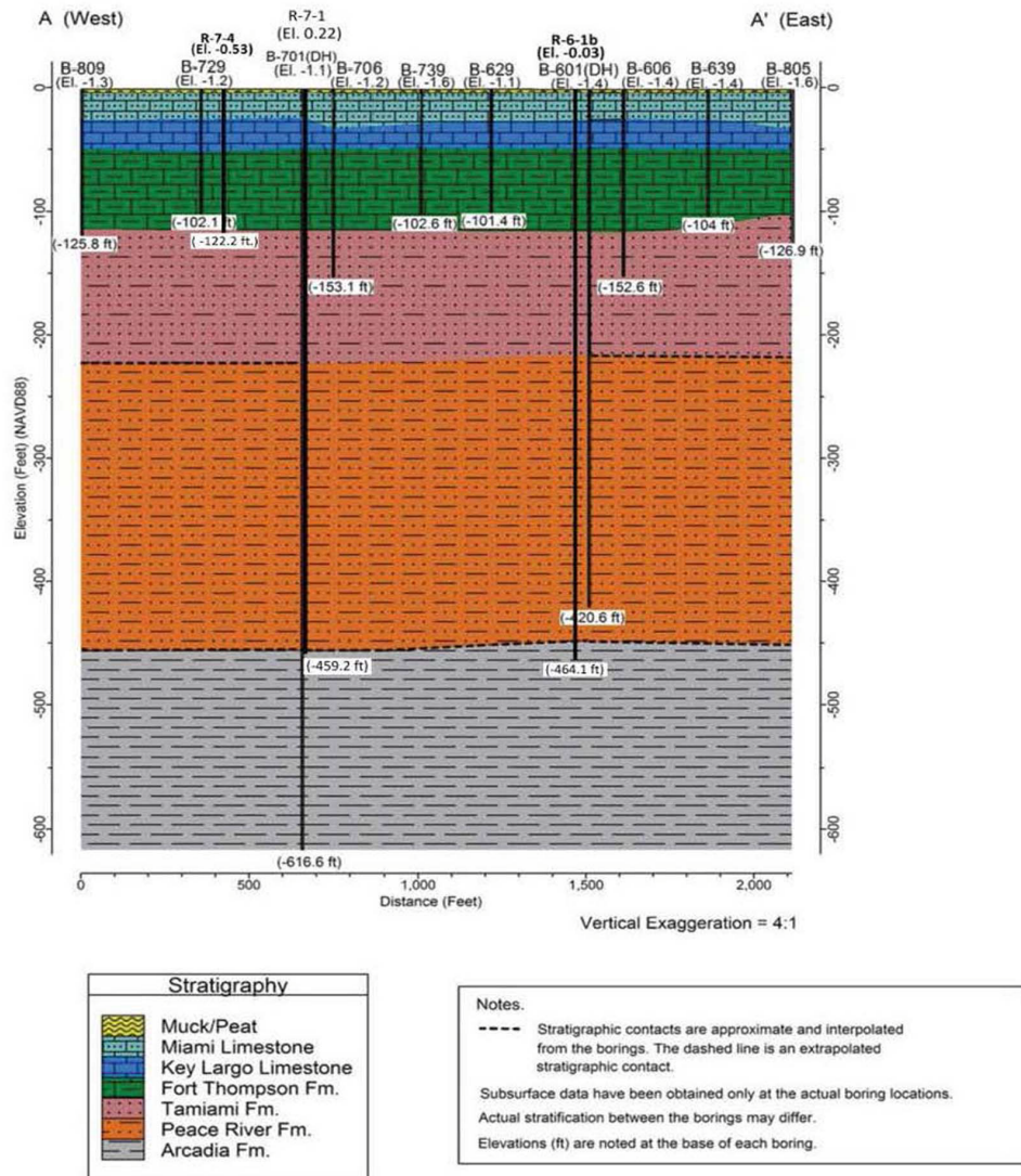
Figure 2.5AA-215 Cross-Section A-A' (Vertical Exaggeration = 4:1) This figure appears in FSAR Subsection 2.5.1 as Figure 2.5.1-386
