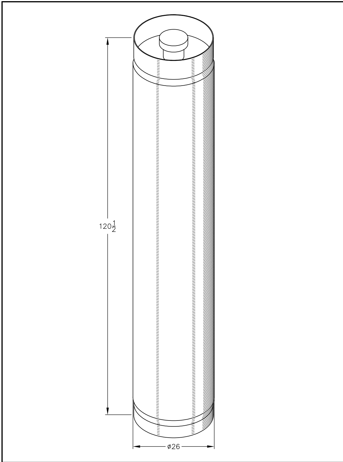
Figure 2.8-1 – RH-TRU Waste Canister
