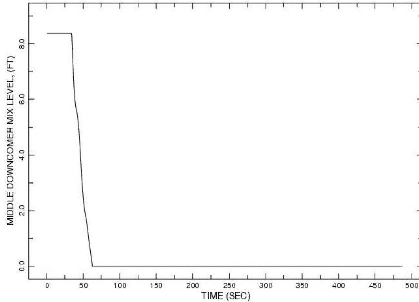
Figure 6.9 Limiting Recirculation Line Break Middle Downcomer Mixture Level
