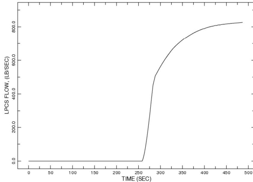
Figure 6.5 Limiting Recirculation Line Break LPCS Flow Rate
