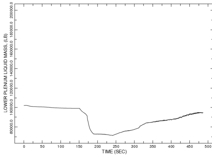
Figure 6.13 Limiting Recirculation Line Break Lower Plenum Liquid Mass
