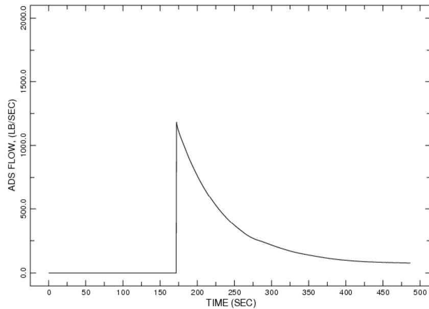
Figure 6.3 Limiting Recirculation Line Break ADS Flow Rate
