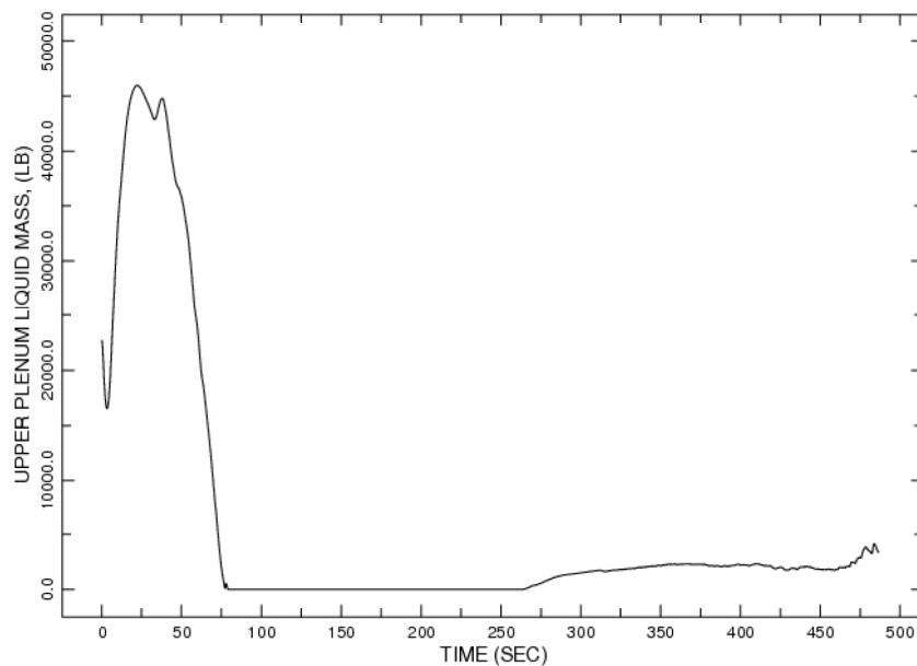
Figure 6.12 Limiting Recirculation Line Break Upper Plenum Liquid Mass
