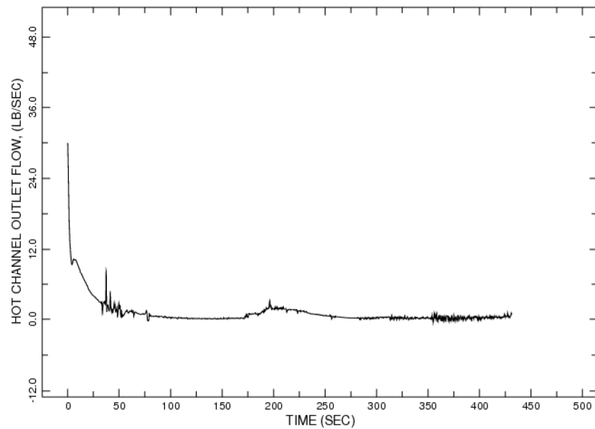
Figure 6.15 Limiting Recirculation Line Break Hot Channel Outlet Flow Rate
