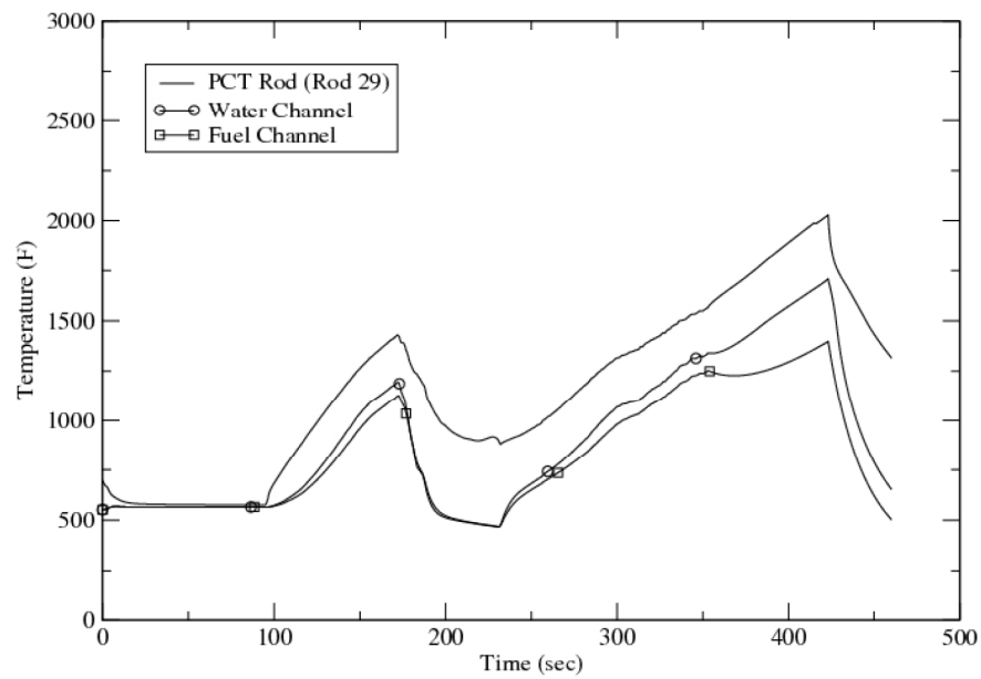
Figure 6.19 Limiting Recirculation Line Break Cladding Temperatures
