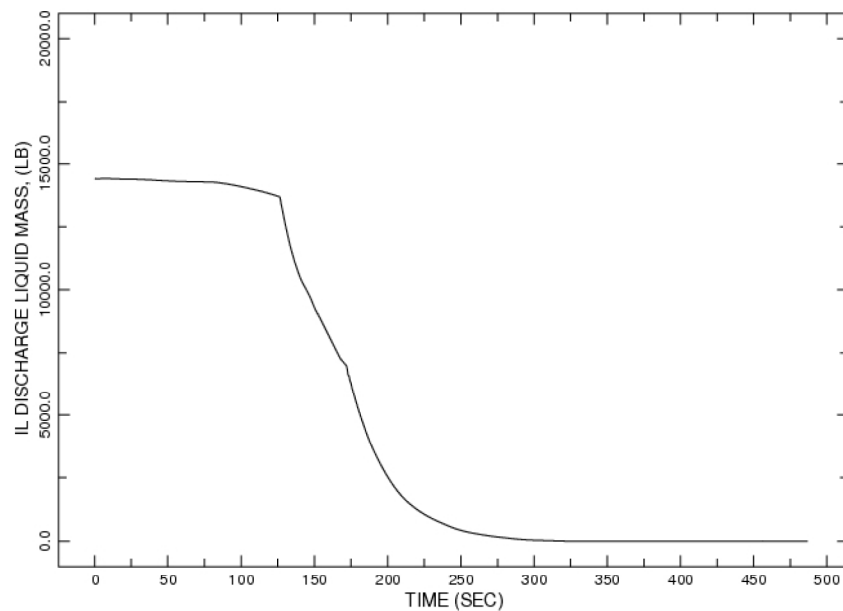
Figure 6.11 Limiting Recirculation Line Break Intact Loop Discharge Liquid Mass
