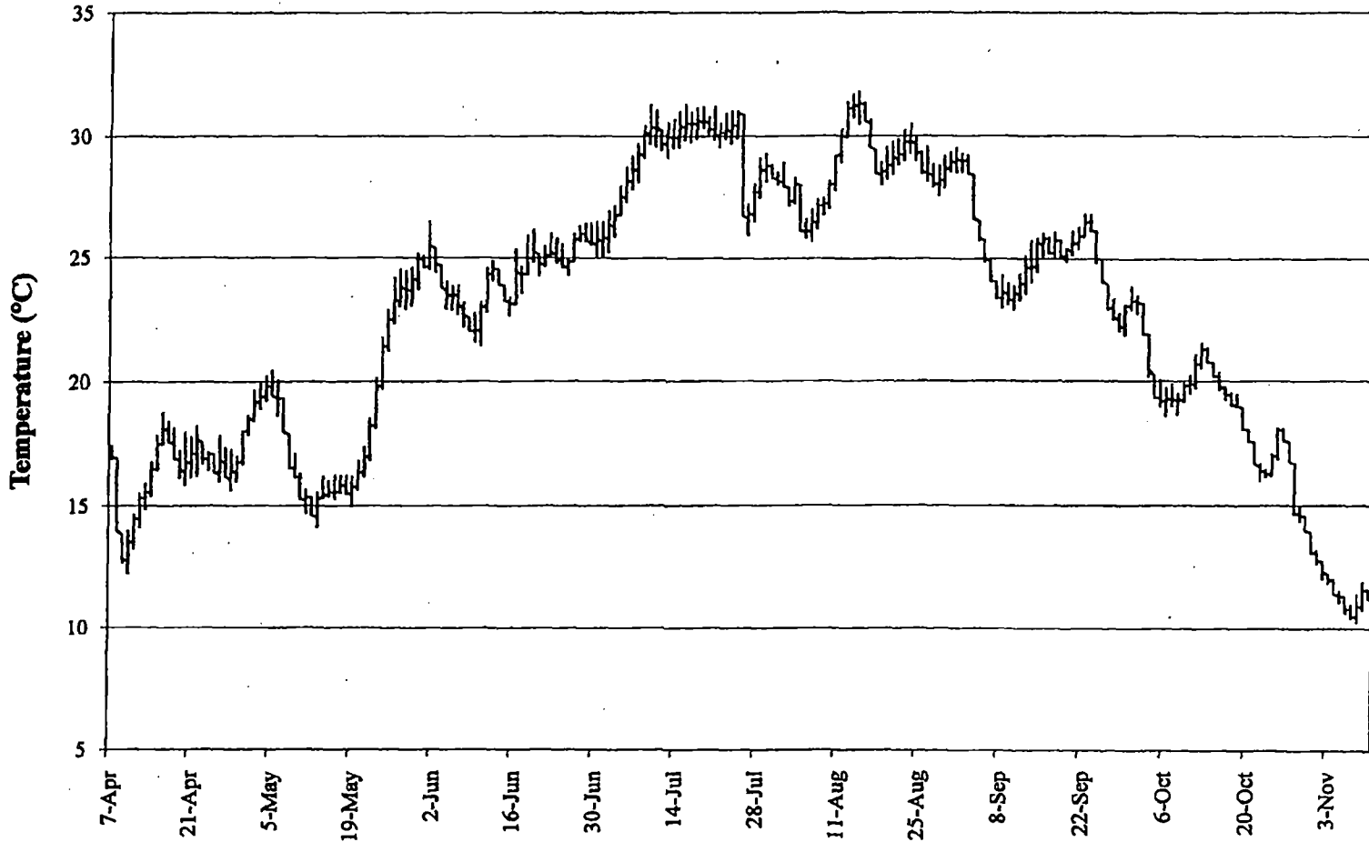
Figure 3-1. Temperature Profile at the LaSalle Station Intake for the Period of 7 April to 10 November, 2010.
