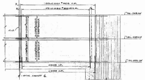
SECTION K-K (1)
