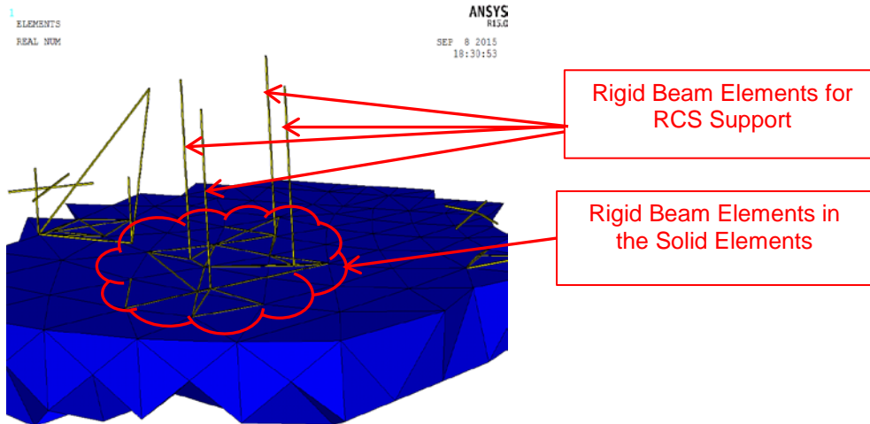
Figure 1. Connections between RCS Support and Solid Element
