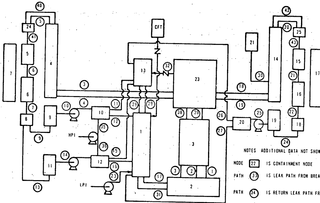
FIGURE 1 CRAFT2 NODING DIAGRAM FOR SMALL BREAKS
