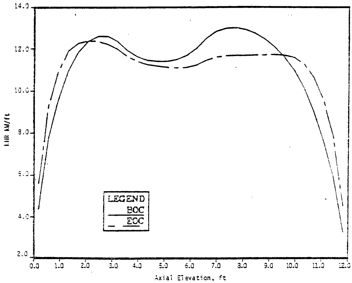
Figure 4-3. BOC and EOC Axial Power Shape Comparison
