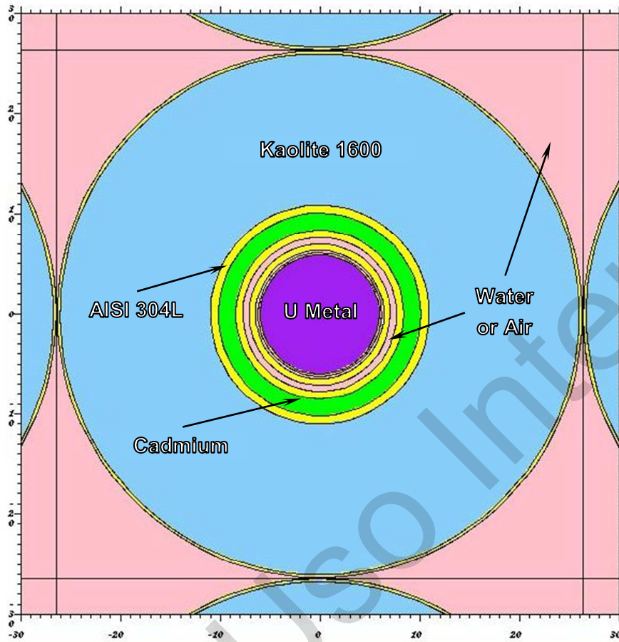
Picture 1: LEUPA horizontal section showing one of the packages in piling up
