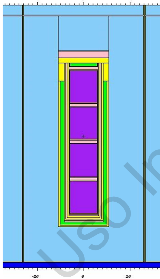
Picture 2: LEUPA vertical section showing one of the packages in piling up
