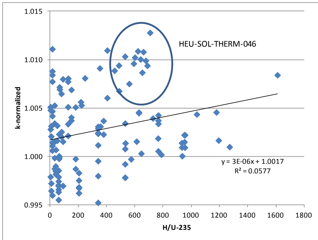
Figure 2 - H/^{235}U Trend
