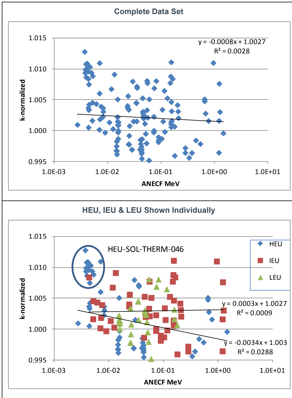
Figure 1 - ANECF Trend
