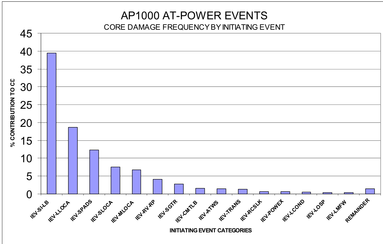
Figure 19.59-1 Contribution of Initiating Events to Core Damage
