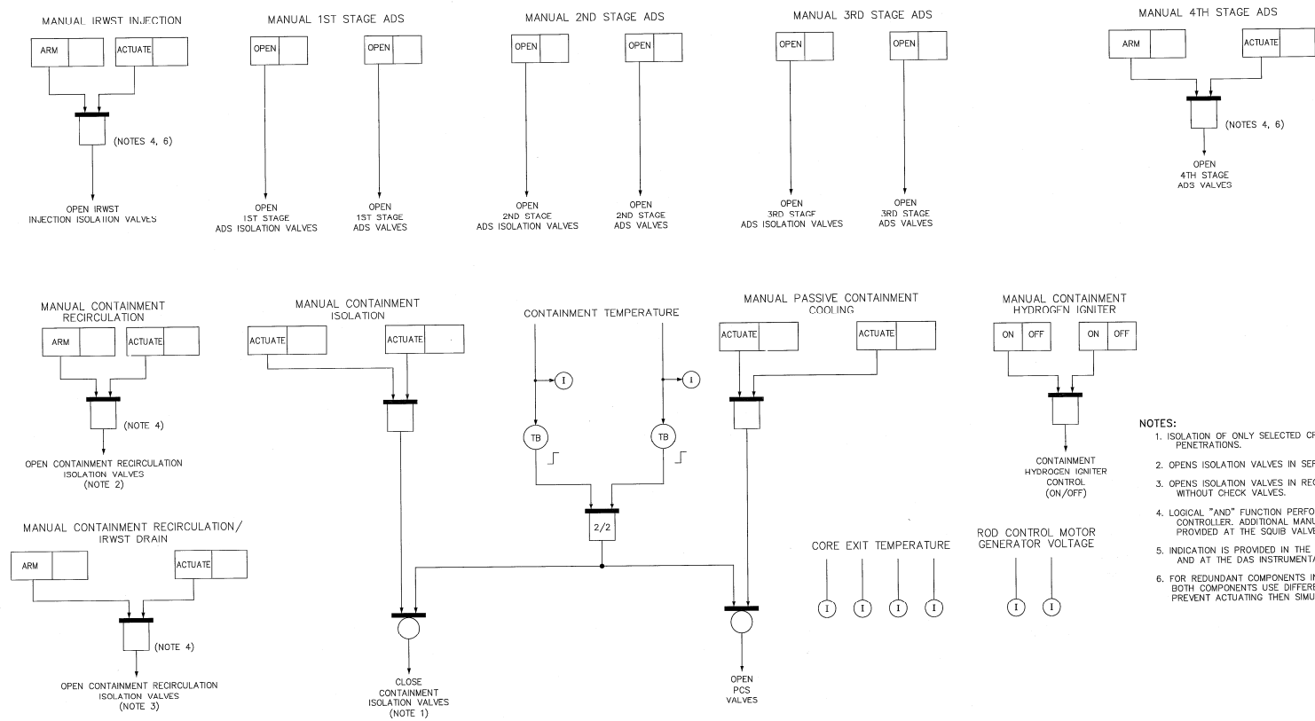
Figure 7.2-1 (Sheet 21 of 21) Functional Diagram Diverse Actuation System Logic, Manual Actuations
