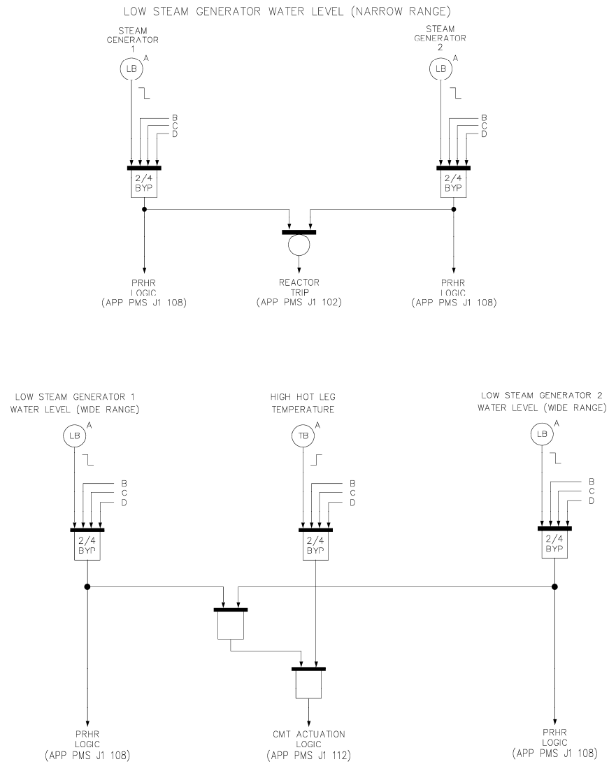
Figure 7.2-1 (Sheet 7 of 21) Functional Diagram Loss of Heat Sink Protection
