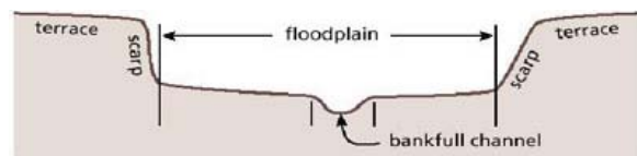
B. Incised Stream (early widening phase)
