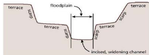
C. Incised Stream (widening phase complete)
