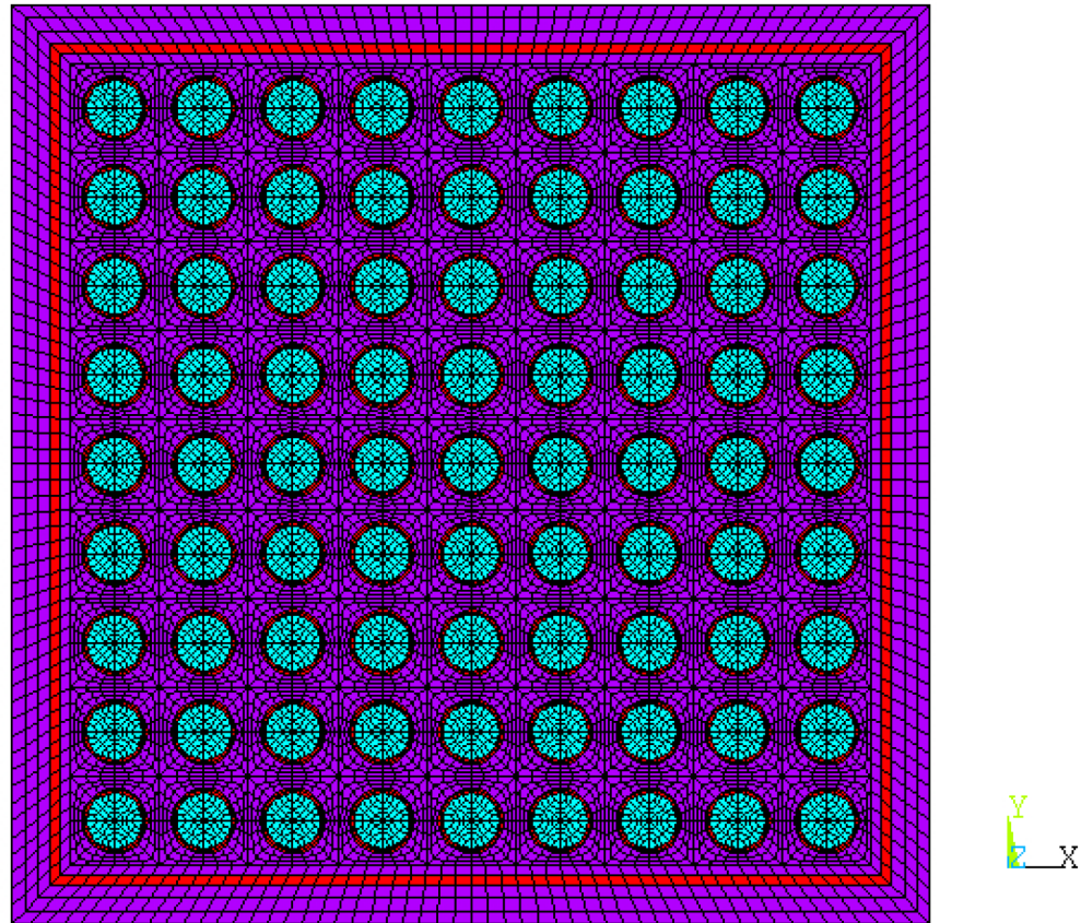
Figure 4.9.1-3 Finite Element Model of the FANP 9x9 Fuel Assembly
