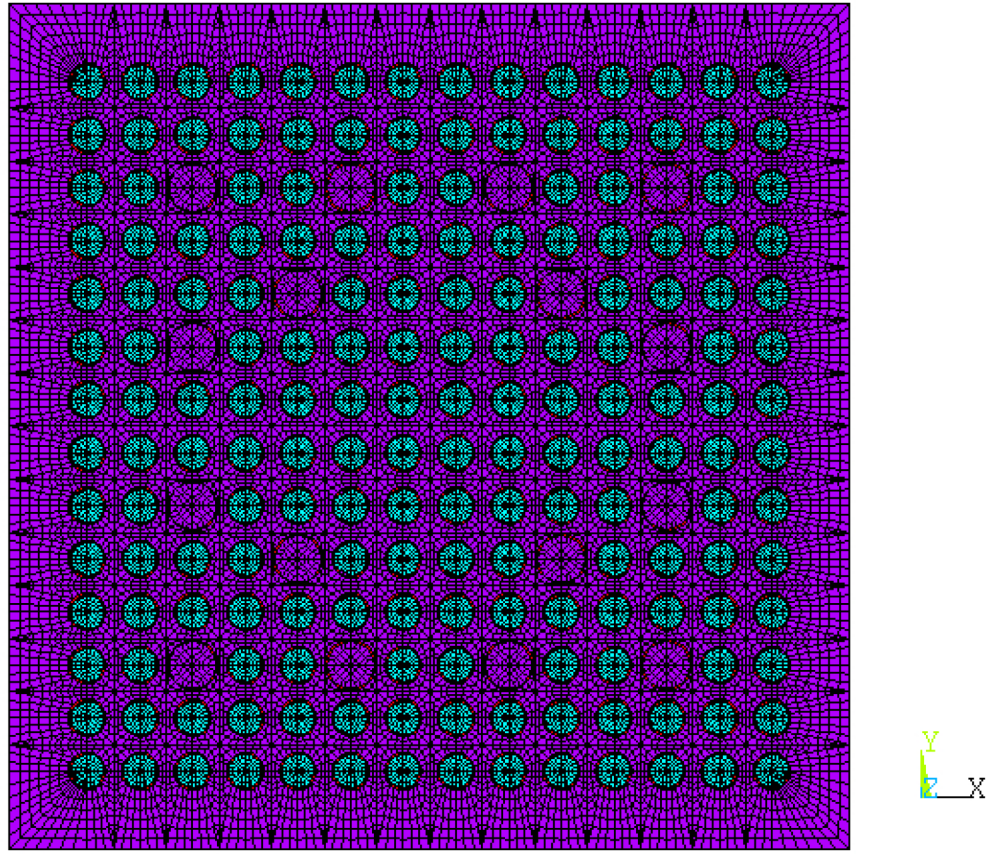
Figure 4.9.1-1 Finite Element Model of WE14x14 Fuel Assembly
