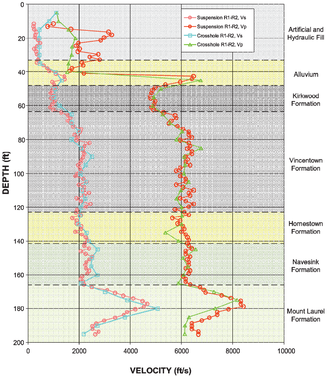
PSEG Power, LLC PSEG SITE ESPA Part 2, Site Safety Analysis Report P- and S-Wave Comparison for Crosshole and P-S suspension Techniques, NB-8 FIGURE 2.5.4.4-7 Rev 0
