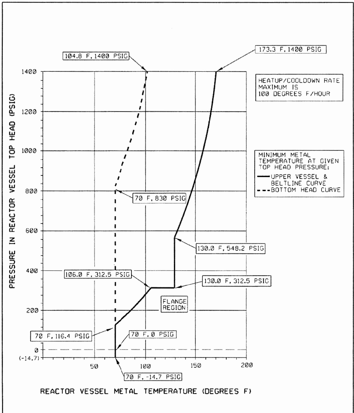
FIGURE 3.4.11-1(b): NON-NUCLEAR HEATUP/COOLDOWN CURVES (VALID UP TO 32 EFPY)
