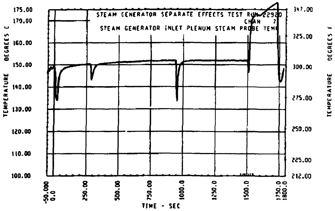
Figure 5: R22920 Primary Side Inlet Temperature
