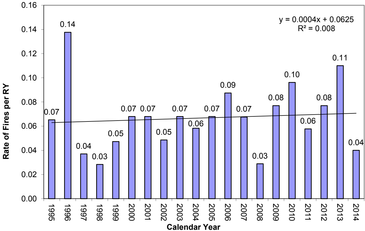
Figure 2: Number of Significant Fires Reported per Reactor Year 1995-2014
