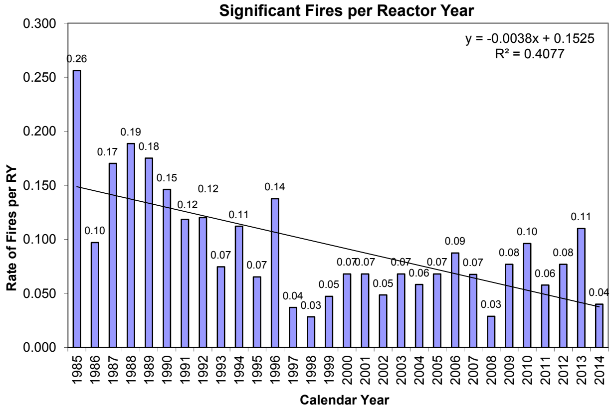
Figure 3: Number of Significant Fires Reported per Reactor Year 1985-2014
