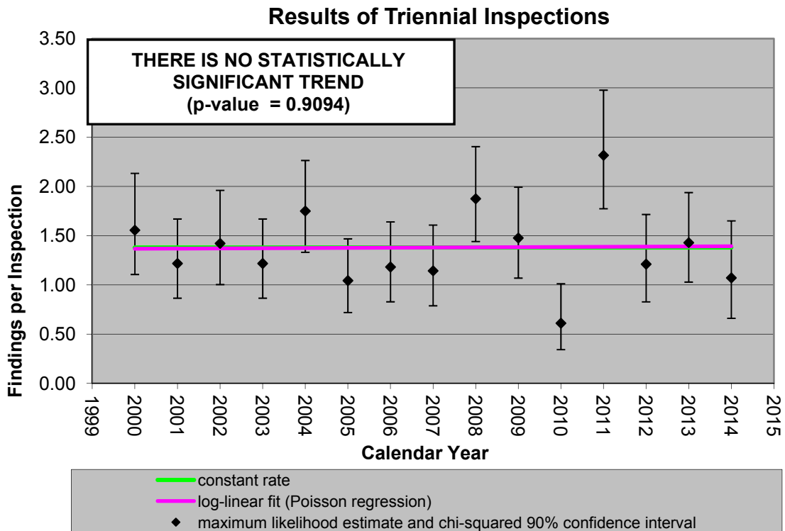
Figure 6: Trend analysis of findings made during triennial fire protection inspections for the period 2000-2014.
