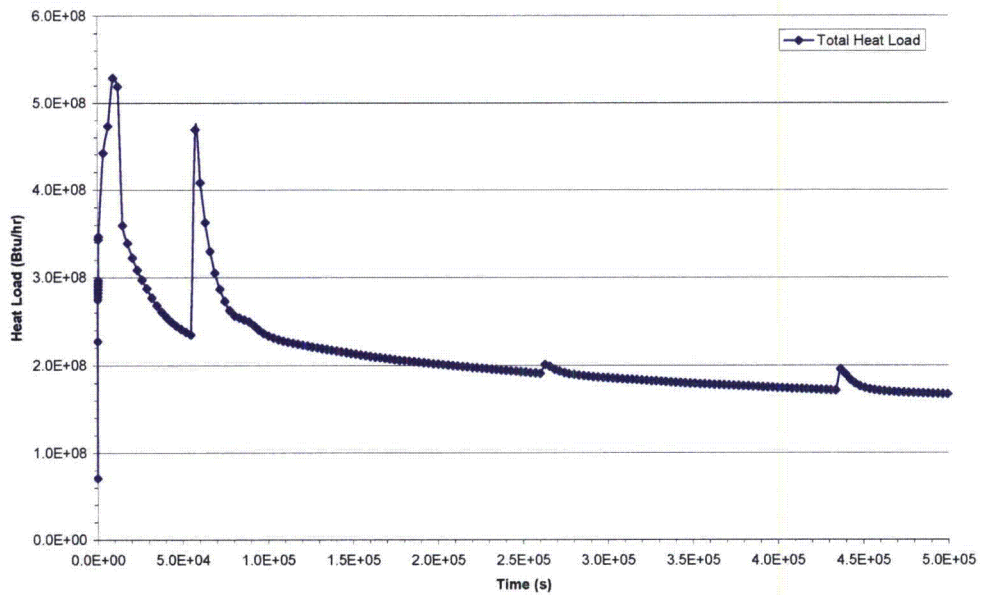
Fig. D6-3: Total Heat Loads to UHS
