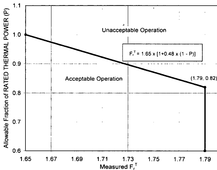
FIGURE 3.2-3 Allowable Combinations of THERMAL POWER and F_r^T
