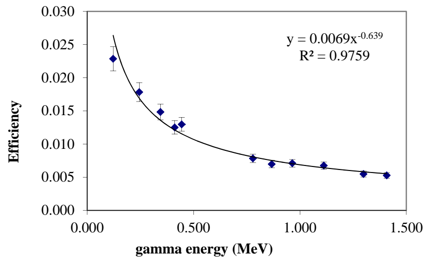
Figure C3: HPGGe6 Efficiency curve used for analysis of samples from FY13Q2 and FY13Q3 sampling intervals determined from counting 45mL of a 152 Eu standard in a 50mL conical centrifuge tube.
