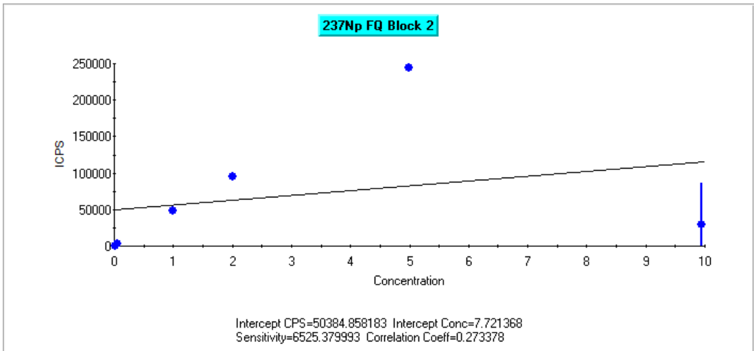
Figure D2: Screen capture of the 237 Np calibration curve using Thermo Plasma Lab software to control the data collection and analysis for the FY13Q1 sampling interval. R^2=0.27338 , Intercept Conc. (Detection Limit) = 7.7214 ppb.
