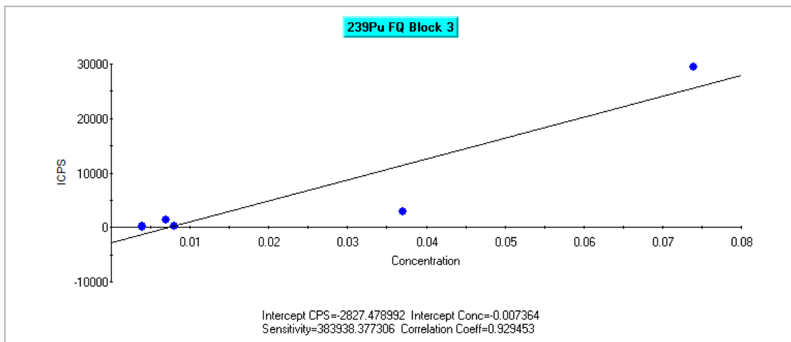
Figure D3: Screen capture of the 239 Pu calibration curve using Thermo Plasma Lab software to control the data collection and analysis for the FY13Q1 sampling interval. R^2=0.92945 , Intercept Conc. (Detection Limit) = 0.00736 ppb.
