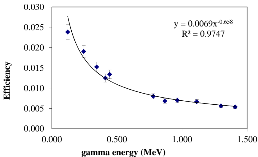
Figure 2: HPGe Efficiency curve determined from counting 45mL of a 152 Eu standard in a 50mL conical centrifuge tube.
