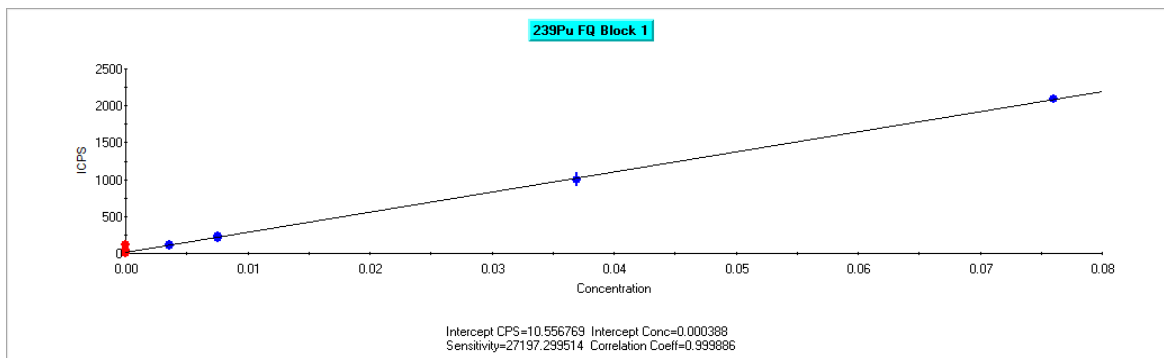
Figure 4: Screen capture of the ^{239}\text{Pu} calibration curve using Thermo Plasma Lab software to control the data collection and analysis for the FY13Q3 sampling interval. R^2=0.99989 , Intercept Conc. (Detection Limit) = 0.0004 ppb.
