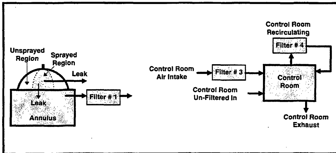
Figure 8. Advanced PWR Control Room Detail
