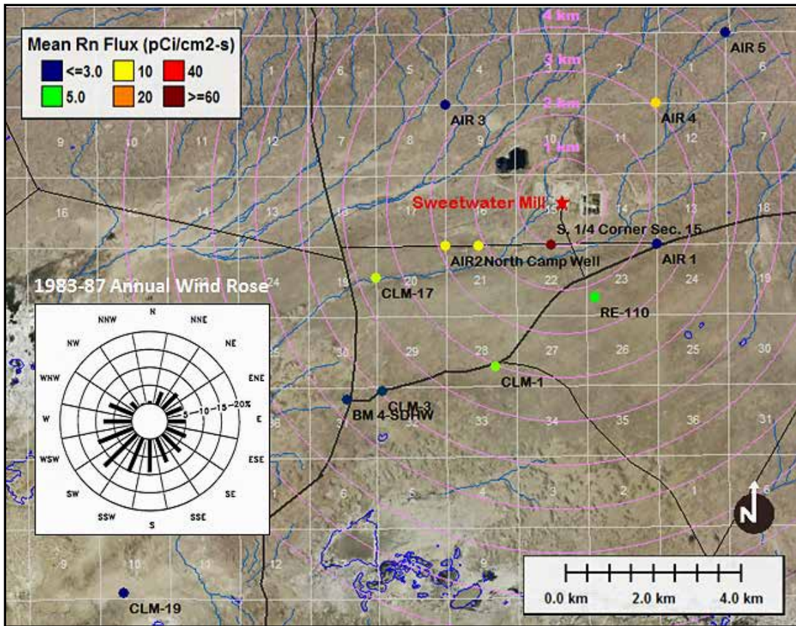
Figure 2.10-7: Average Rn-222 radon flux rates (pCi/cm 2 /second) at the soil surface in the vicinity of the Sweetwater Mill site based on Method 115 flux measurements. Mean values are represented by interpolated color blends based on the range of discrete color assignments shown in the legend.
