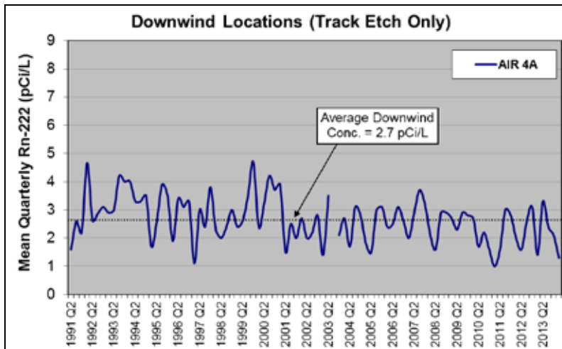
Figure 2.10-5: Average long-term quarterly Rn-222 concentrations at the downwind monitoring location.
