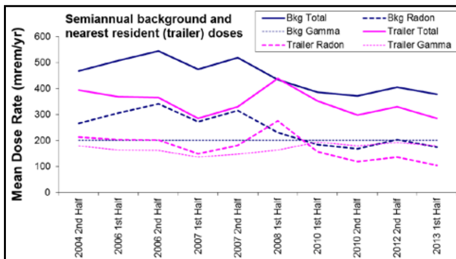
Figure 2.12-5: Reported total annual background dose rates and dose rates to the nearest member of the public (security trailer occupant), along with dose from major pathway components (radon and gamma radiation), since the 2004 license renewal.
