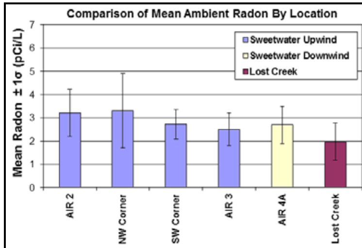
Figure 2.10-6: Average long-term quarterly Rn-226 concentrations and standard deviations ( \pm 1\sigma ) at individual Sweetwater Mill site locations, compared with an overall average baseline concentration at the nearby Lost Creek ISR site.
