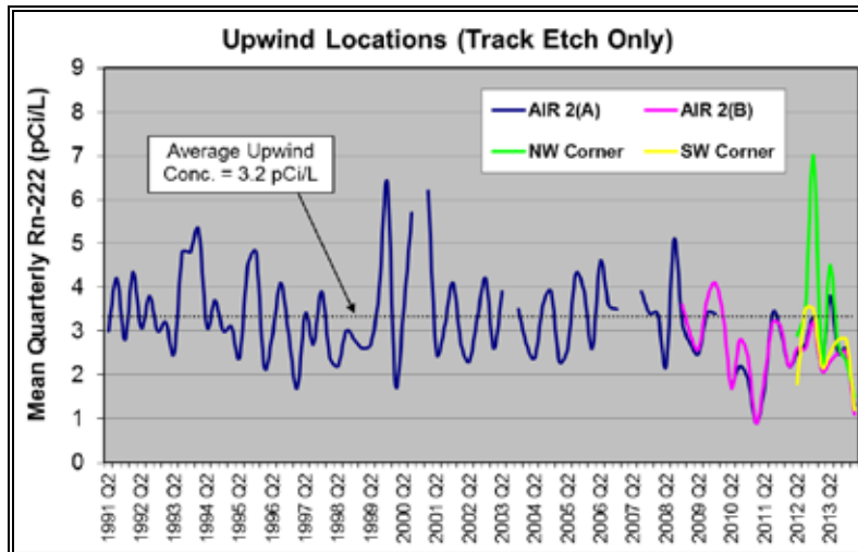
Figure 2.10-4: Average long-term quarterly Rn-222 concentrations at upwind monitoring locations.
