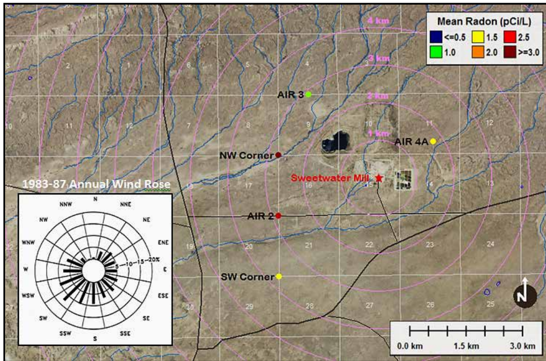
Figure 2.10-3: Average long-term quarterly Rn-226 concentrations in the vicinity of the Sweetwater Mill site based on track-etch radon detector monitoring. Mean values are represented by interpolated color blends based on the range of discrete color assignments shown in the legend.
