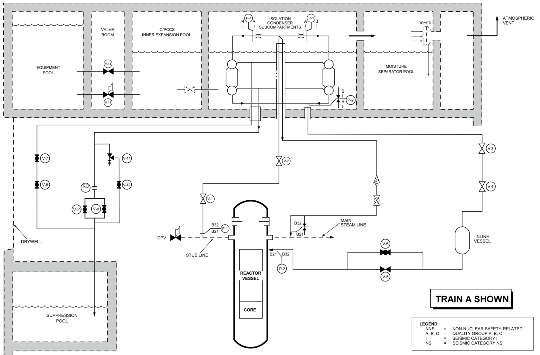
Figure 2.4.1-1. Isolation Condenser System Schematic
