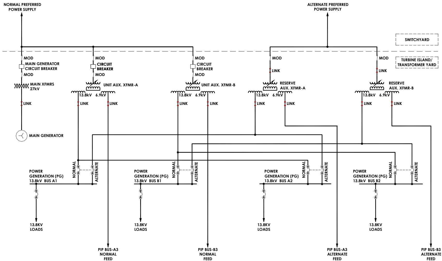
Figure 2.13.1-1 Sh 1. Electric Power Distribution System Functional Arrangement
