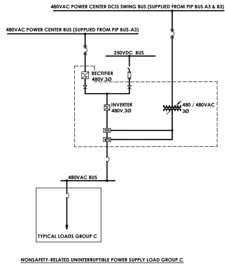
Figure 2.13.5-2. Sh 1. Nonsafety-Related UPS System Functional Arrangement
