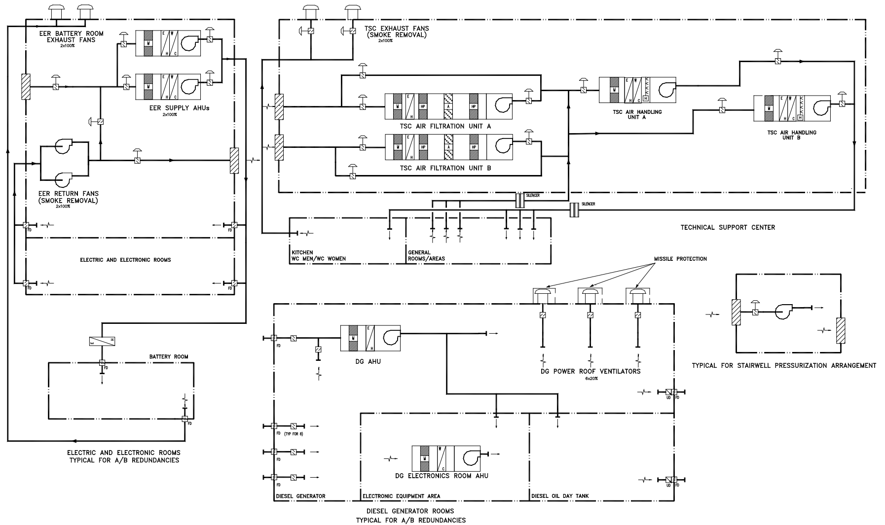
Figure 2.16.2-9. EBVS Functional Arrangement Diagram
