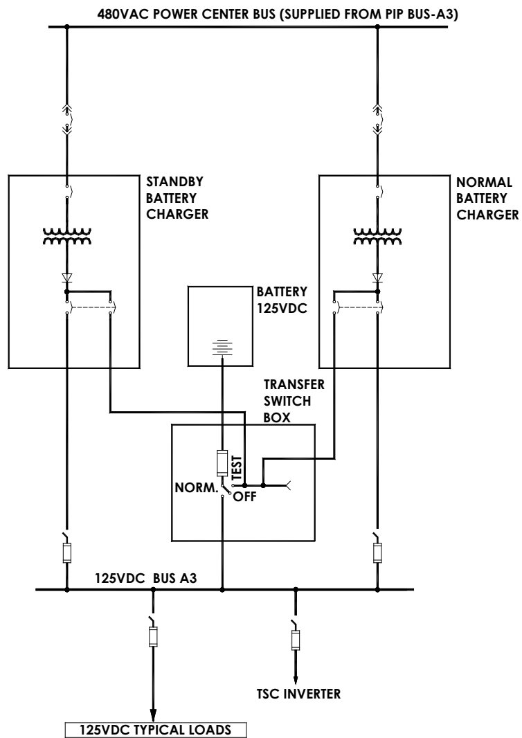
NONSAFETY-RELATED 125VDC SYSTEM
