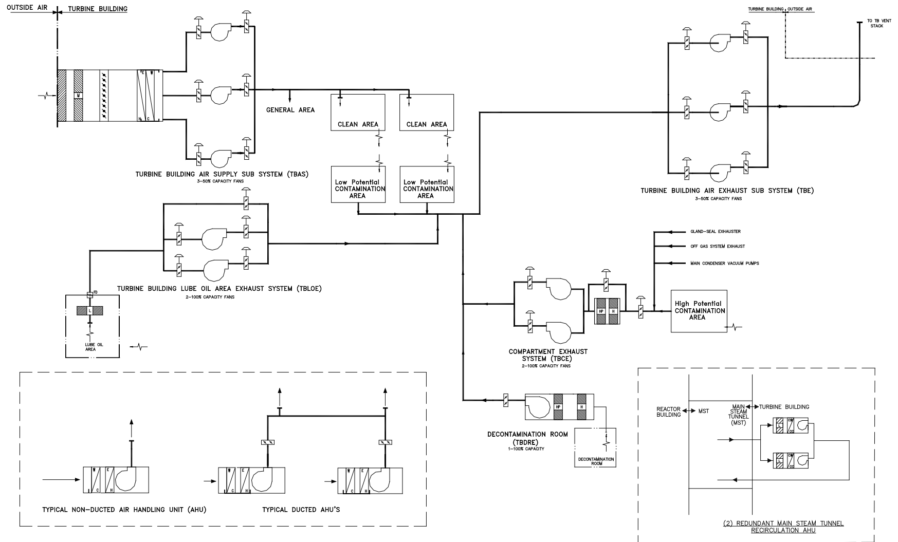
Figure 2.16.2-6. TBVS Functional Arrangement Diagram
