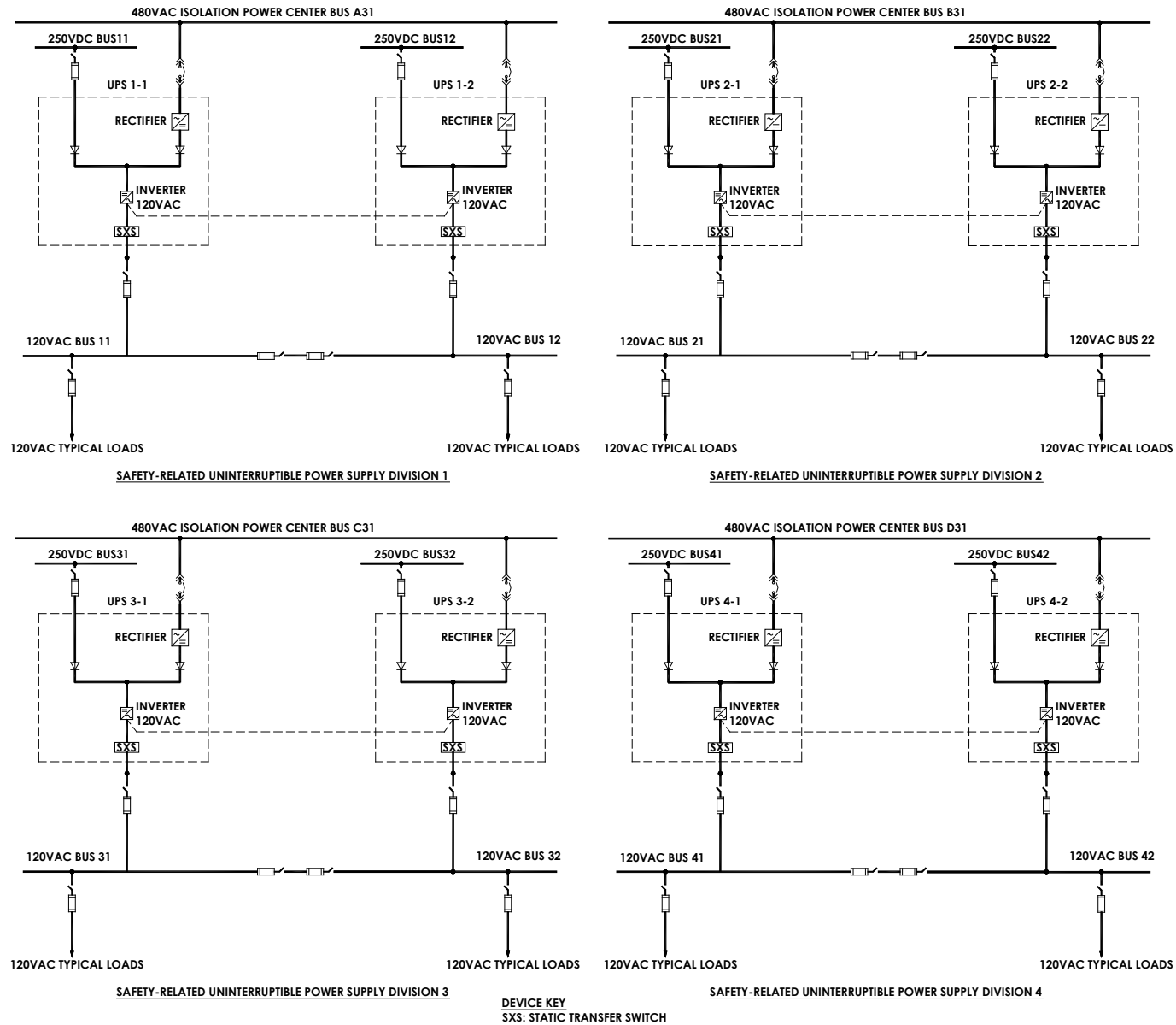
Figure 2.13.5-1. Safety-Related UPS System Functional Arrangement
