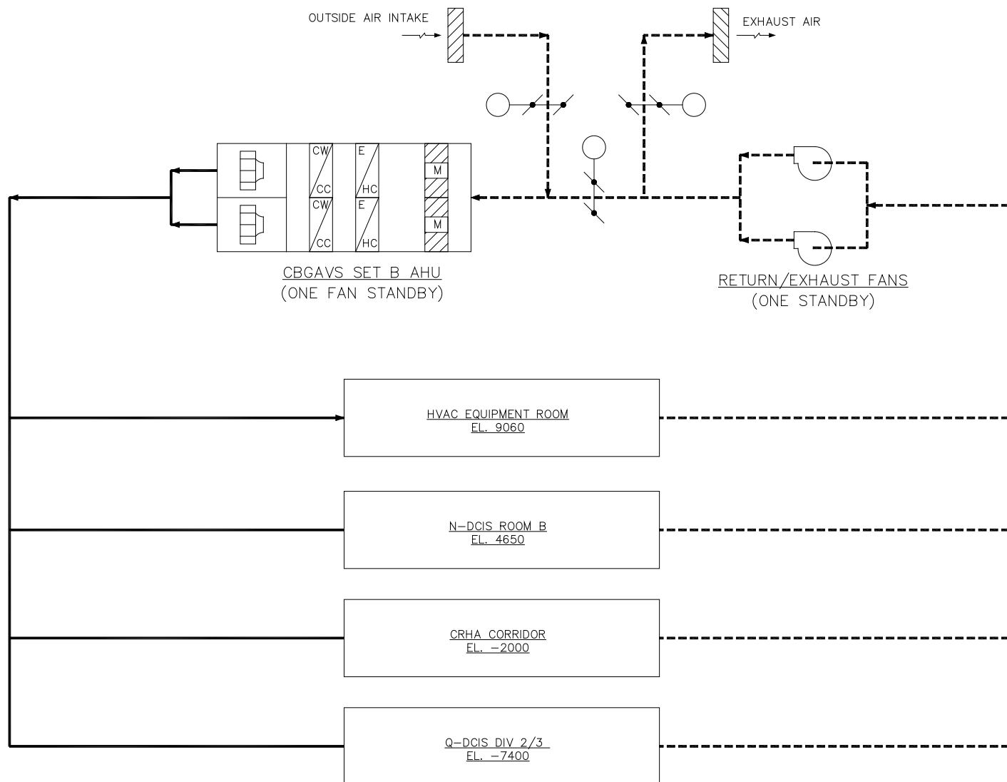
Figure 2.16.2-5b. CBGAVS (Set B) Functional Arrangement Diagram
