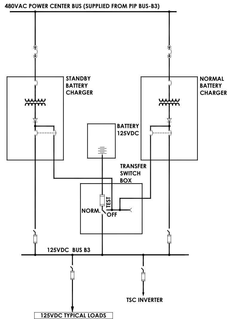
Figure 2.13.3-2 Sh 2. Nonsafety-Related 125 VDC System Functional Arrangement
