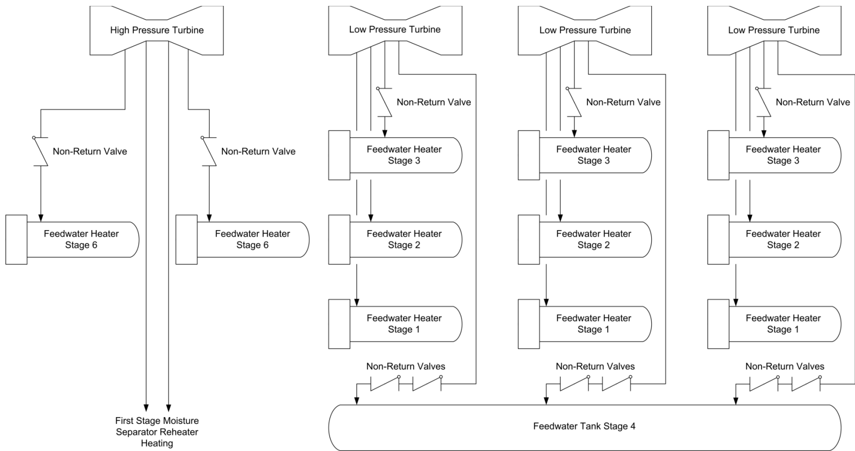
Figure 2.11.1-3. Extraction Steam Functional Arrangement
