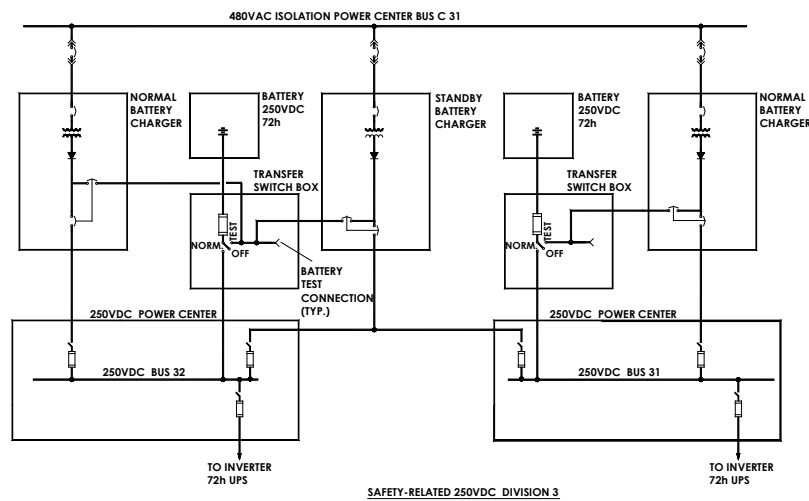
Figure 2.13.3-1. Safety-Related 250 VDC System Functional Arrangement
