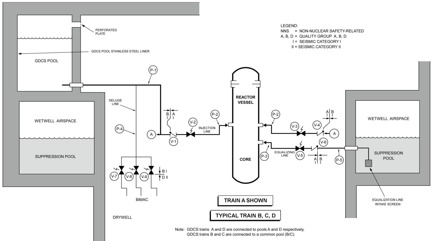
Figure 2.4.2-1. Gravity-Driven Cooling System
