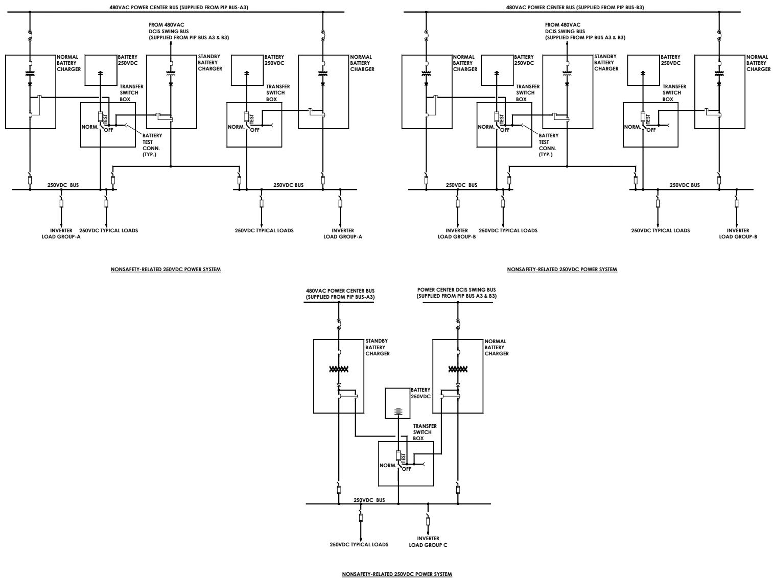
Figure 2.13.3-2 Sh 1. Nonsafety-Related 250 VDC System Functional Arrangement
