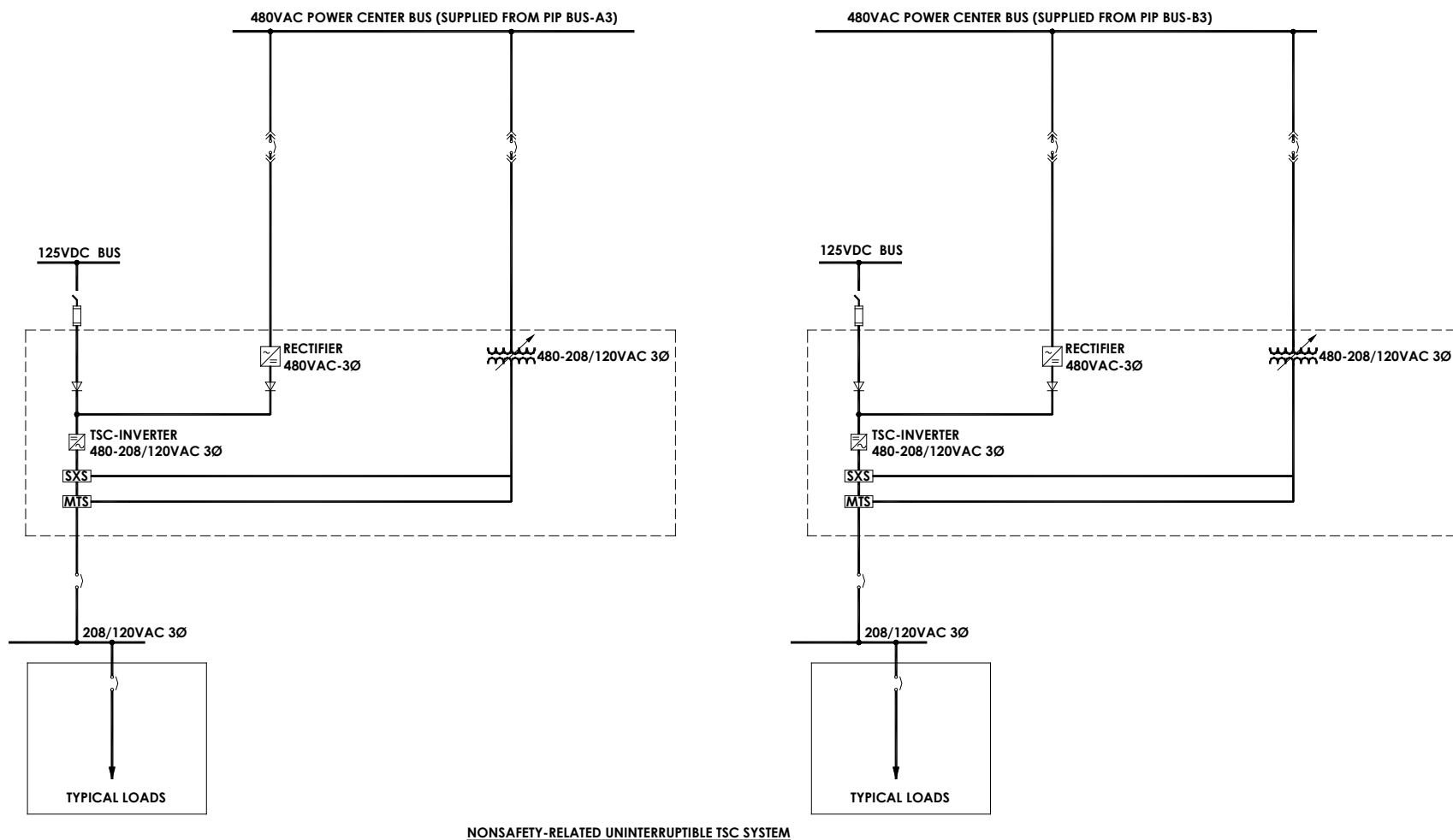
Figure 2.13.5-2 Sh 2 Nonsafety-Related UPS System Functional Arrangement
