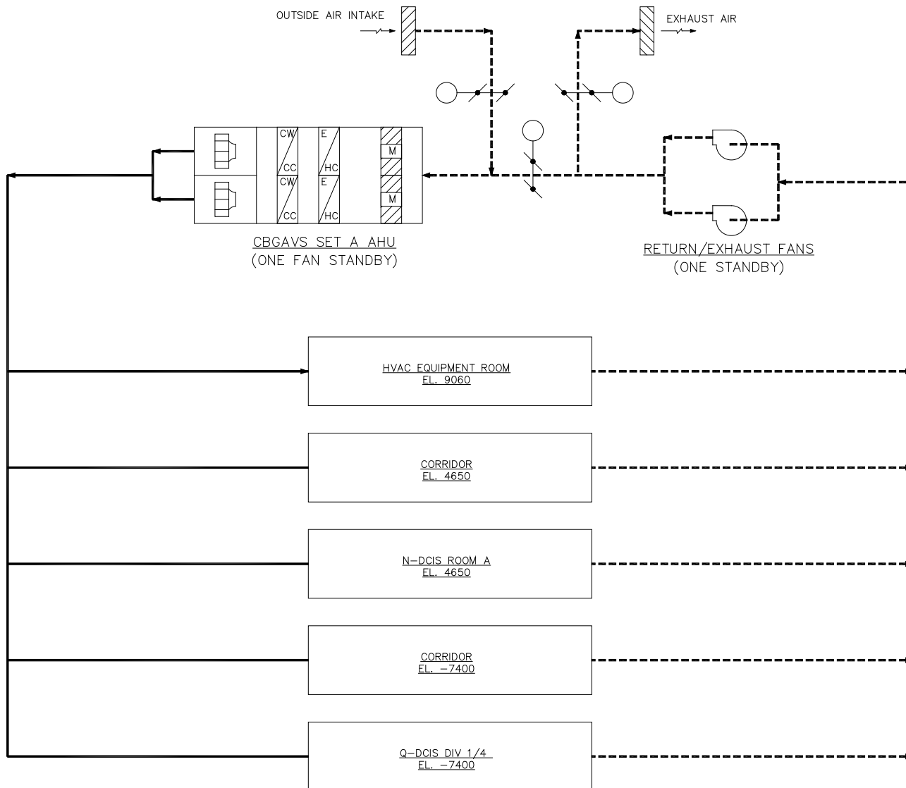
Figure 2.16.2-5a. CBGAVS (Set A) Functional Arrangement Diagram
