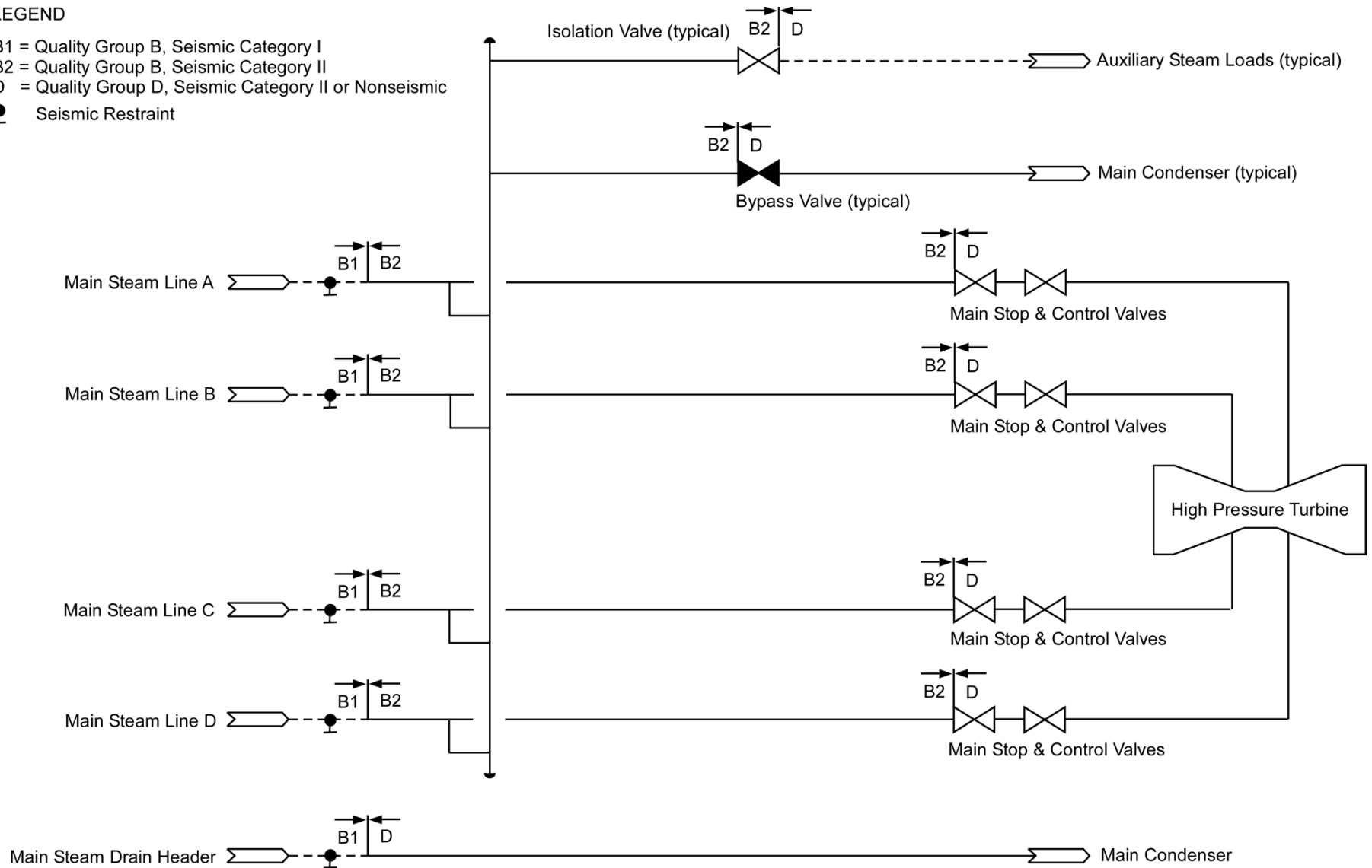
Figure 2.11.1-1. TMSS Functional Arrangement
