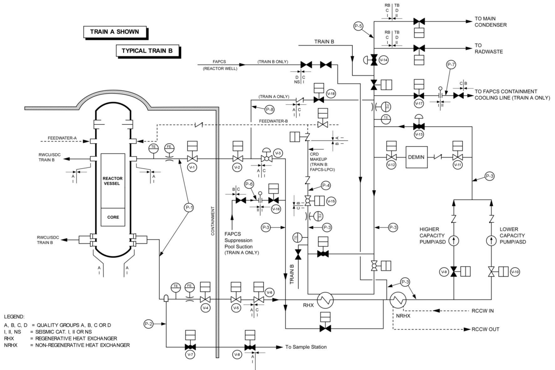
Figure 2.6.1-1. Reactor Water Cleanup/Shutdown Cooling System
