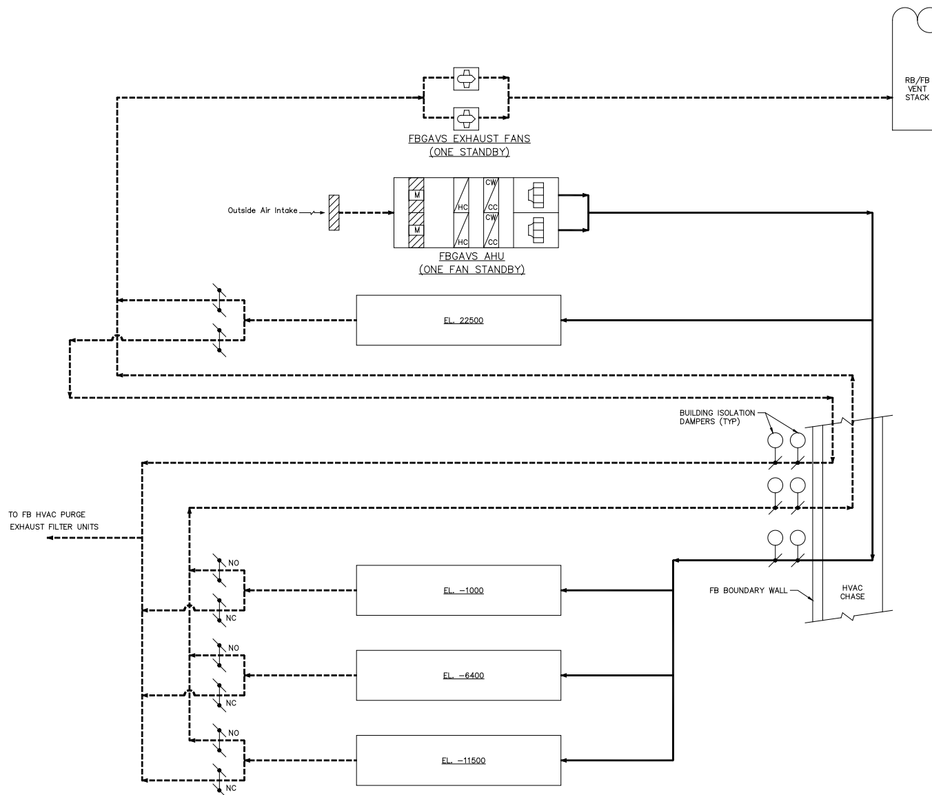
Figure 2.16.2-7. FBGAVS Functional Arrangement Diagram
