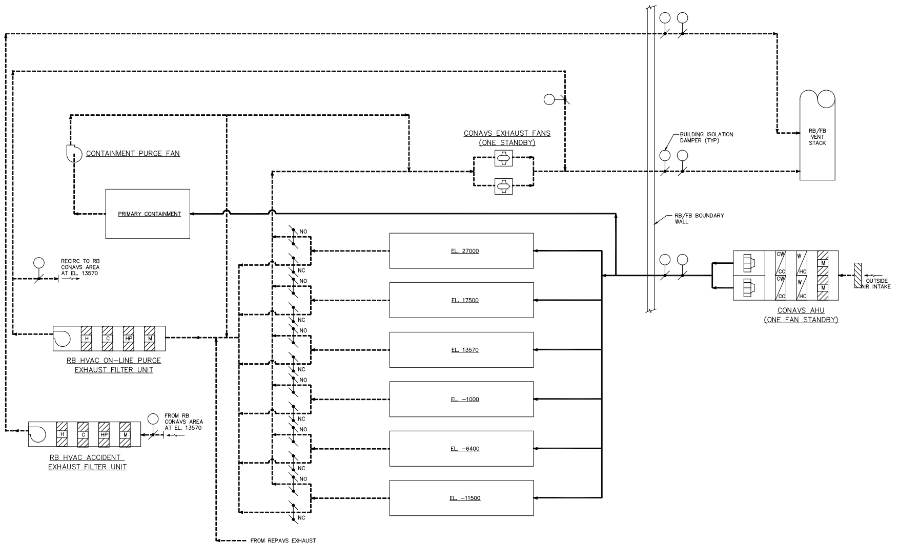
Figure 2.16.2-2. CONAVS Functional Arrangement Diagram (Typical Train A/B)
