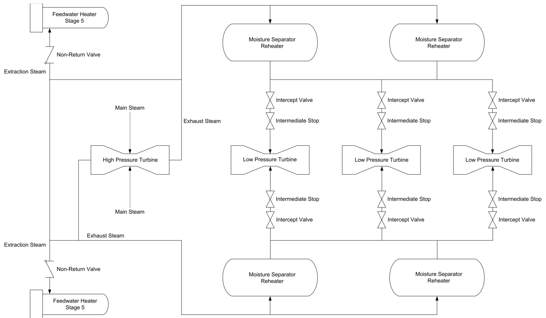
Figure 2.11.1-2. High Pressure Turbine Exhaust Functional Arrangement
