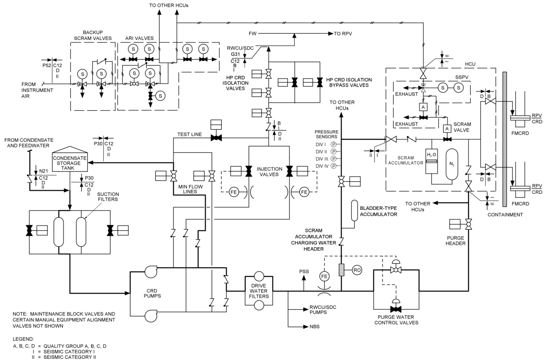
Figure 2.2.2-1. Control Rod Drive System
