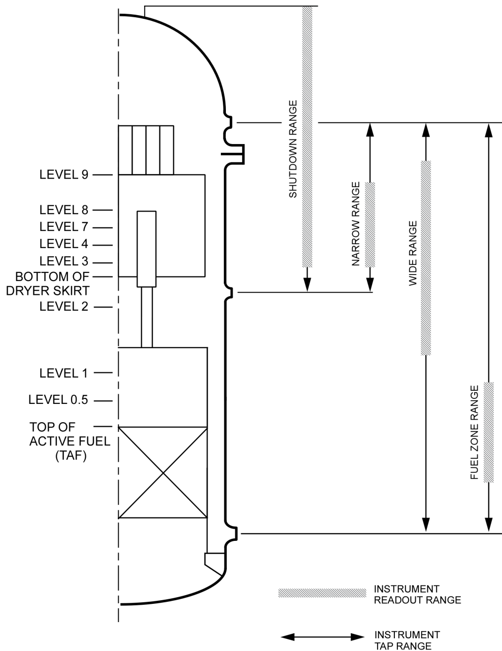
Figure 1.1.1-1 RPV Water Level Range Definition
