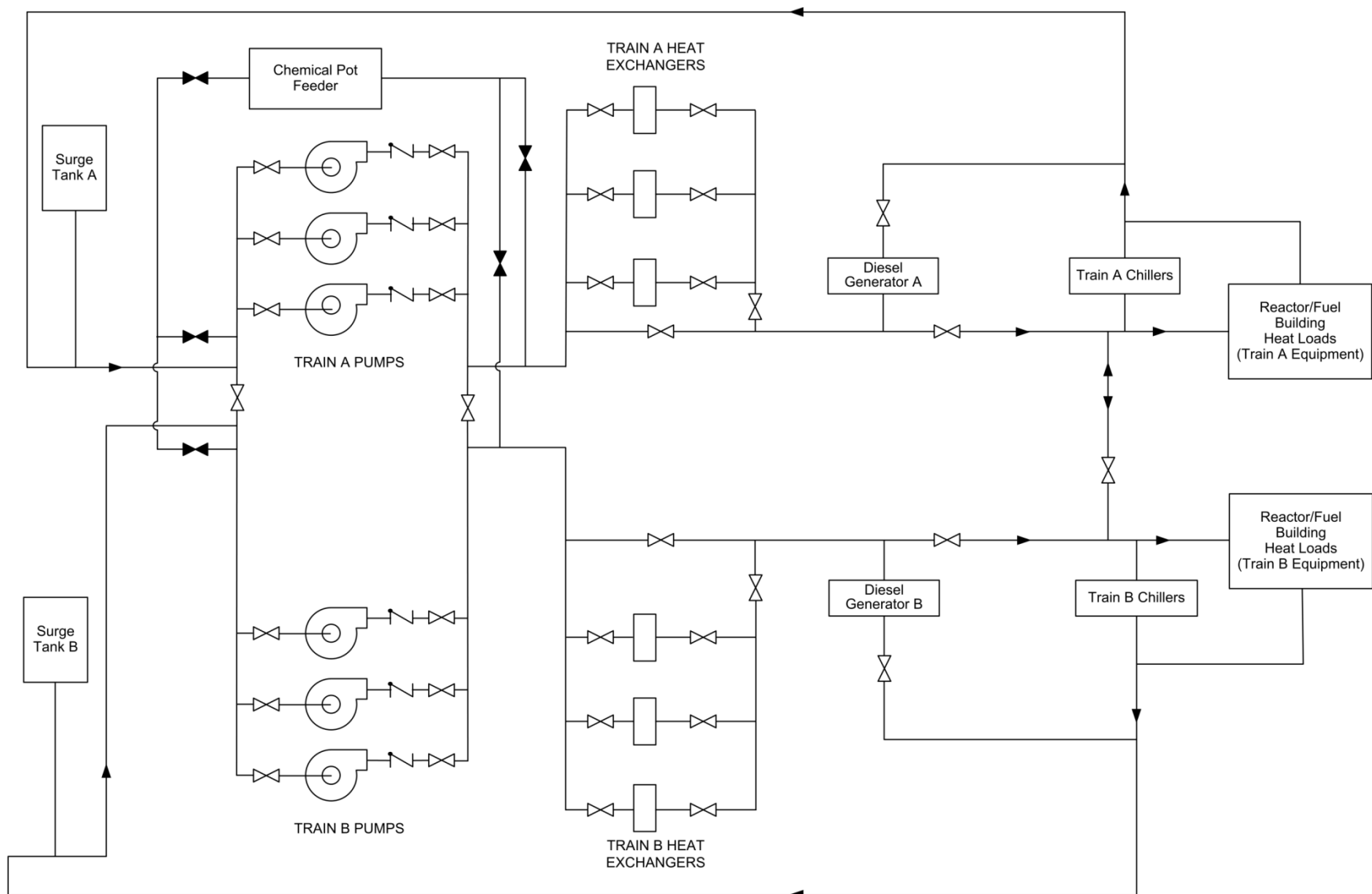
Figure 2.12.3-1. Reactor Component Cooling Water System Functional Arrangement
