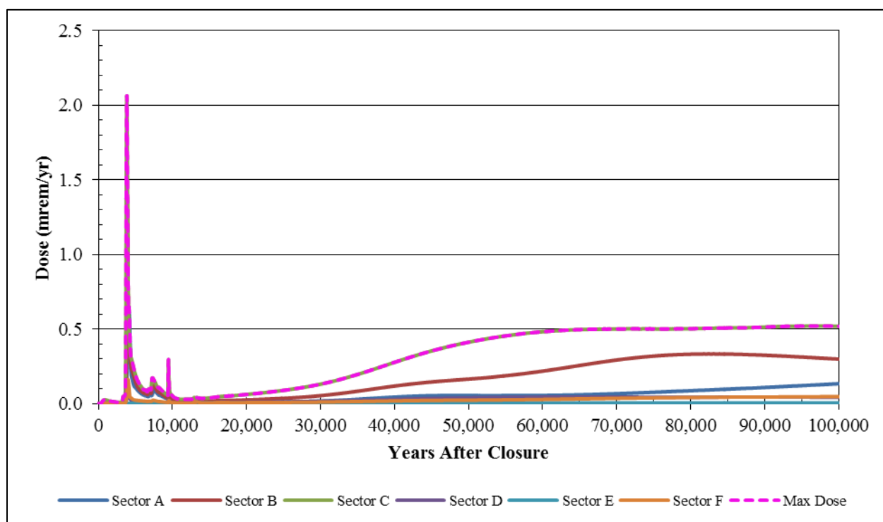
Figure ES-2: 100-Meter MOP Groundwater Pathway Dose within 100,000 Years for Each Sector – with Tank 16 Contribution Only
