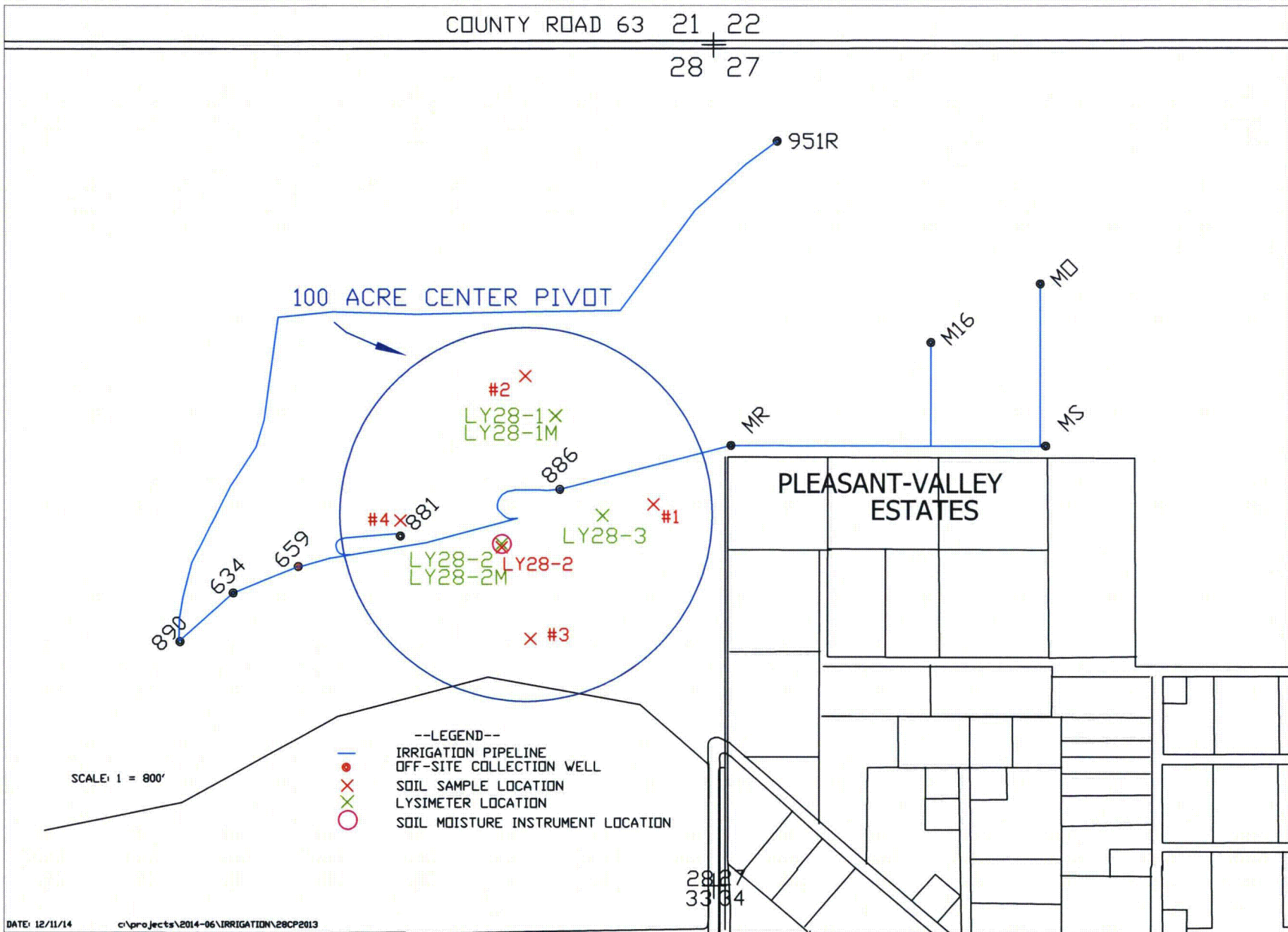
FIGURE A.1-2. SECTION 28 FORMER IRRIGATION AREA WITH SOIL SAMPLE, LYSIMETER, AND SOIL MOISTURE LOCATIONS
