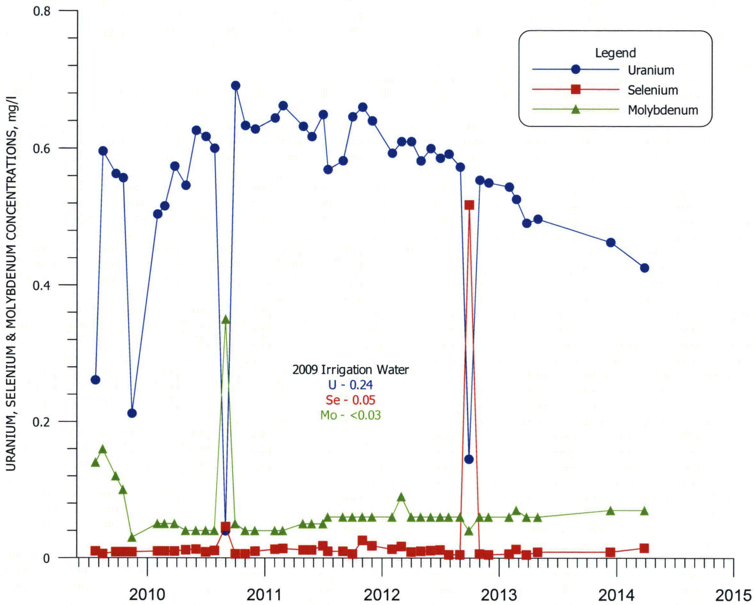
FIGURE A.3-22. URANIUM, SELENIUM AND MOLYBDENUM CONCENTRATIONS FROM LY4MU.
