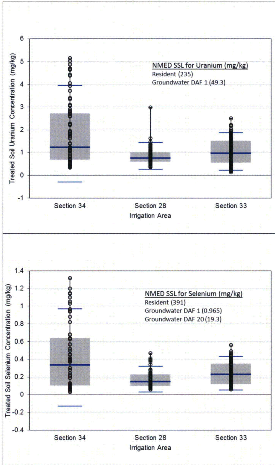
Figure 4-1. Uranium and Selenium Concentrations in Soil with the HMC Irrigation Areas
