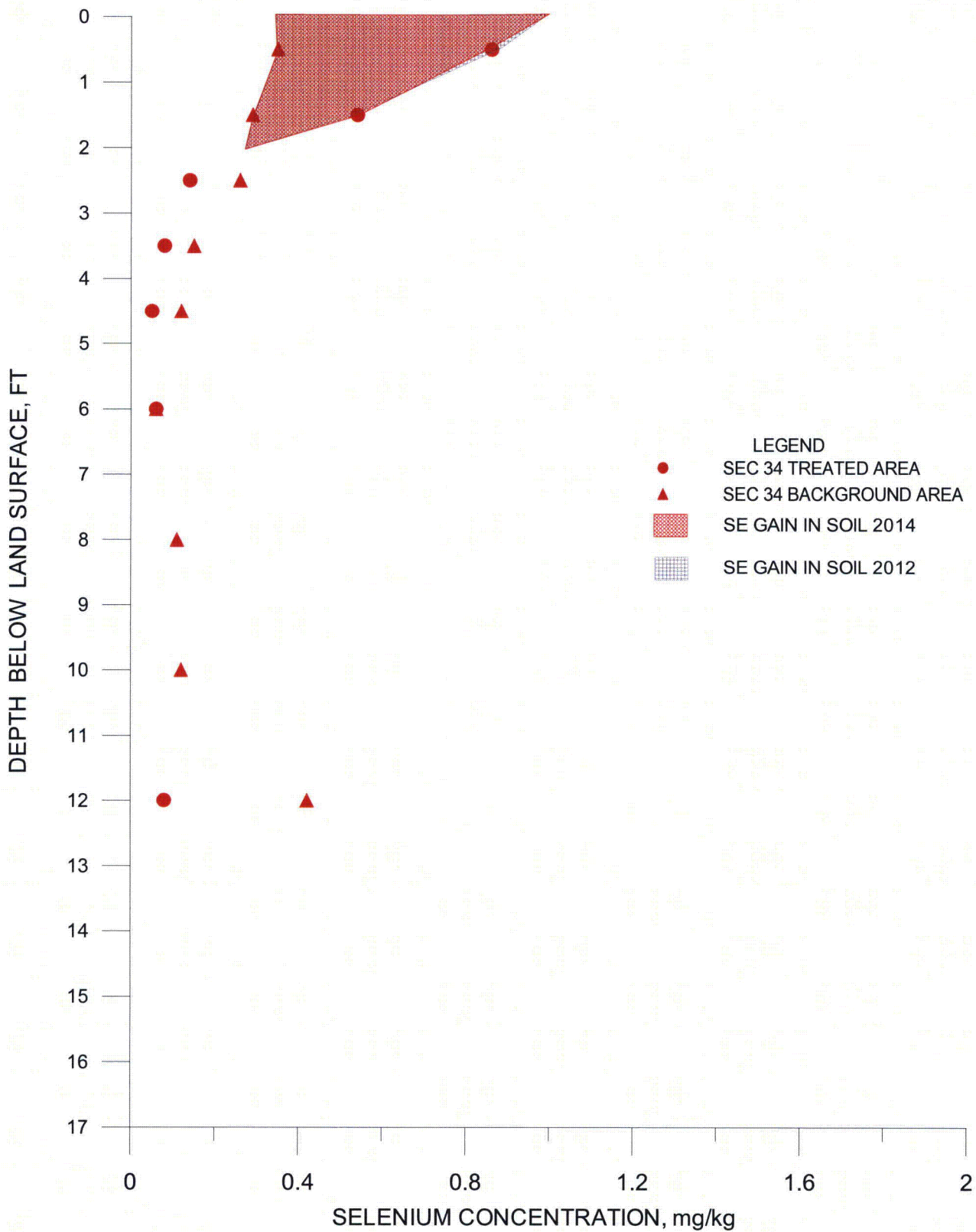
FIGURE A.2-2. SELENIUM CONCENTRATION IN THE SOILS WITH DEPTH IN SECTION 34 IRRIGATION AREA
