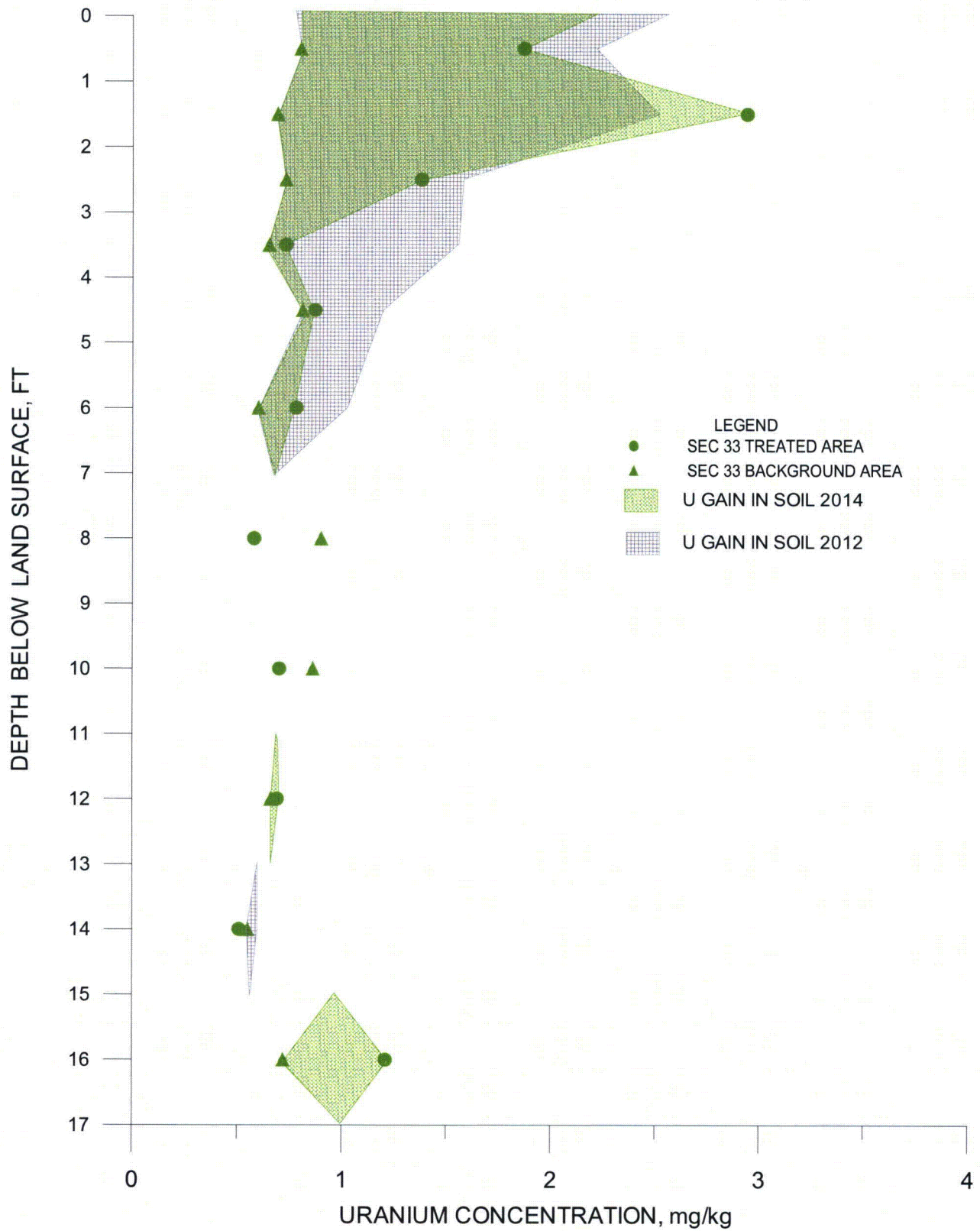
FIGURE A.2-5. URANIUM CONCENTRATION IN THE SOILS WITH DEPTH IN SECTION 33 IRRIGATION AREAS
