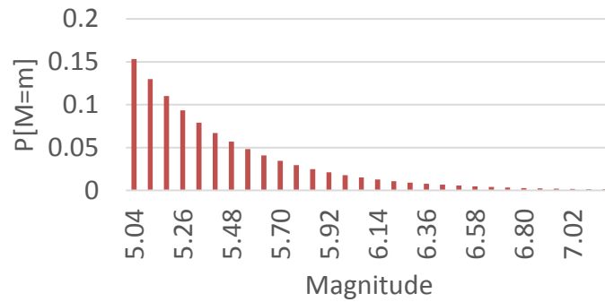
Magnitude PMF
