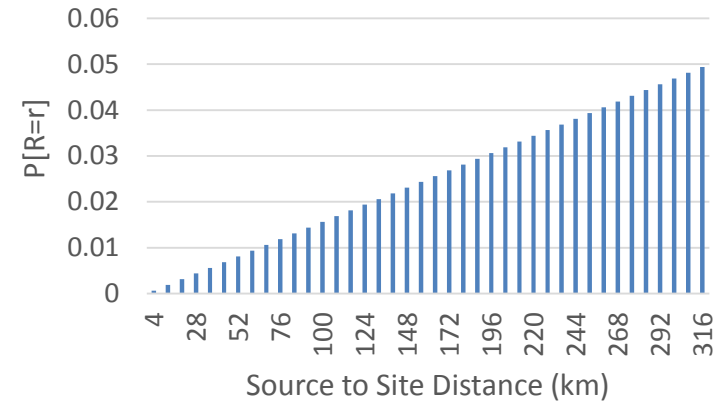
Distance PMF
