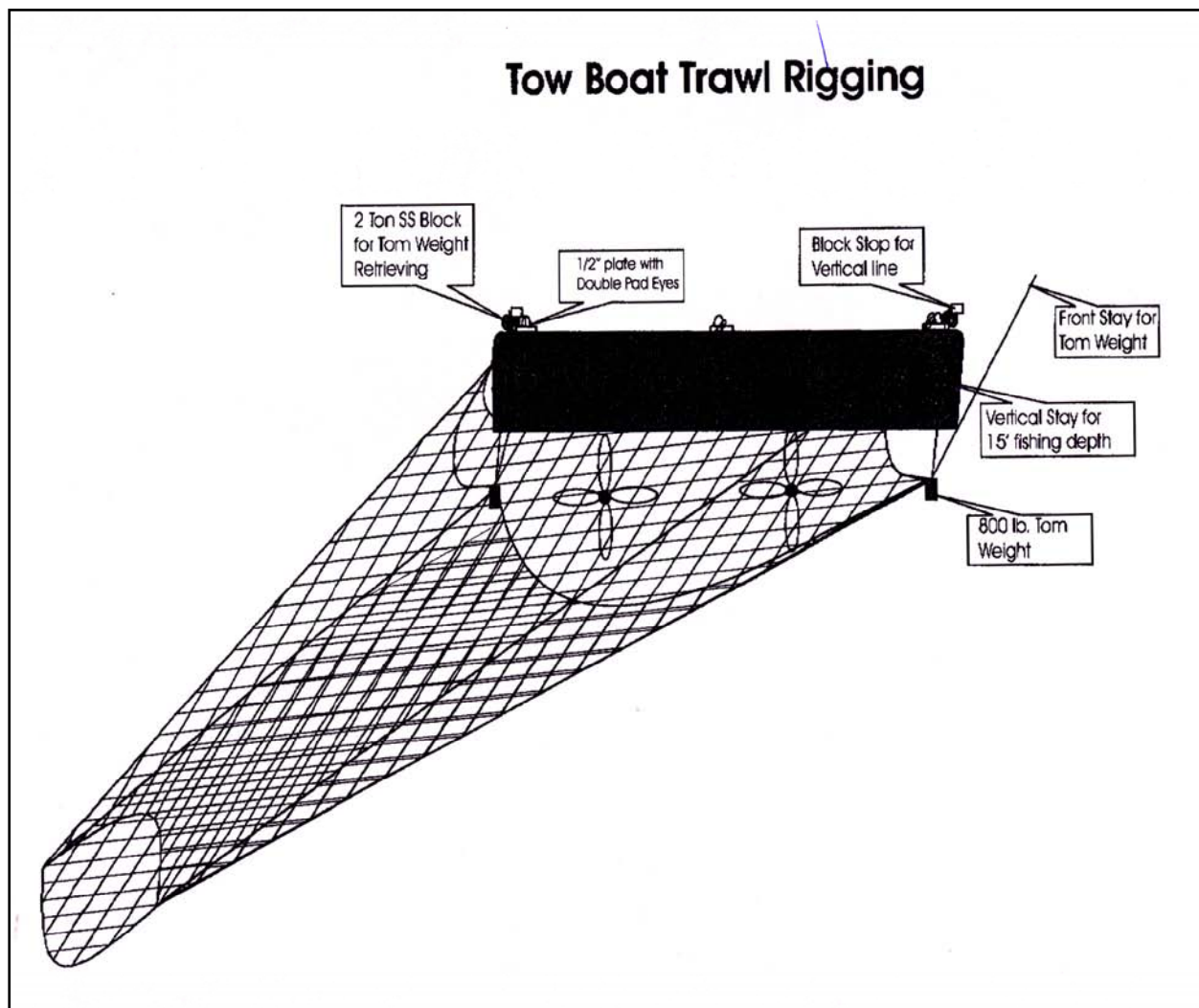
Figure 1. Schematic of the net and trawling gantry deployed from the towboat to filter propwash and entrained fish
