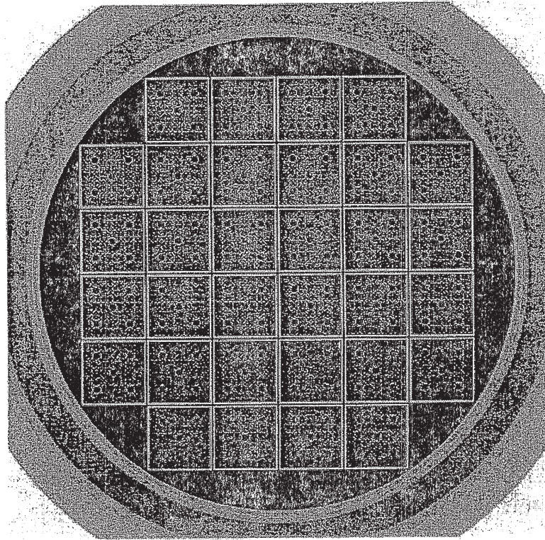
NUHOMS-32P DSC and Transfer Cask KENO V.a Criticality Model
