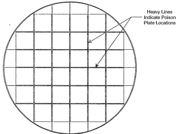
Poison Plate Locations in DSC and Transfer Cask KENO V.a Criticality Model
