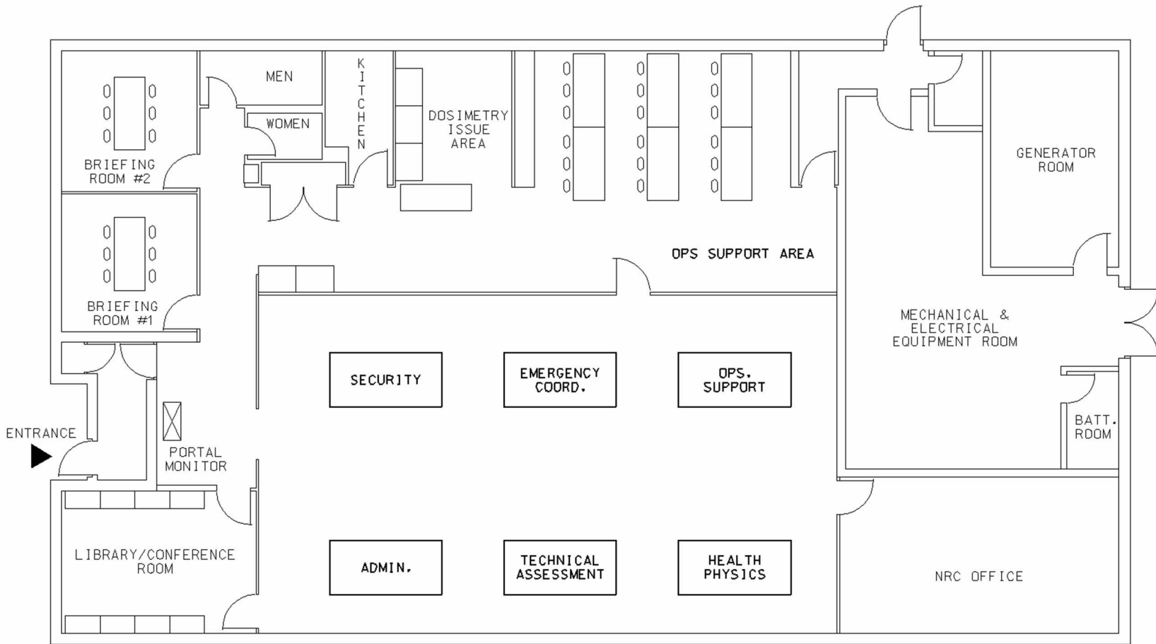
TECHNICAL SUPPORT CENTER (TYPICAL TSC LAYOUT)
