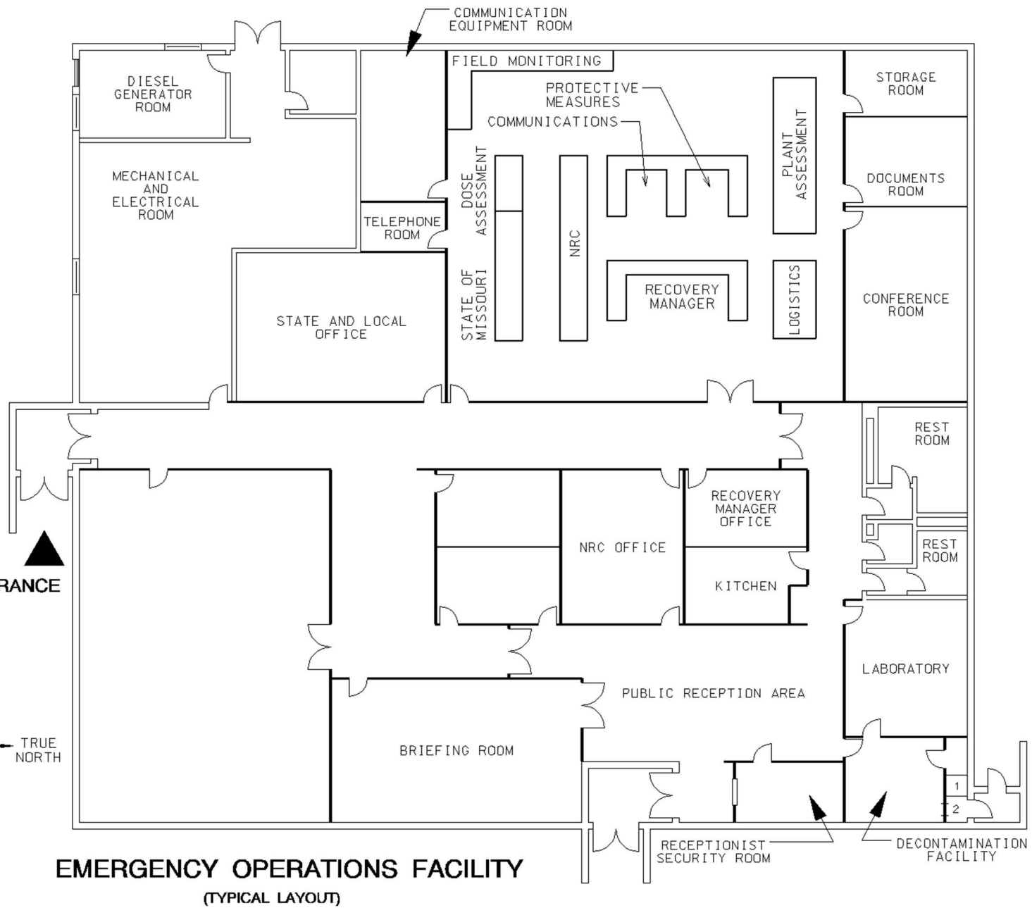
Figure 7-2 Emergency Operations Facility Sheet 1 of 1
