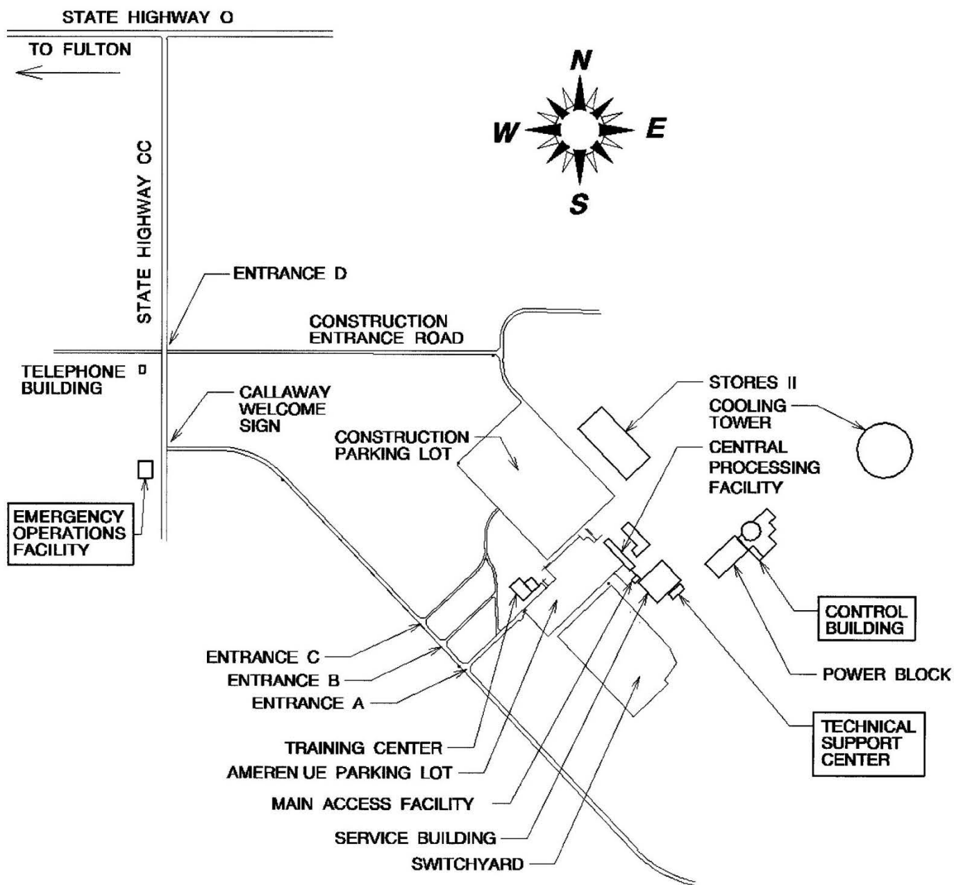
CALLAWAY PLANT FIGURE 7-3 EMERGENCY RESPONSE FACILITY LOCATIONS
