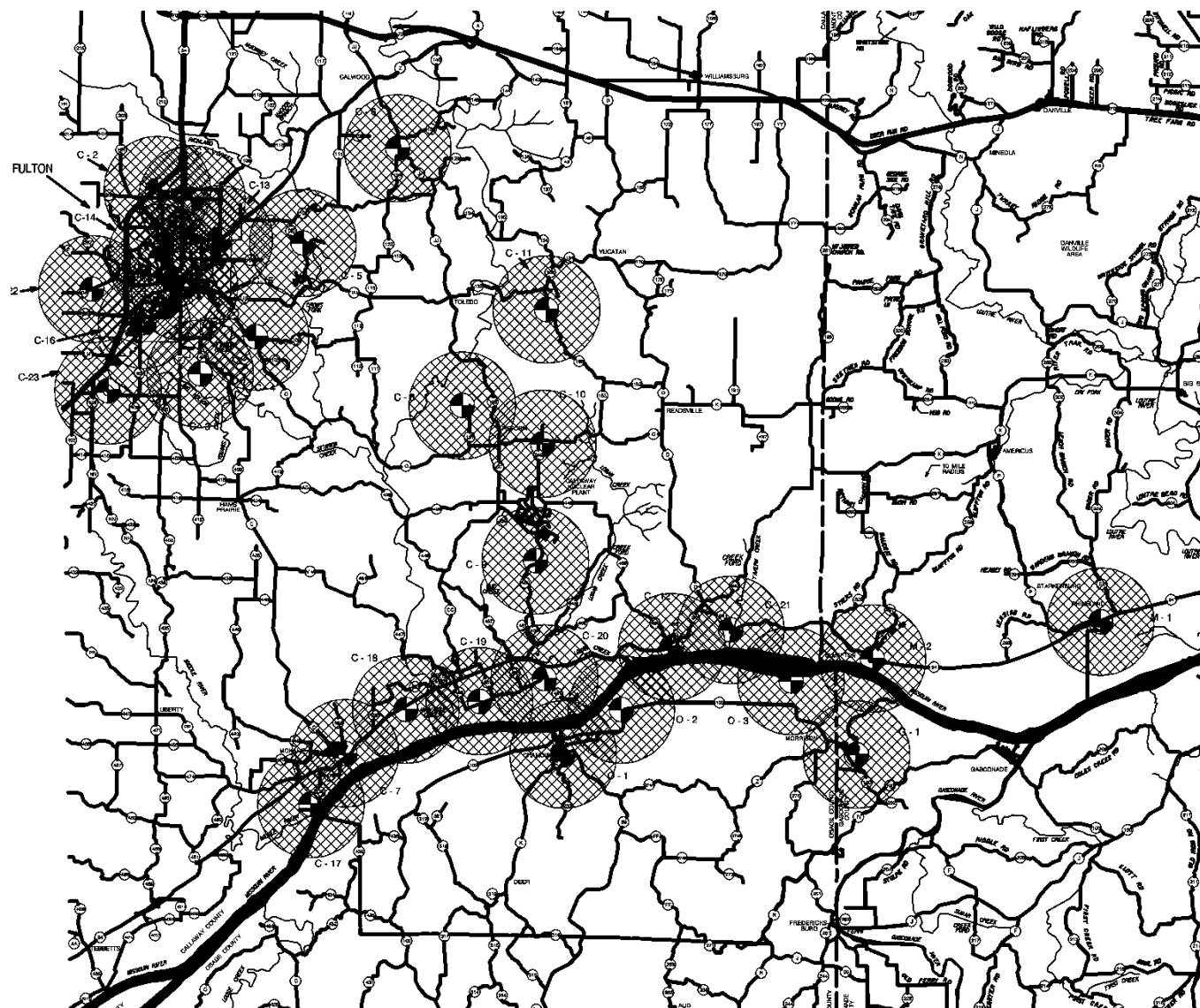
Figure H-1 Public Alert System Siren Coverage
